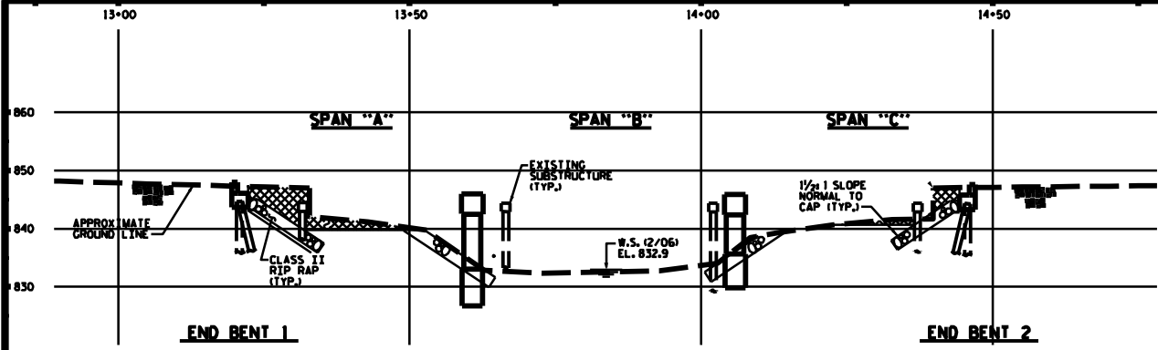
SECTION ALONG -L- SECTION @ END BENTS & BENTS ARE @ RIGHT ANGLES.
