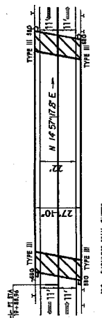
SKETCH SHOWING BRIDGE / PAVEMENT RELATIONSHIP
