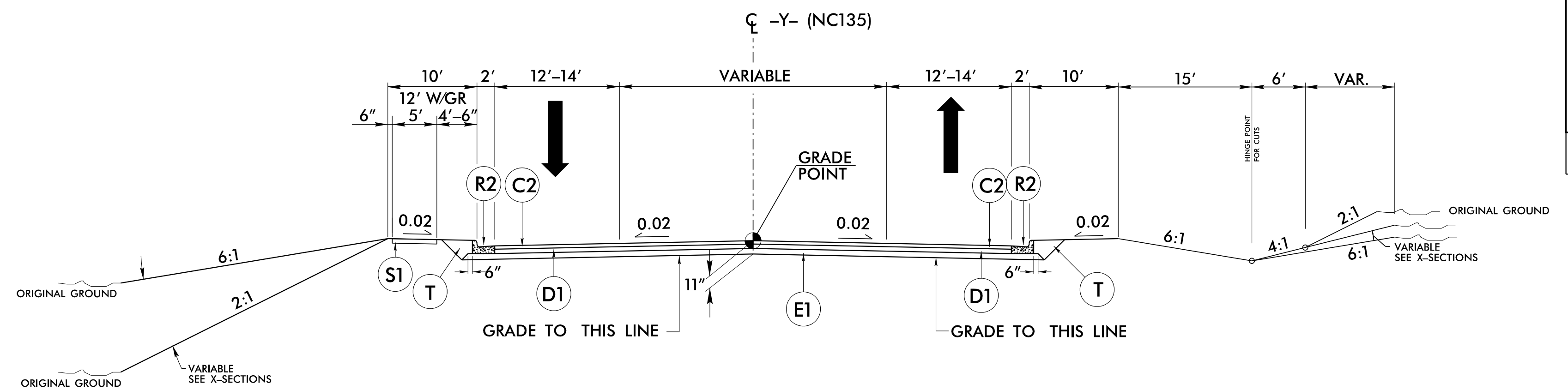
TYPICAL SECTION NO. 2 -Y- STA. 115+91.09 TO -Y- STA. 118+79.50 (Begin Bridge) -Y- STA. 120+59.55 (End Bridge) TO -Y- STA. 122+33.05
