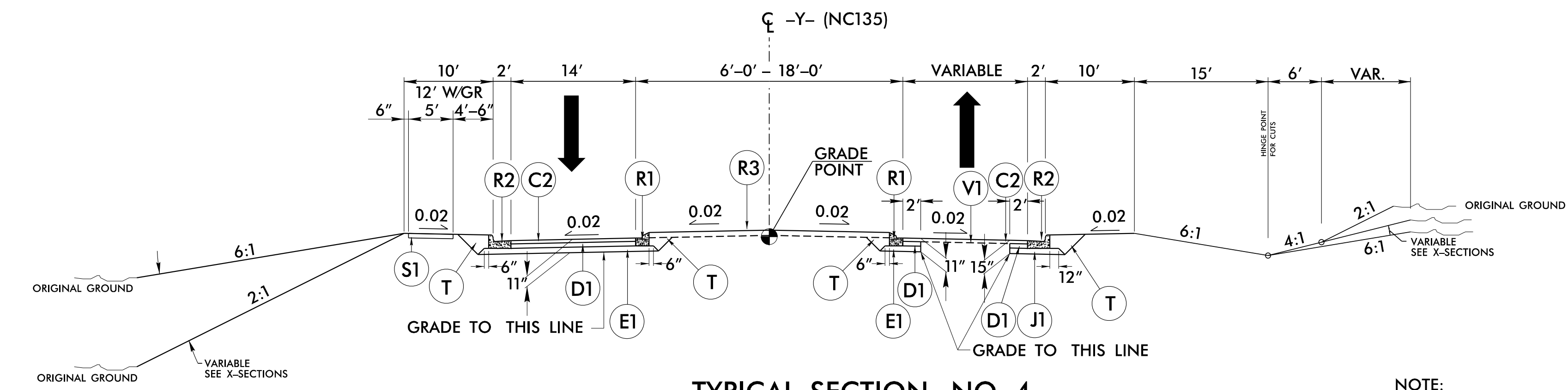
TYPICAL SECTION NO. 4 -Y- STA. 124+50.00 TO -Y- STA. 130+18.89
