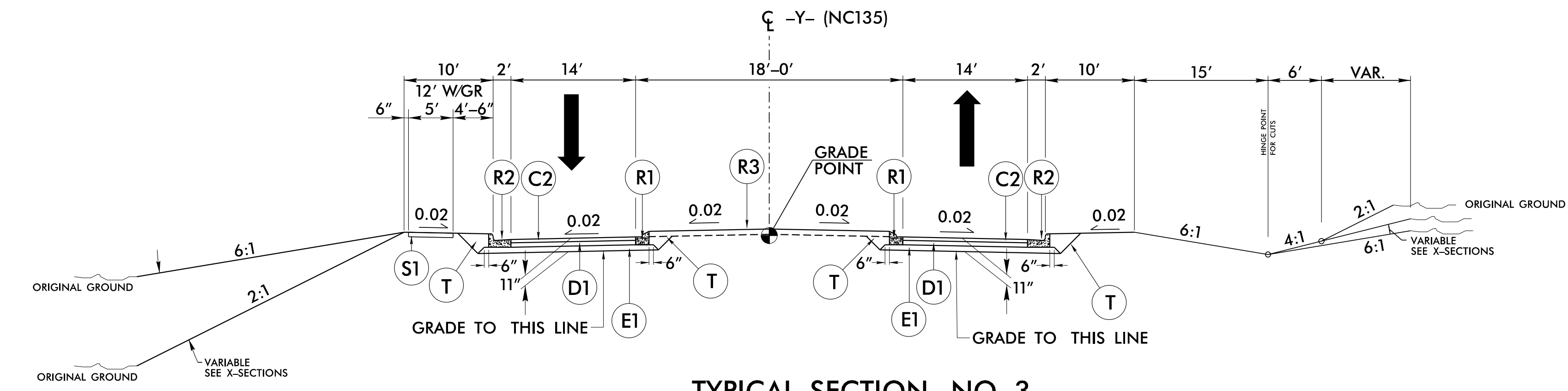
TYPICAL SECTION NO. 3 -Y- STA. 111+02.20 TO -Y- STA. 115+91.09 -Y- STA. 122+33.05 TO -Y- STA. 124+50.00
