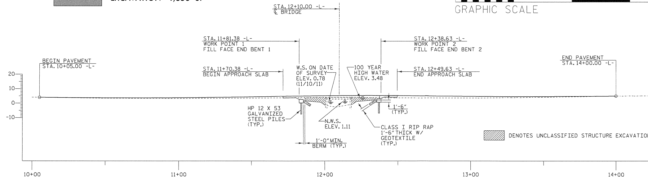
PROFILE ALONG Q SURVEY
