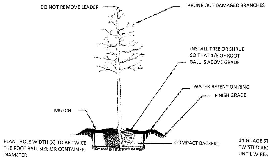
TREE OR SHRUB PLANTING DETAIL (LEVEL GROUND)
