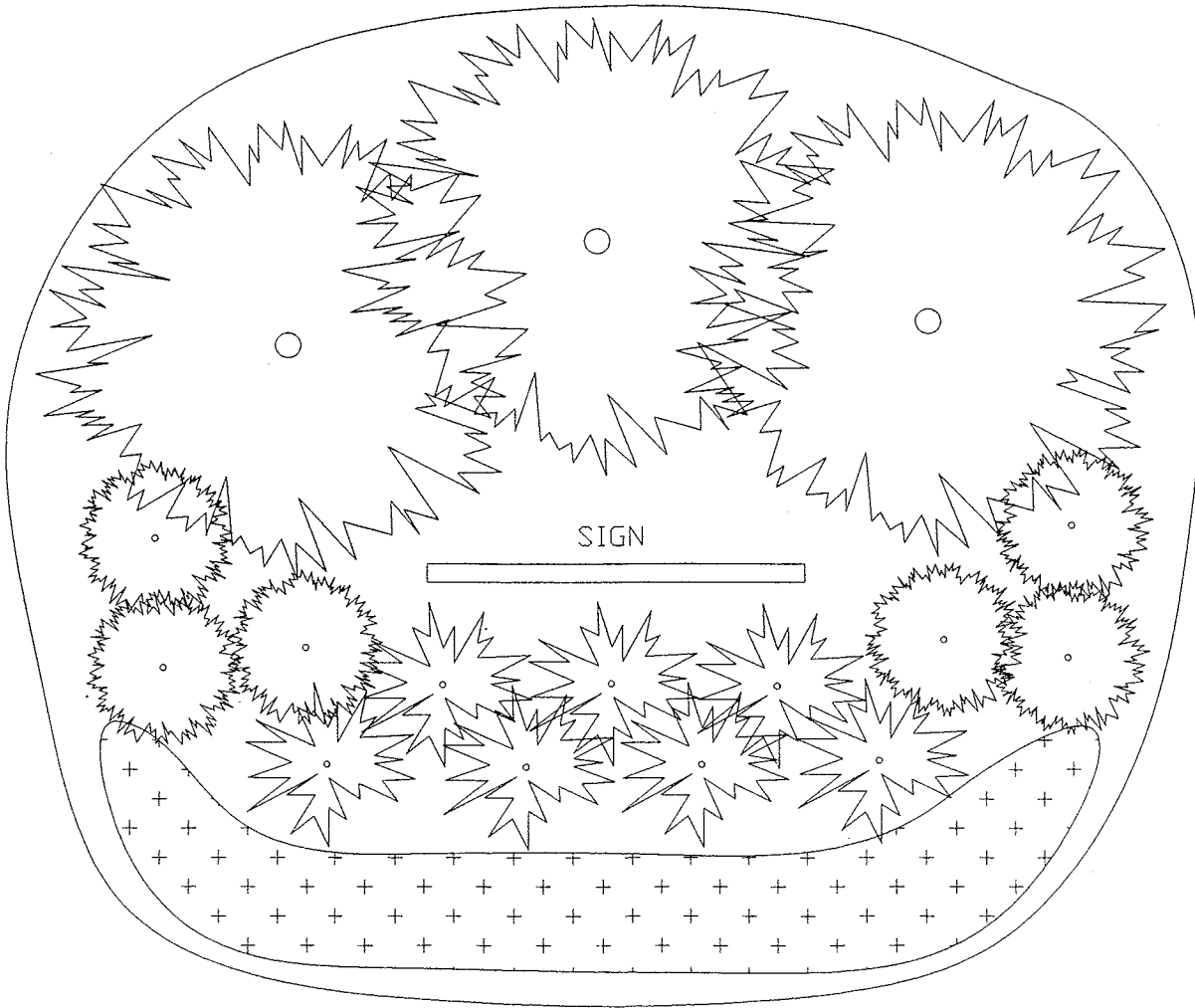
DETAIL A Planting Plan
