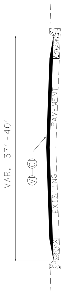
TYPICAL SECTION NO. 3
