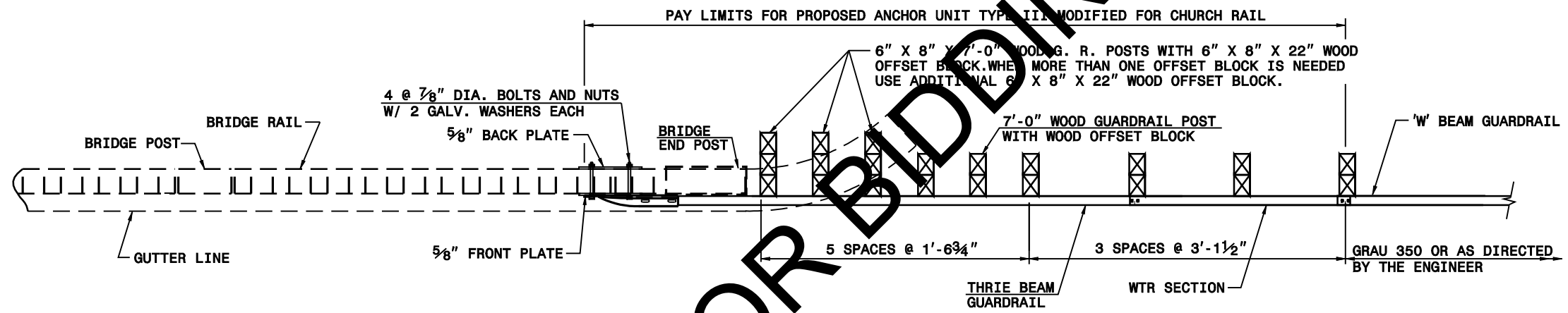
PLAN VIEW
