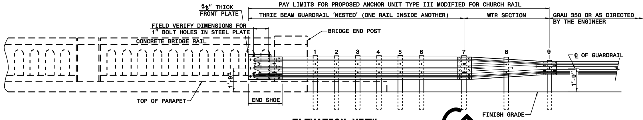
ELEVATION VIEW
