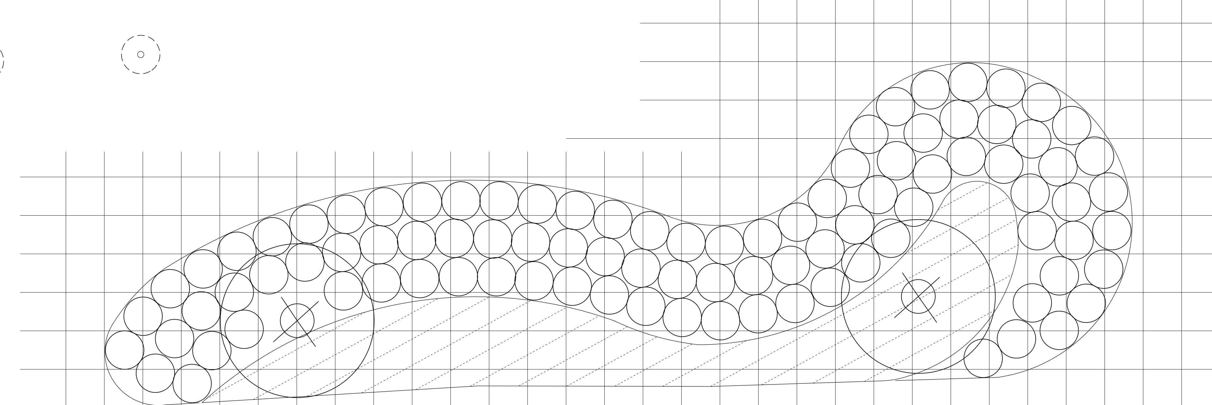
PLANTING DETAIL D
