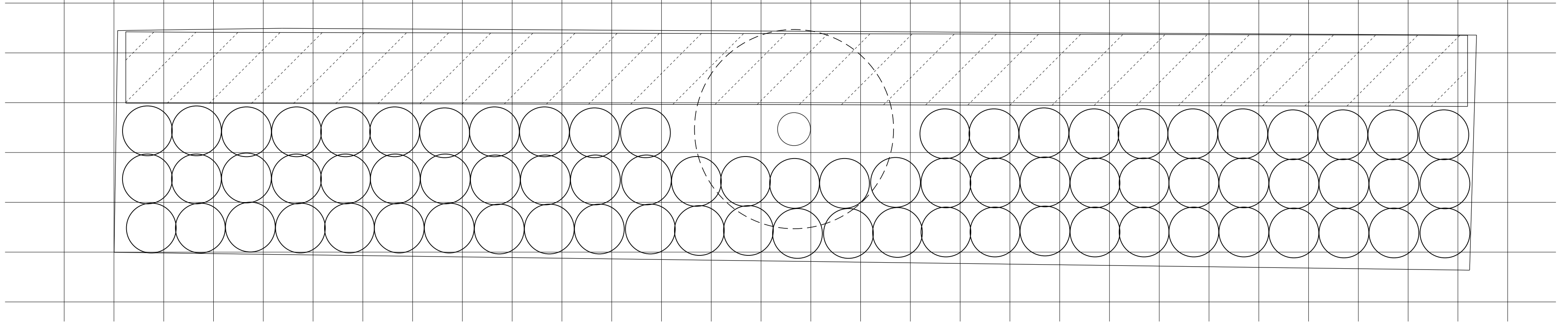
PLANTING DETAIL B GRAPHIC SQUARES 5' O.C.
