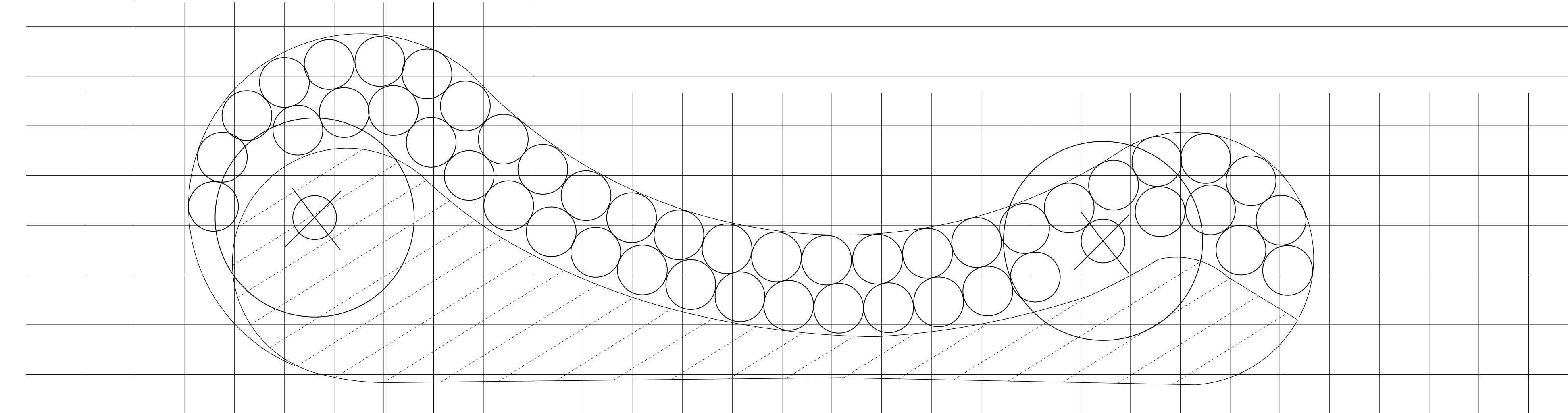
PLANTING DETAIL E
