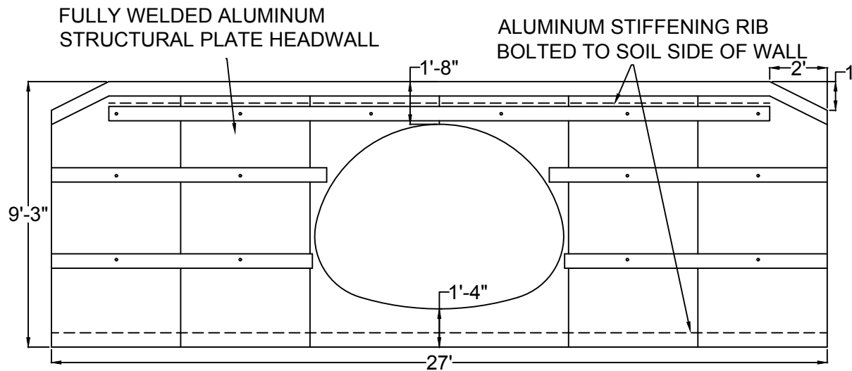
END VIEW- INLET & OUTLET HEADWALL
