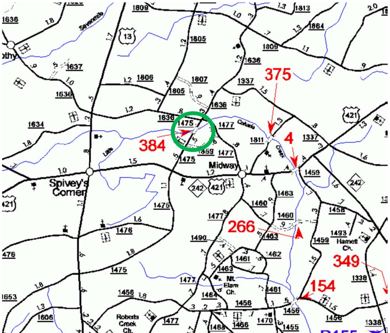
SAMPSON BRIDGE 384 SR 1475 (JB WILSON ROAD) OVER LITTLE COHARIE CREEK 0.8 MILES NORTH OF JCT US 421 78^{\circ} 27' 47.5'' 35^{\circ} 10' 50.5''
