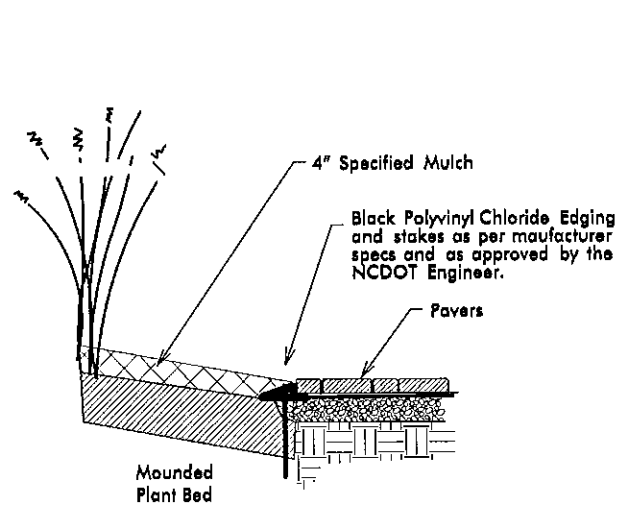
EDGE RESTRAINT FOR PAVERS DETAIL
