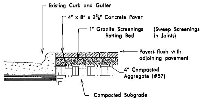
PAVERS ADJACENT TO CURB DETAIL
