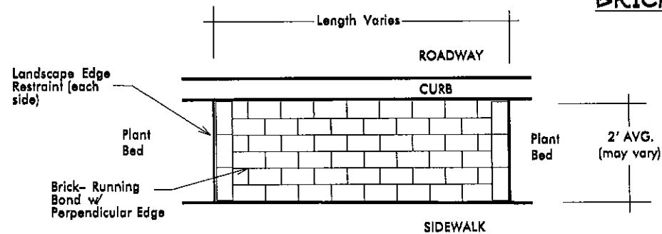
BRICK PAVEMENT DETAIL
