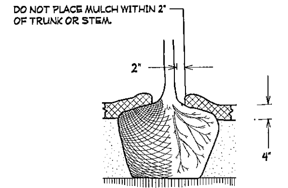
MULCH DETAIL
