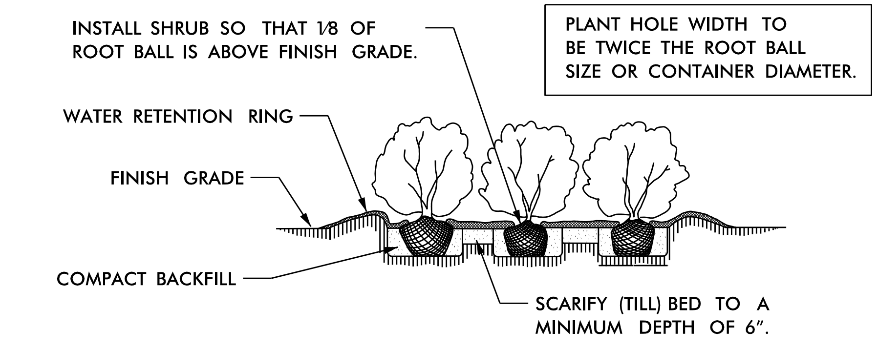
SHRUB BED PLANTING DETAIL
