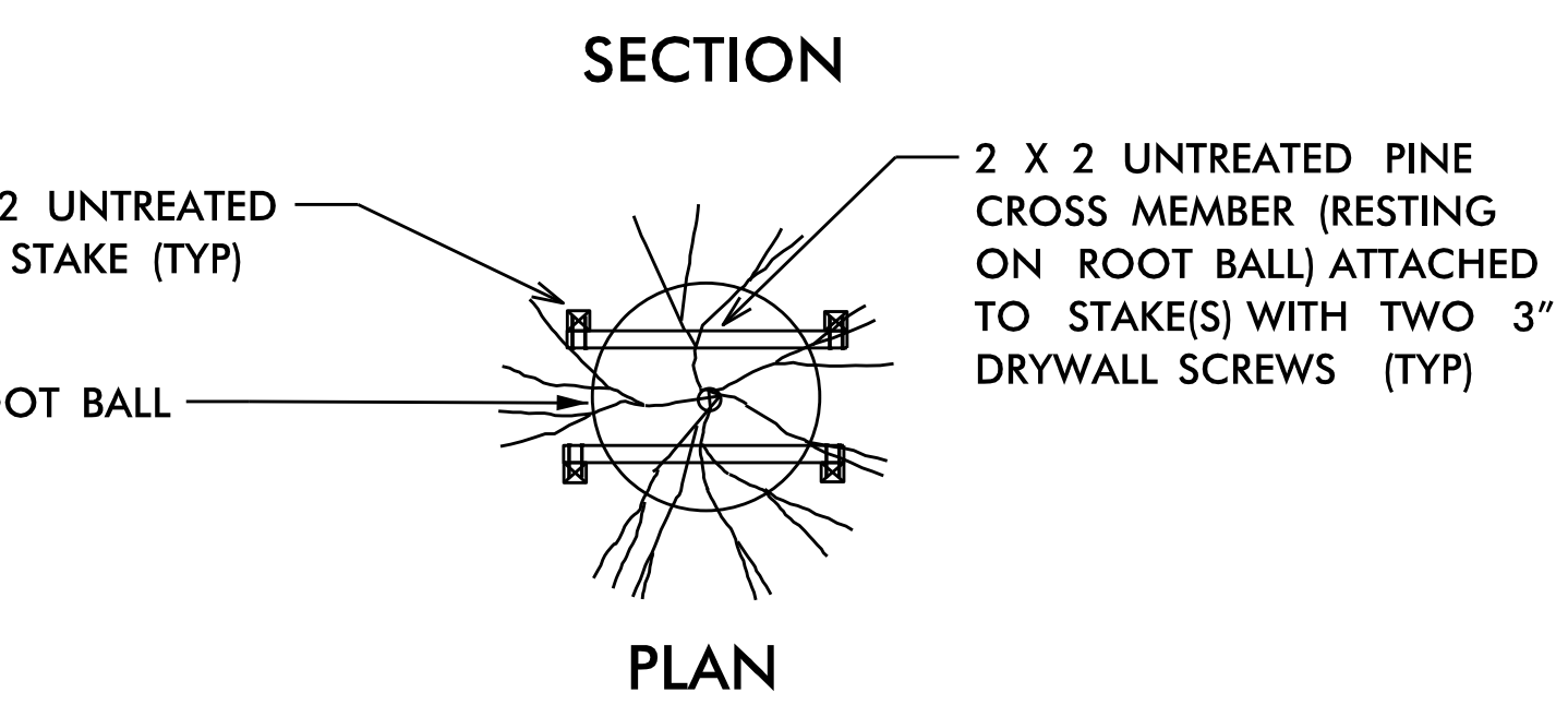
TREE PLANTING & ROOT BALL STAKING DETAIL (STAKE TREES 8' OR TALLER)
