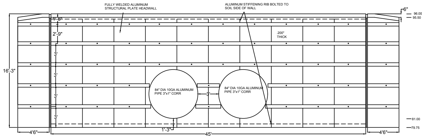
END VIEW- INLET & OUTLET HEADWALL
