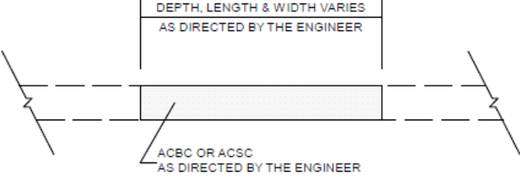
PATCHING EXISTING PAVEMENT
