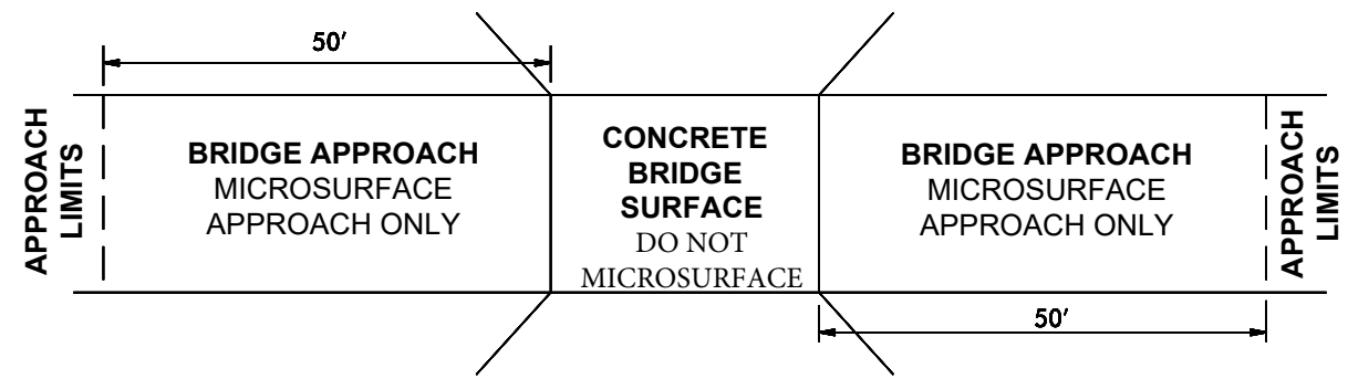
DETAIL FOR MAP # 3 / STRUCTURE # 0245
