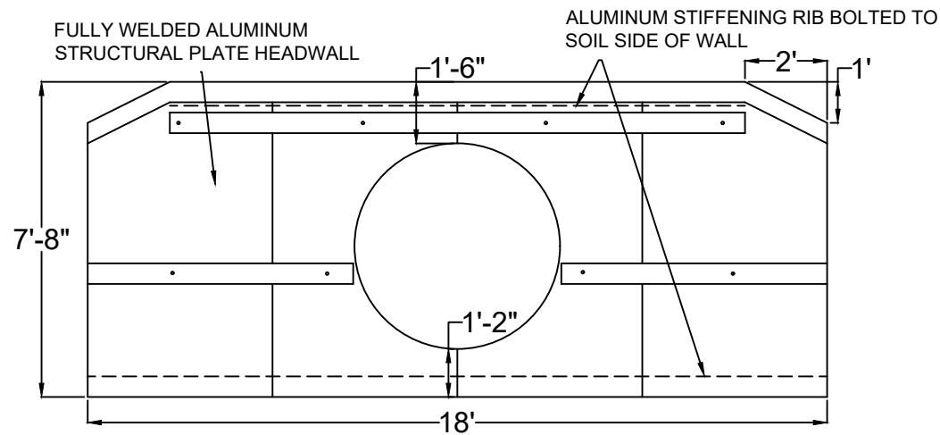
END VIEW- INLET & OUTLET HEADWALL
