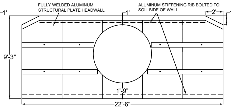
END VIEW- OUTLET HEADWALL
