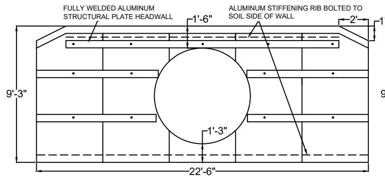
END VIEW- INLET HEADWALL
