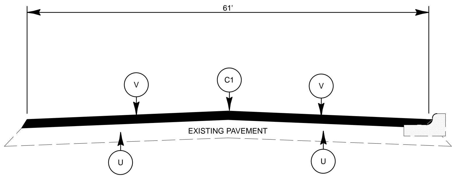
TYPICAL SECTION NO. 2 Typical section to be used for Map 1 from Grace Dr. to Chockoyotte St.
