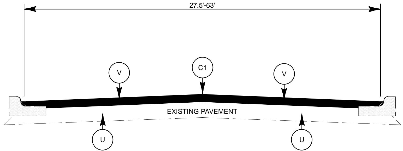
TYPICAL SECTION NO. 1 Typical Section to be used for Map 2, A portion of Map 1 from Country Club Rd. to Grace Dr. and a portion of Map 4 from US 258 to Bryan Ave.
