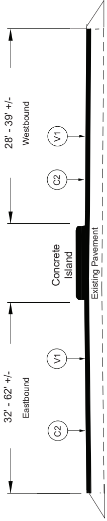
TYPICAL SECTION NO. 1
