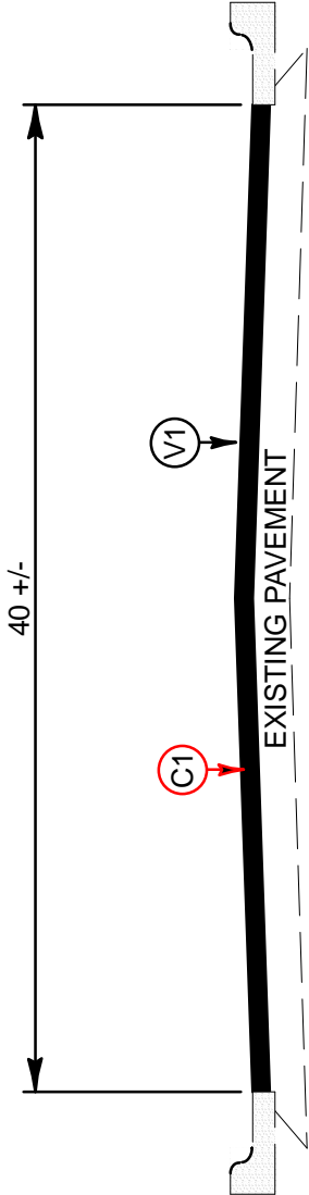
TYPICAL SECTION NO. 3
