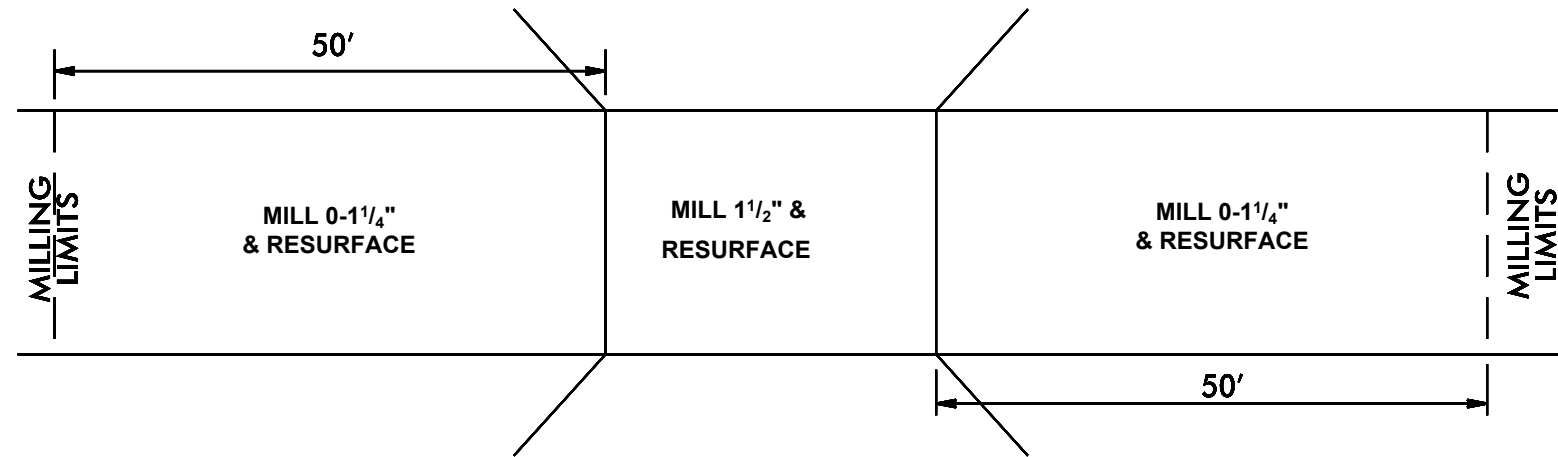
DRAWING FOR BRIDGE #0126 & #0125 & 0011 USE FOR MAP #1
