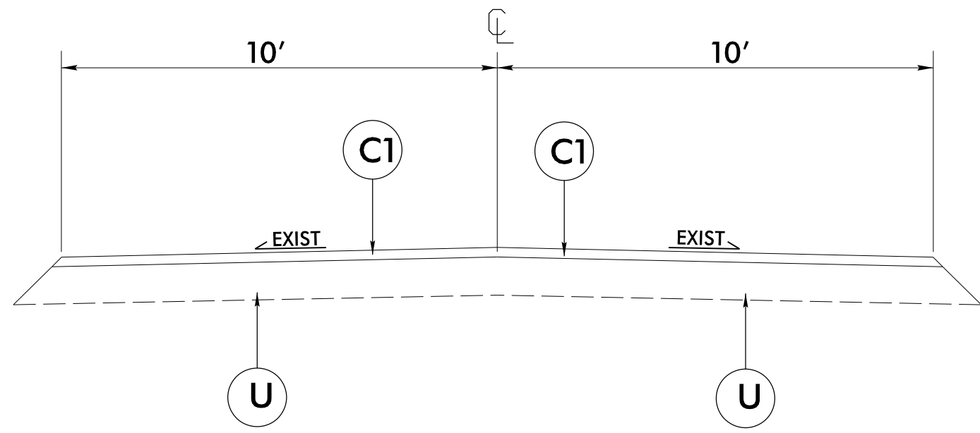
TYPICAL SECTION NO. 1 USE TYPICAL NO. 1 FOR MAPS 1 – 4 & MAP 6
