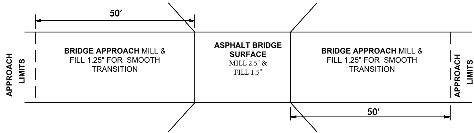
DETAIL FOR MAP # 9 / STRUCTURE # 0225
