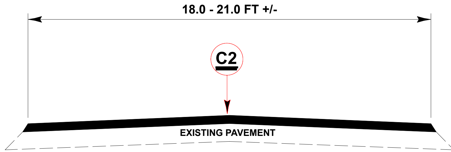
TYPICAL SECTION # 2 MAP(S) # 2, 7-9, 11, 13 - 14
