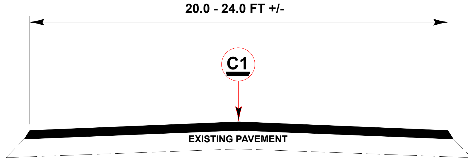
TYPICAL SECTION # 1 MAP(S) # 1, 3, 5 - 6, 10, & 12
