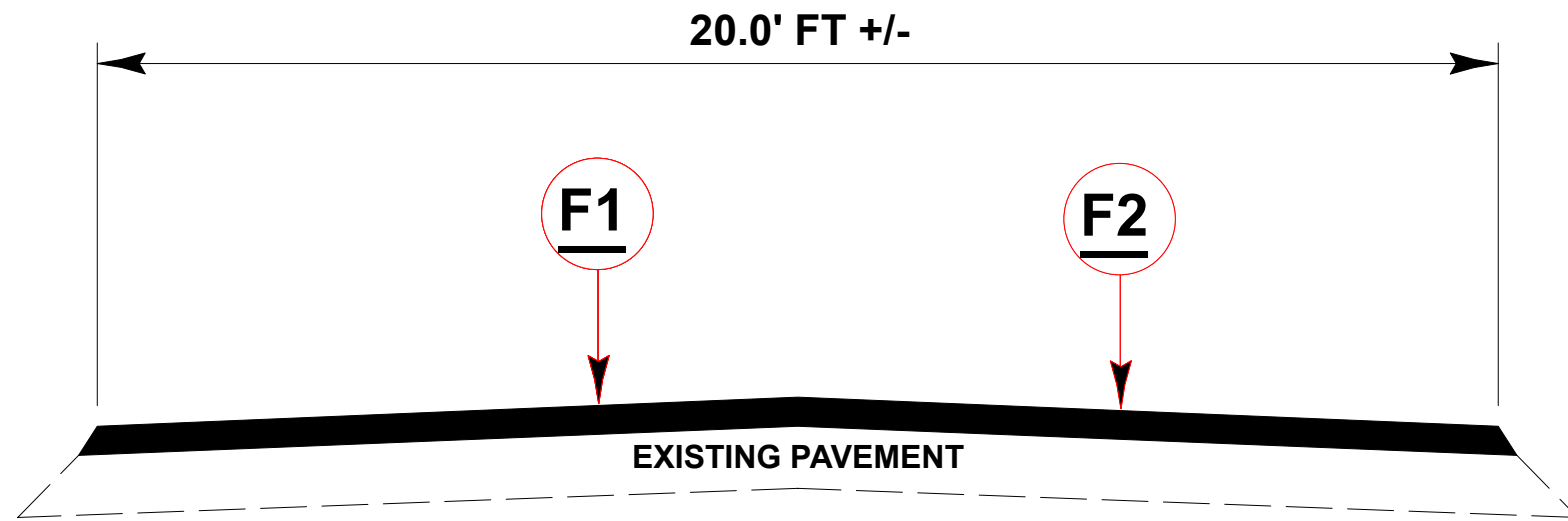
TYPICAL SECTION # 2 MAP(S) # 3 - 7
