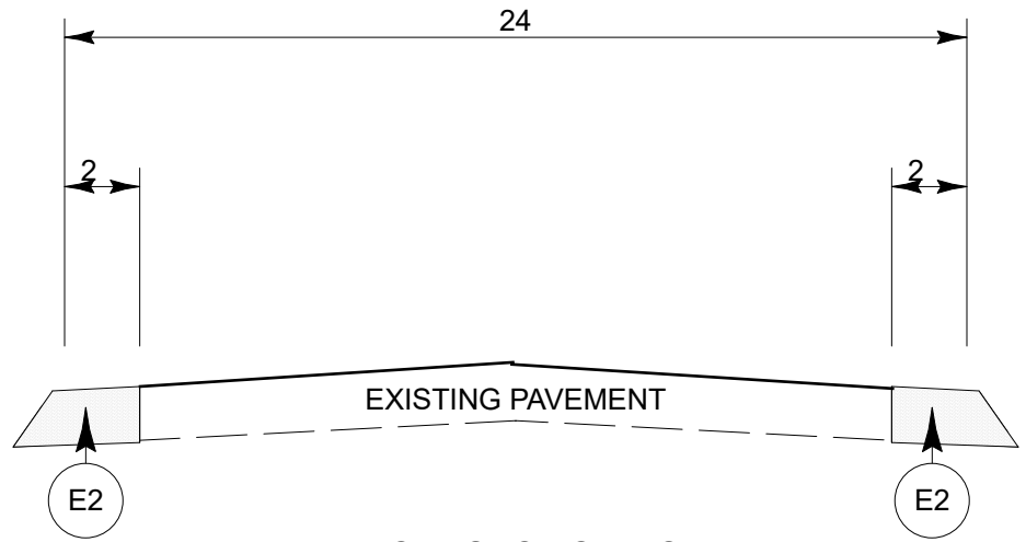
TYPICAL SECTION NO. 6
