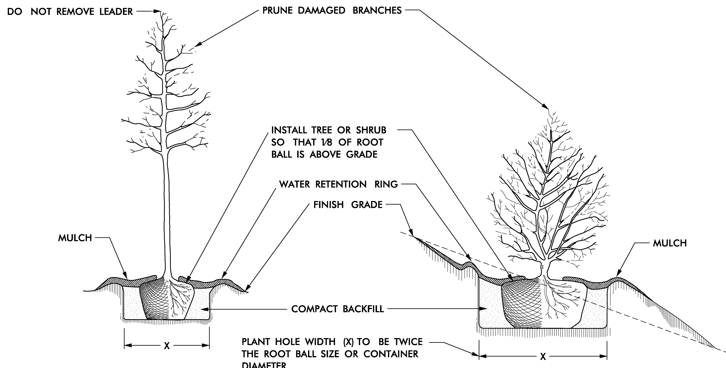
TREE OR SHRUB PLANTING DETAIL (LEVEL GROUND)
