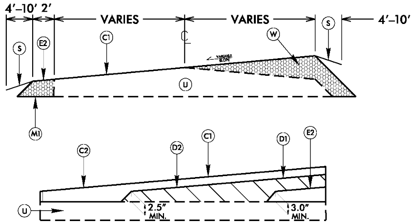
WEDGING DETAIL
