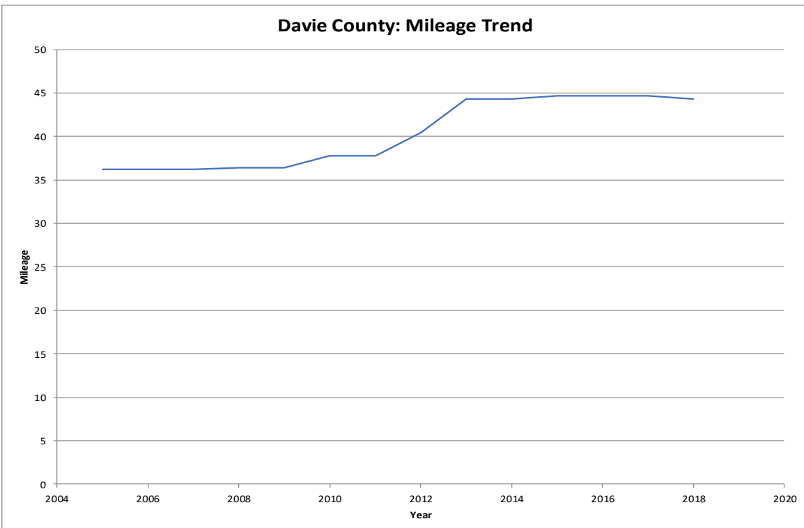
Figure #2: Total non-system mileage for the county of Davie from 2005 to 2018.
