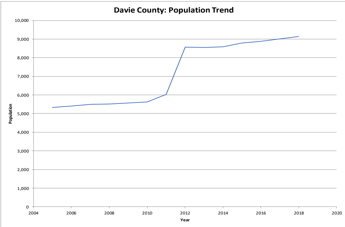
Figure #1: Recorded population in the county of Davie from 2005 to 2018
