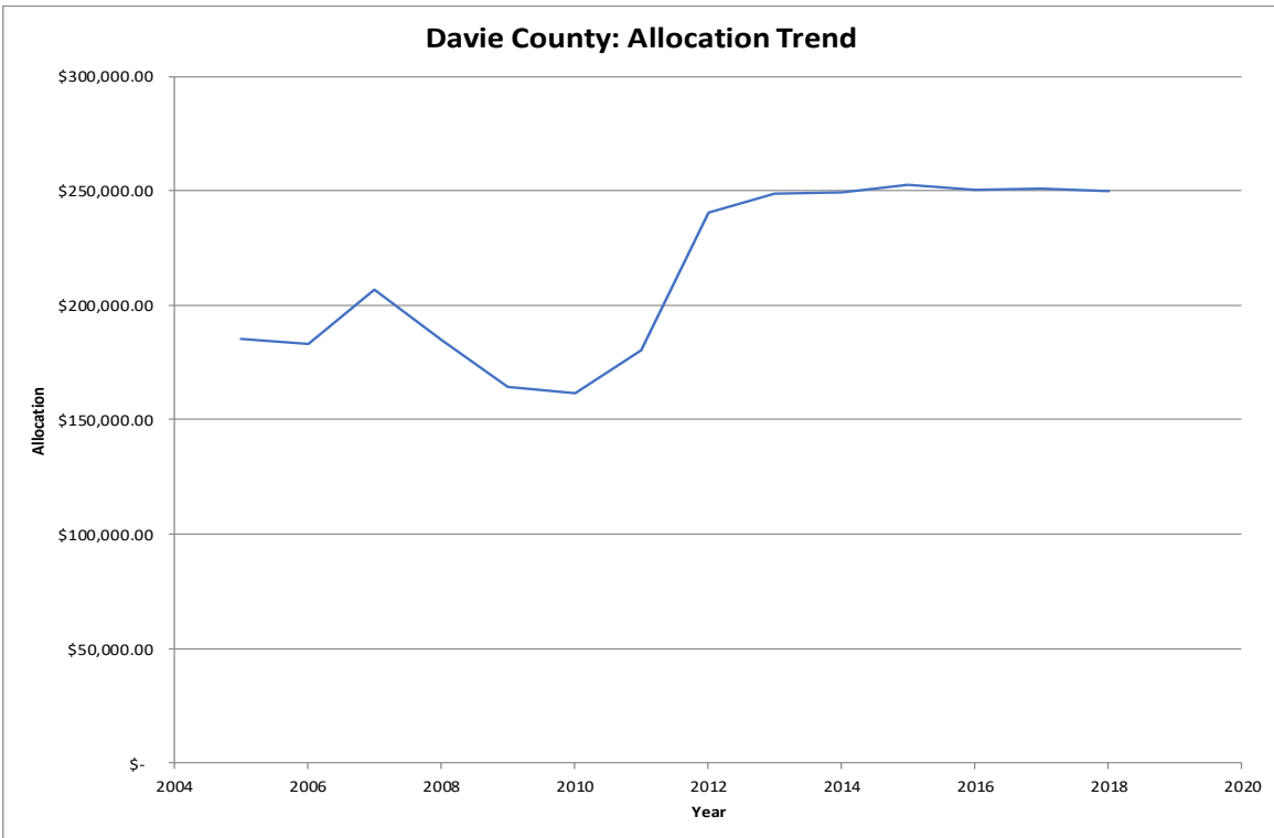
Figure #3: Total allocation given to the county of Davie from 2005 to 2018.
