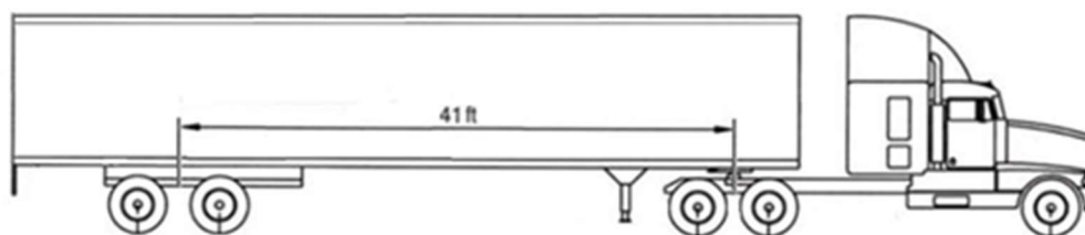
Figure 8-16 Modified WB-62WB-62FL Truck
