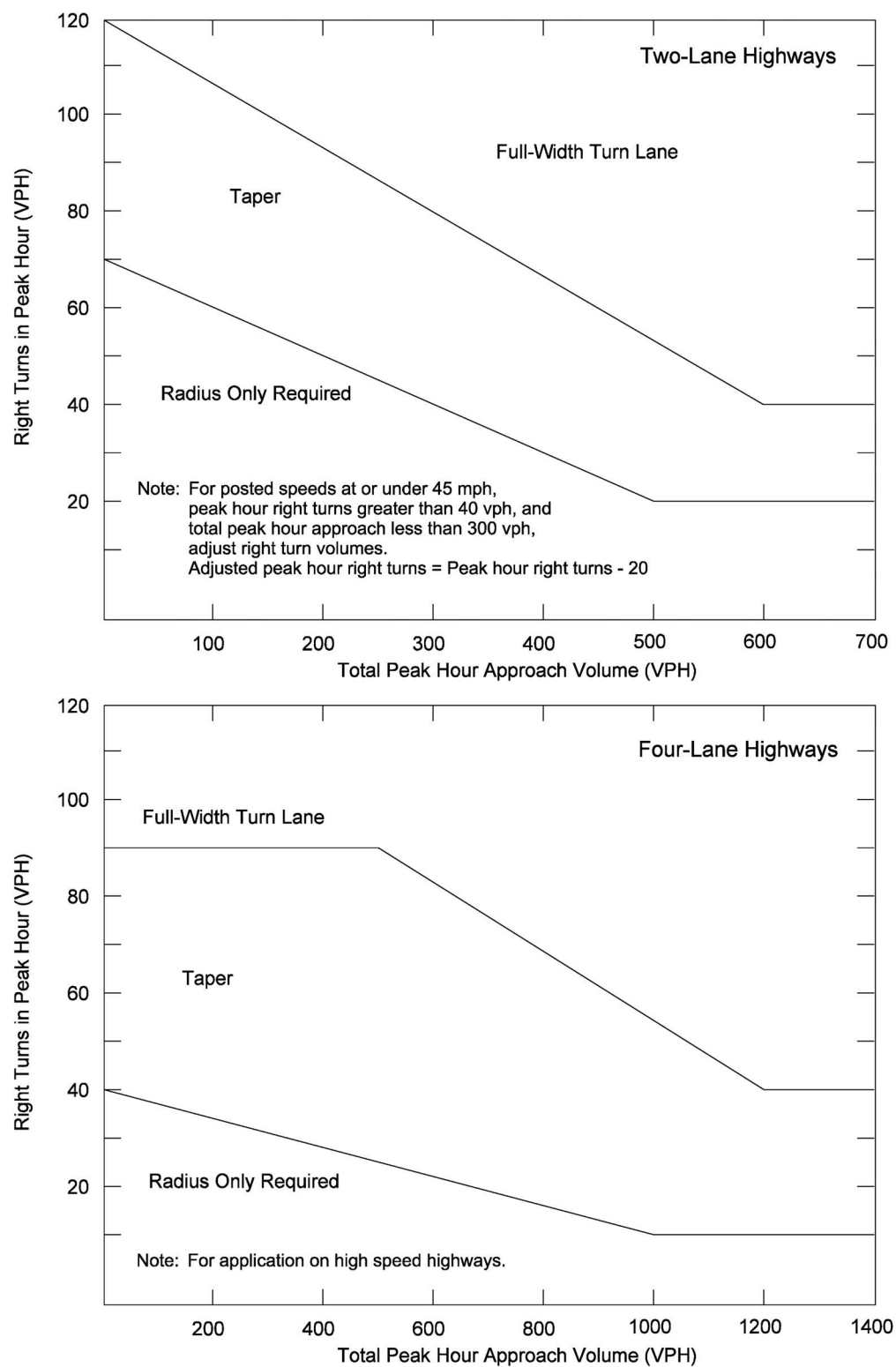
Figure 8-8 Right Turn Lane Warrants
