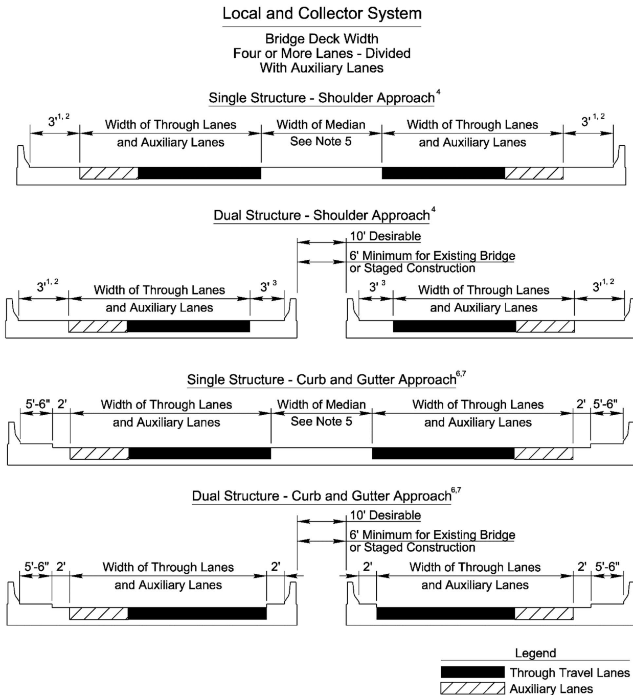
Figure 5-10 Local and Collector System Bridge Deck Widths for Four or More Lanes Divided with Auxiliary Lanes
