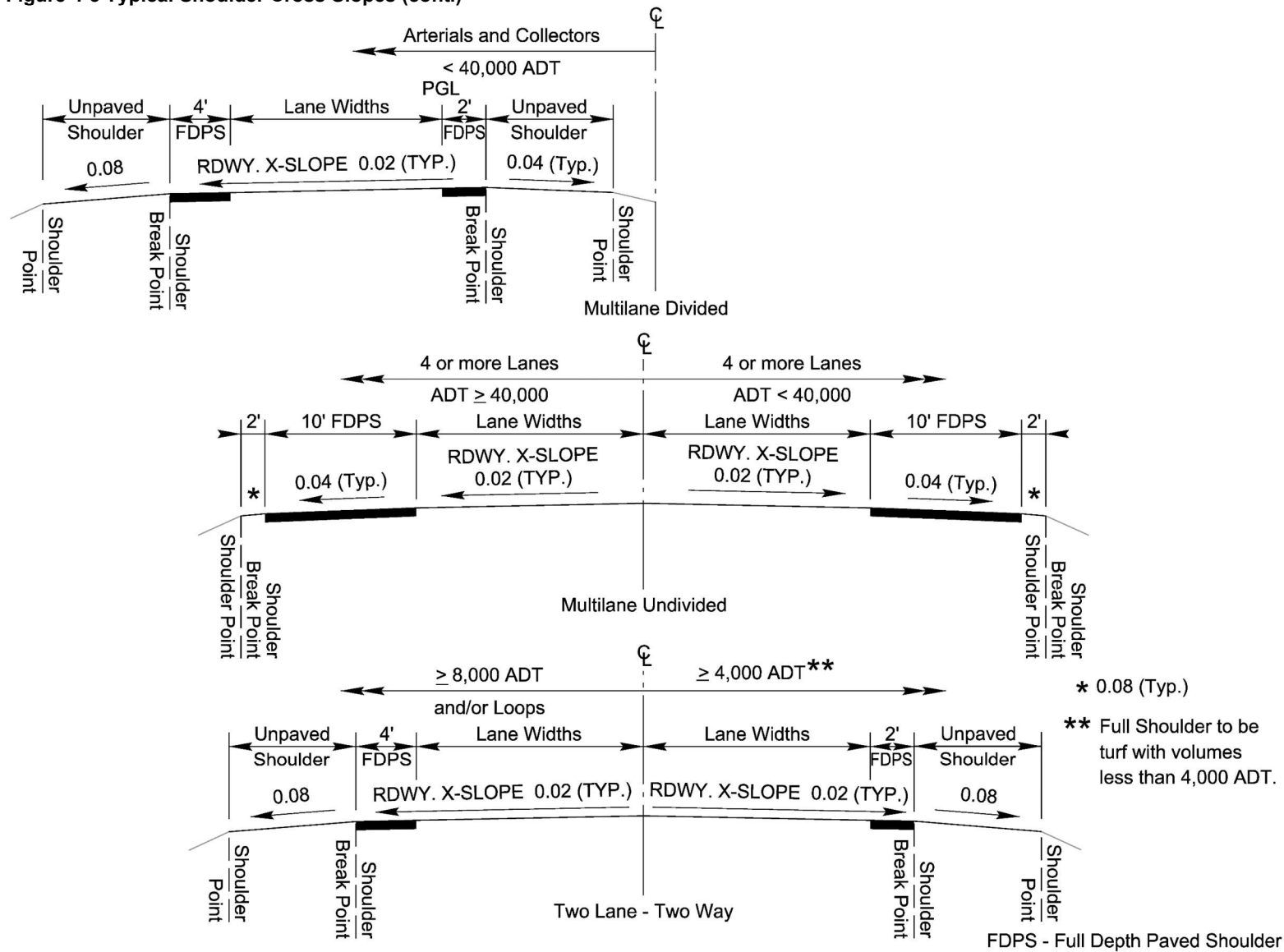
Figure 4-3 Typical Shoulder Cross Slopes (cont.)
