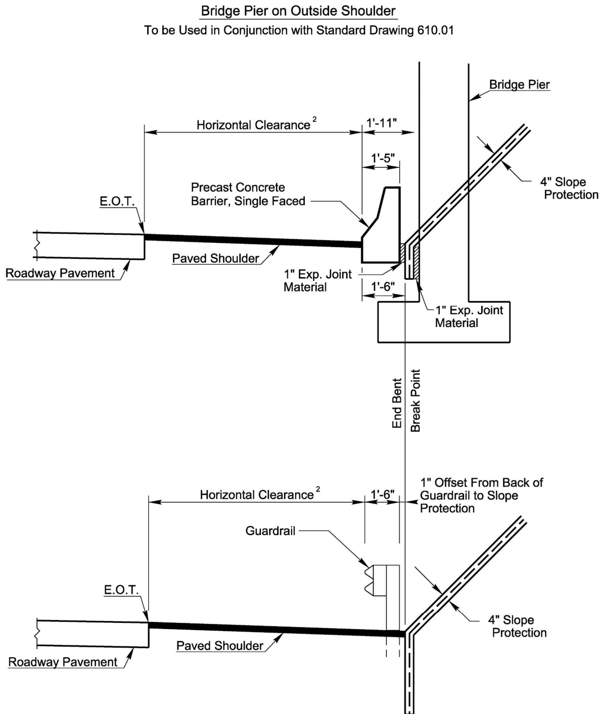
Figure 5-20 Shoulder Detail Under Bridge with Bridge Pier and Concrete Barrier or with End Bent Slope and Guardrail
