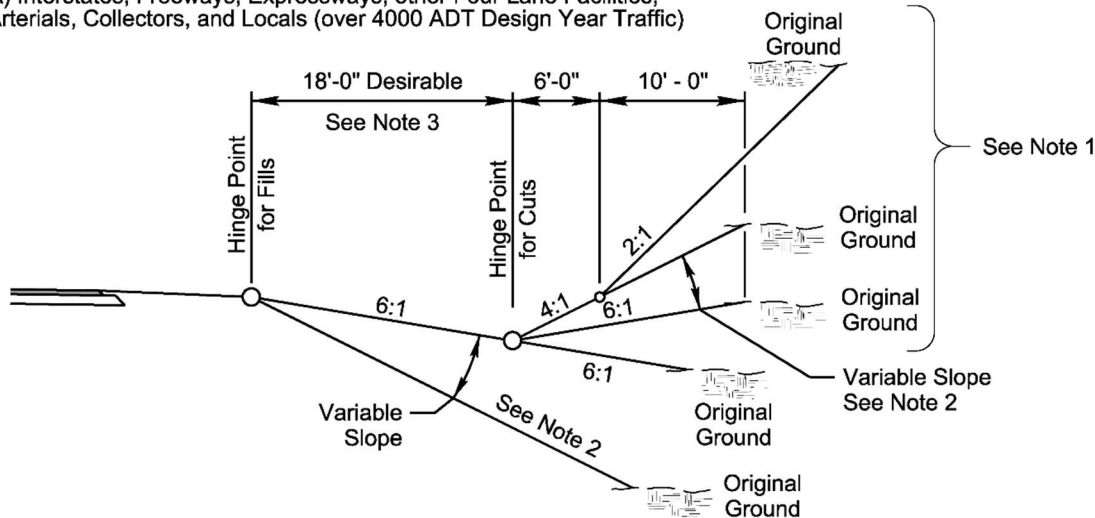
Figure 4-4 Criteria for Roadway Typical Section and Slopes
