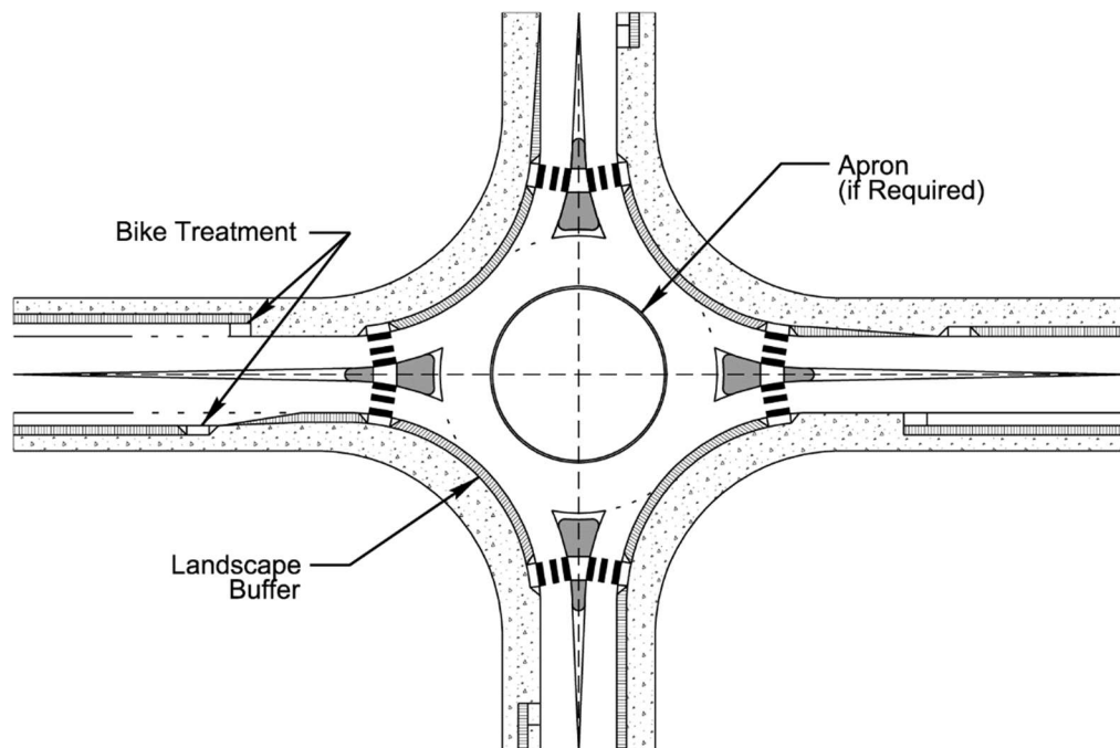
Figure 8-1 Typical Single Lane Roundabout
