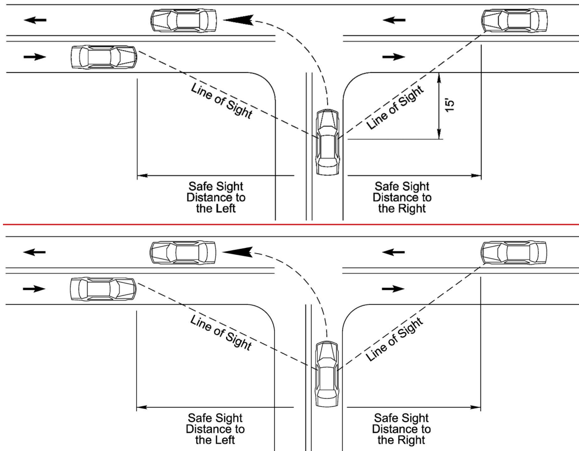
Figure 8-7 Intersection Sight Distance
