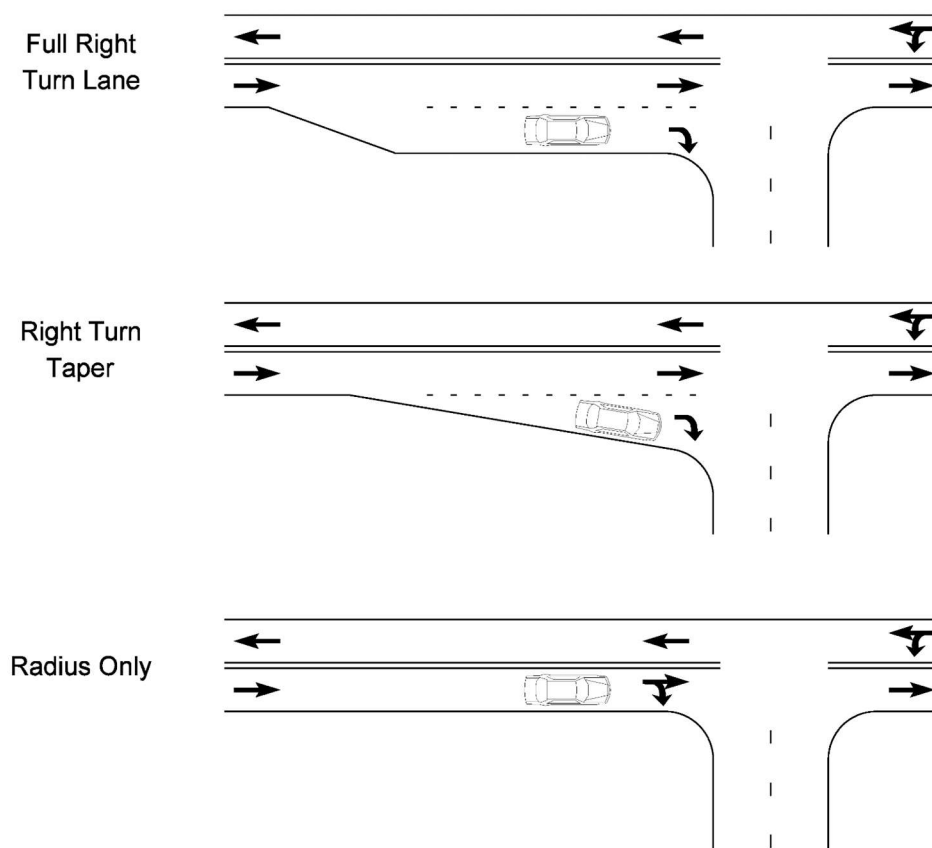
Figure 8-9 Turn Lanes
