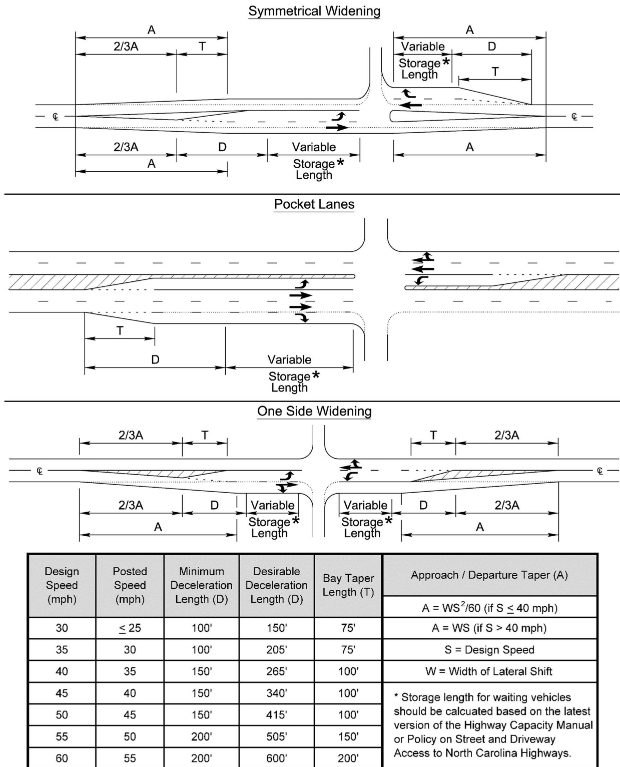
Figure 8-10 Recommended Treatment for Turn Lanes
