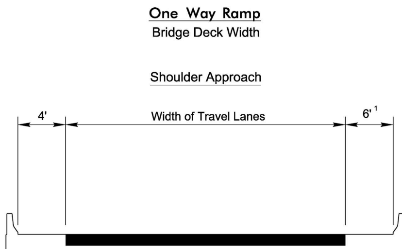
Figure 5-12 One Way Ramp Bridge Deck Widths
