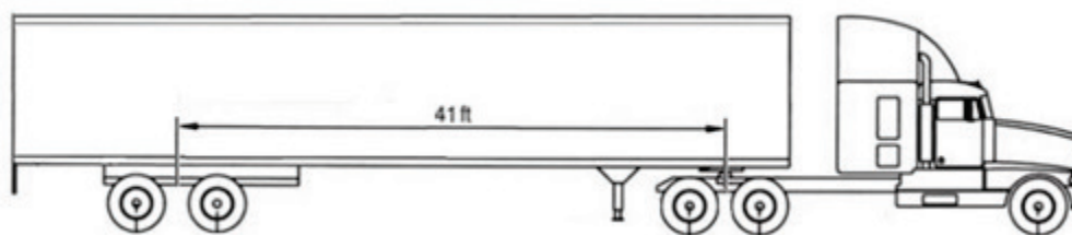
Figure 8-16 WB-62FL Truck
