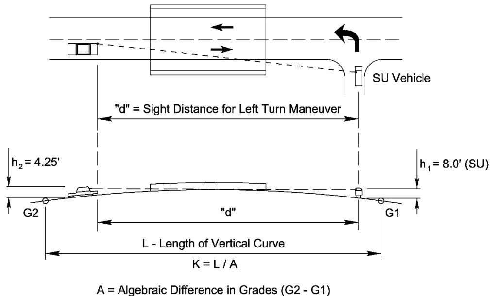
Figure 9-3 Vertical Sight Distance Control for Crest Curves at Interchanges, Single Unit Vehicle Criteria
