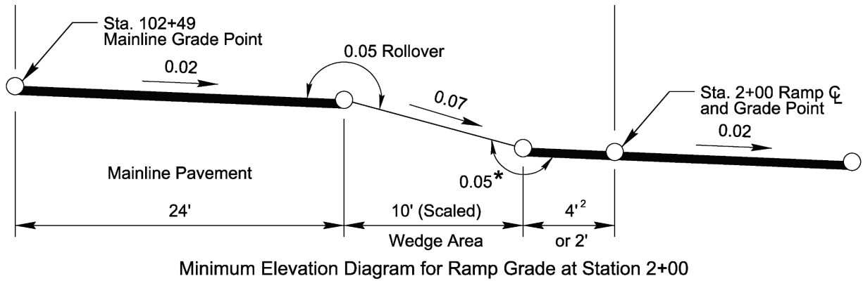
Figure 9-2 Maximum Grade Control Points in Gore Area
