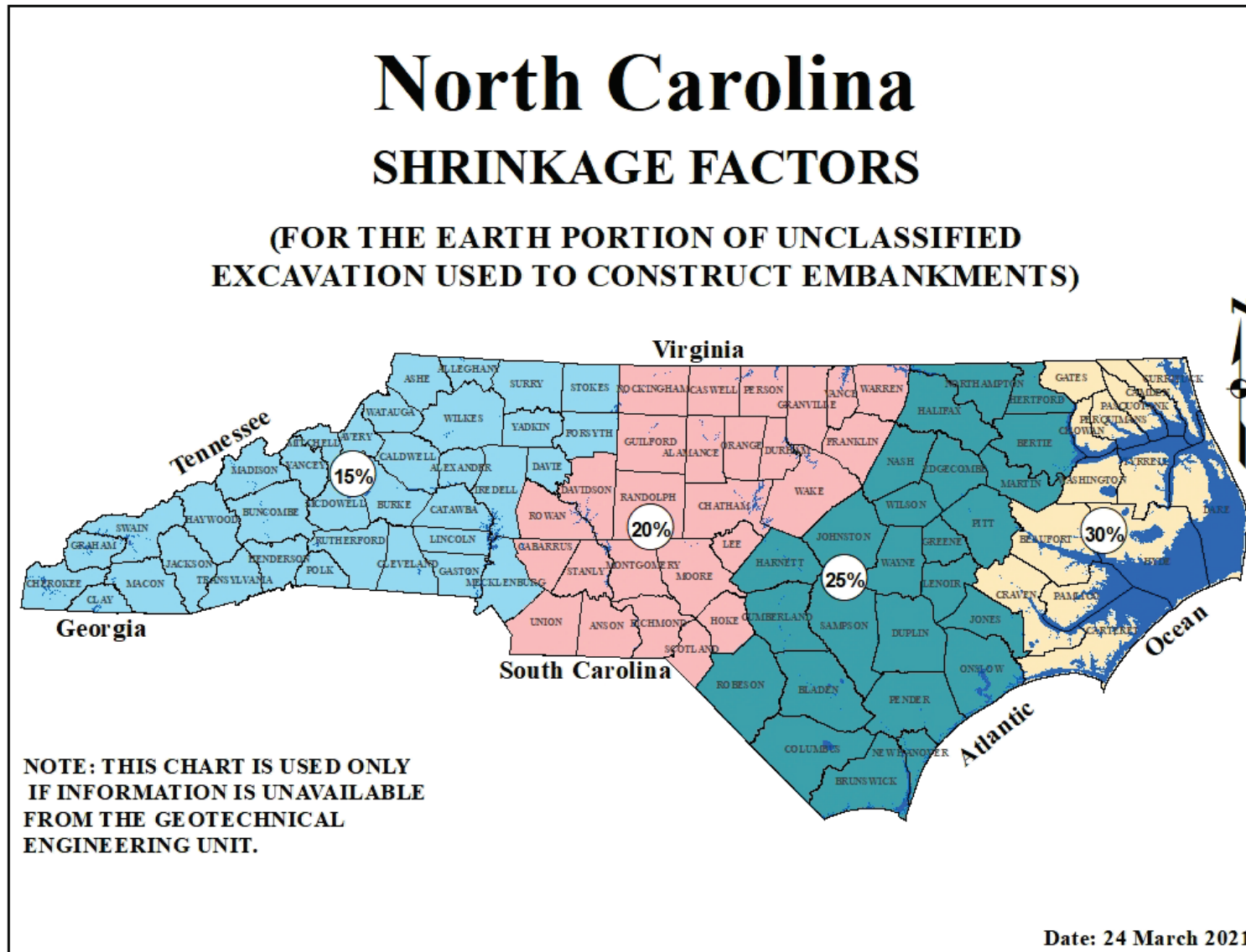
Figure 5-1 Shrinkage Factors
