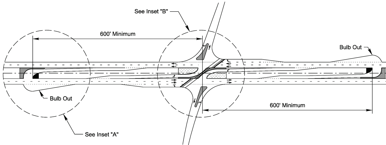
Figure 8-2 Reduced Conflict Intersection
