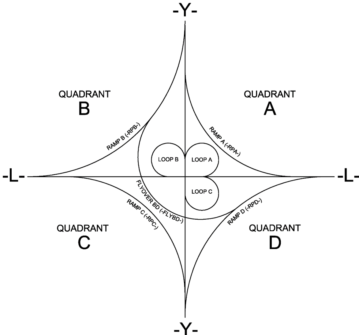
Figure 9-1 Interchange Quadrant Letter Designation
