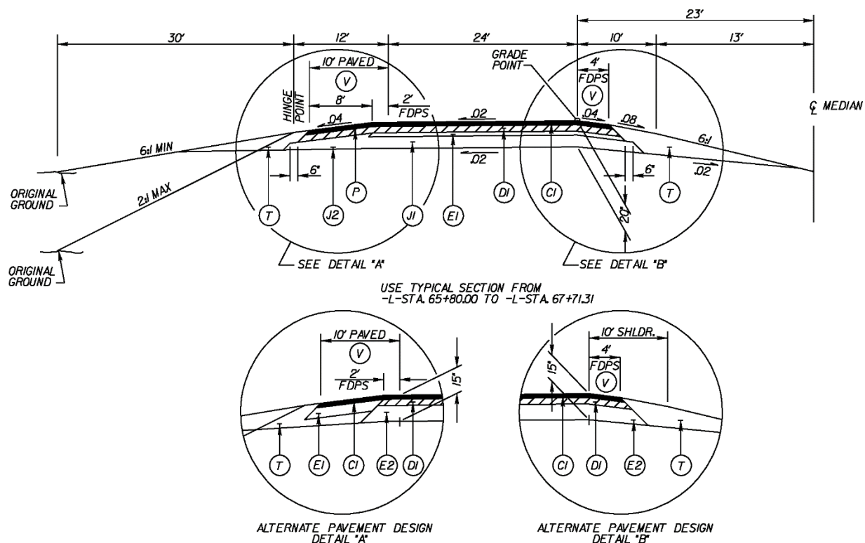
Figure 13-4 Pavement Alternate Base Course Material typical
