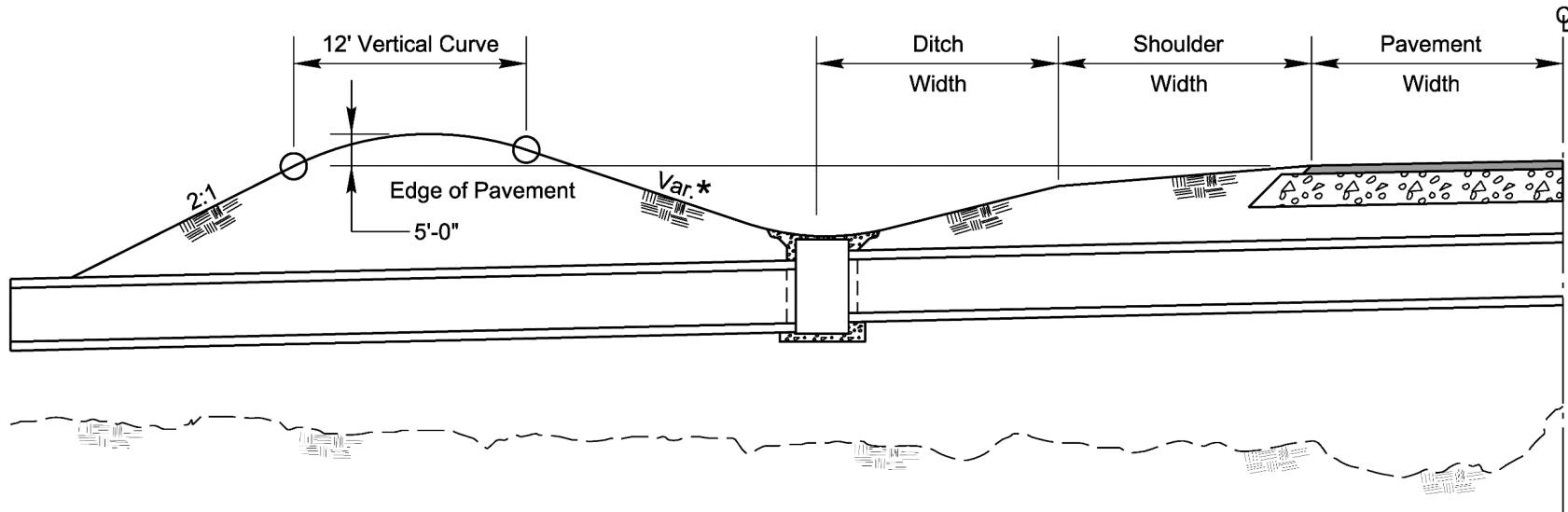
Figure 13-1 False Cut in Draw Between Cut Slopes
