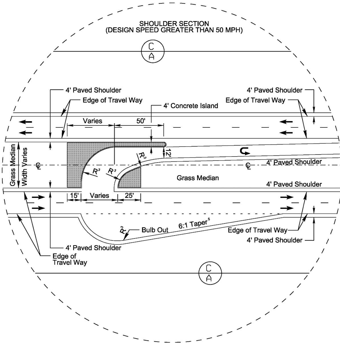
Figure 8-3b Reduced Conflict Intersection – Inset “A” Shoulder Section
