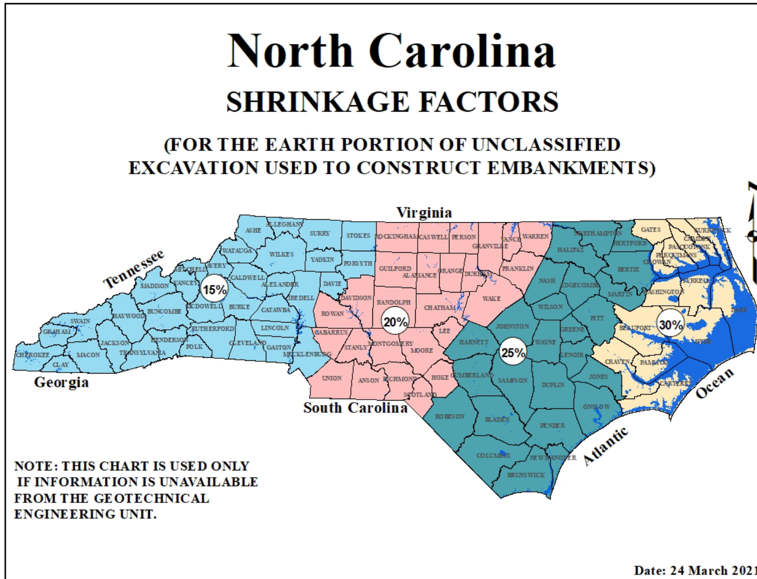
Figure 15-1 Shrinkage Factors
