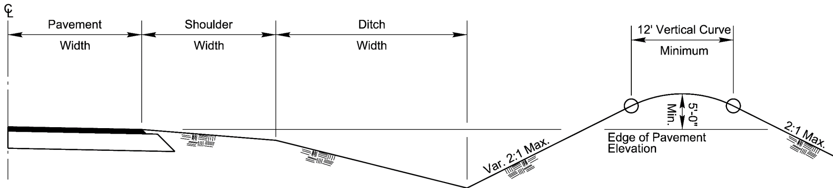
Figure 13-2 False Cut to be Used on Waste Projects Where Fill Height Exceeds 30"
