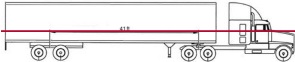
Figure 8-16 WB-62FL Truck
