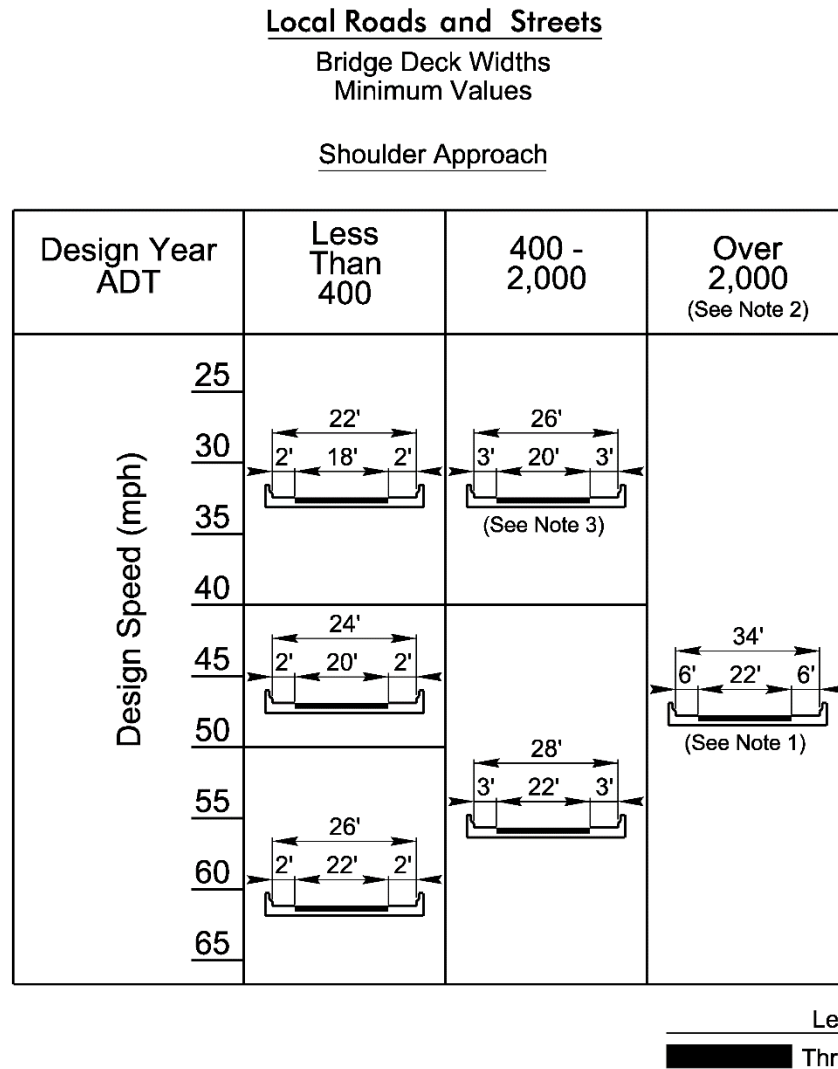
Figure 5-8 Local Roads and Streets Bridge Deck Widths
