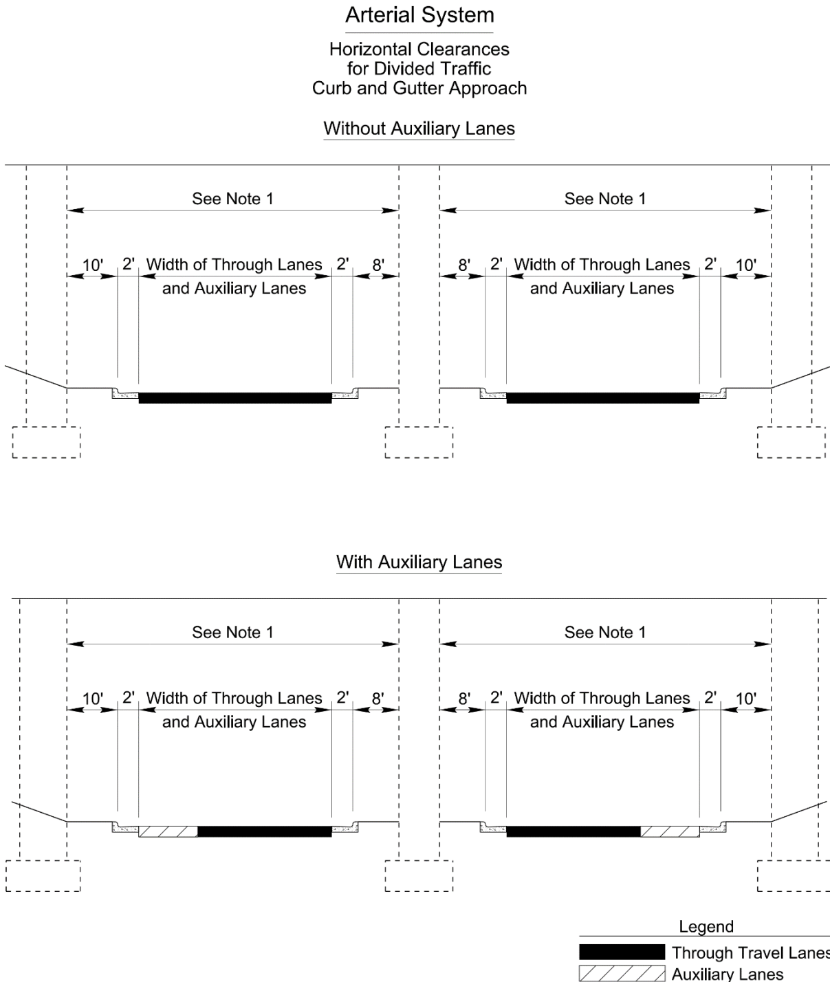
Figure 5-17 Arterial System Horizontal Clearances for Divided Traffic Curb and Gutter Approach
