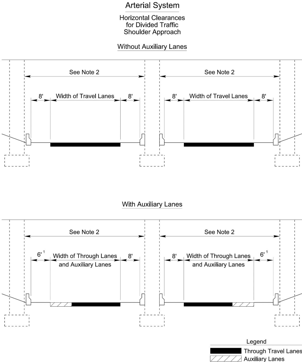
Figure 5-16 Arterial System Horizontal Clearances for Divided Traffic Shoulder Approach
