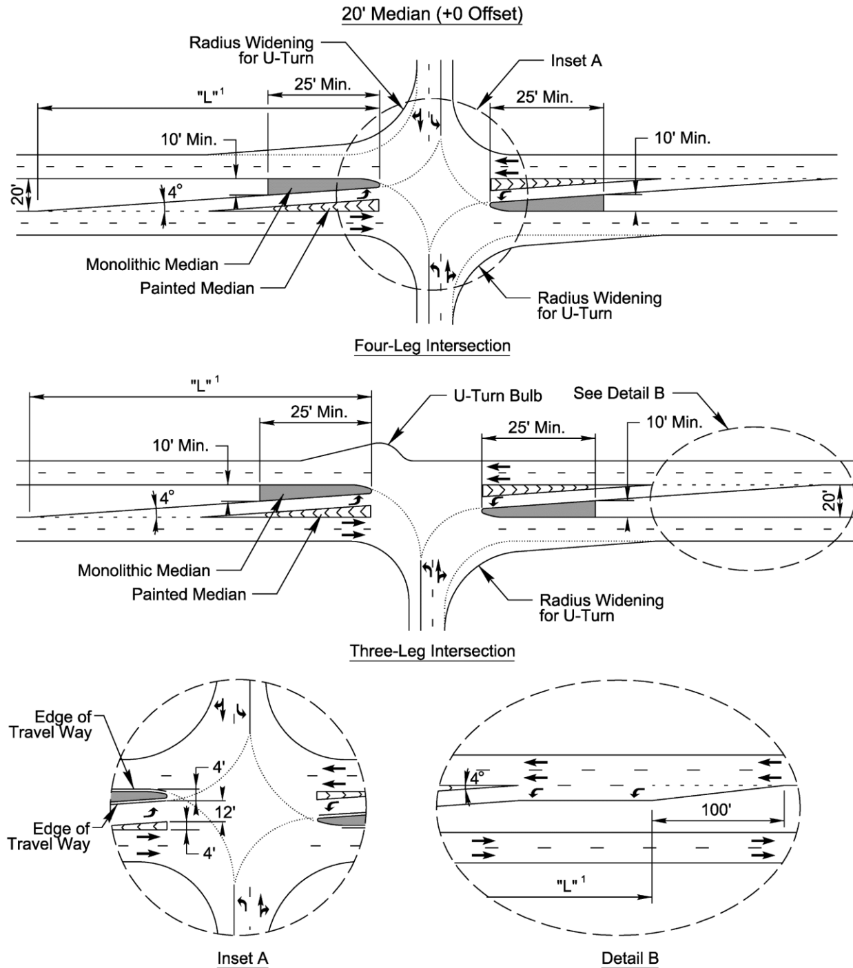
Figure 8-12 Guidelines for Offsetting Opposing Left Turn Lanes on Divided Roadways with a 20' Median
