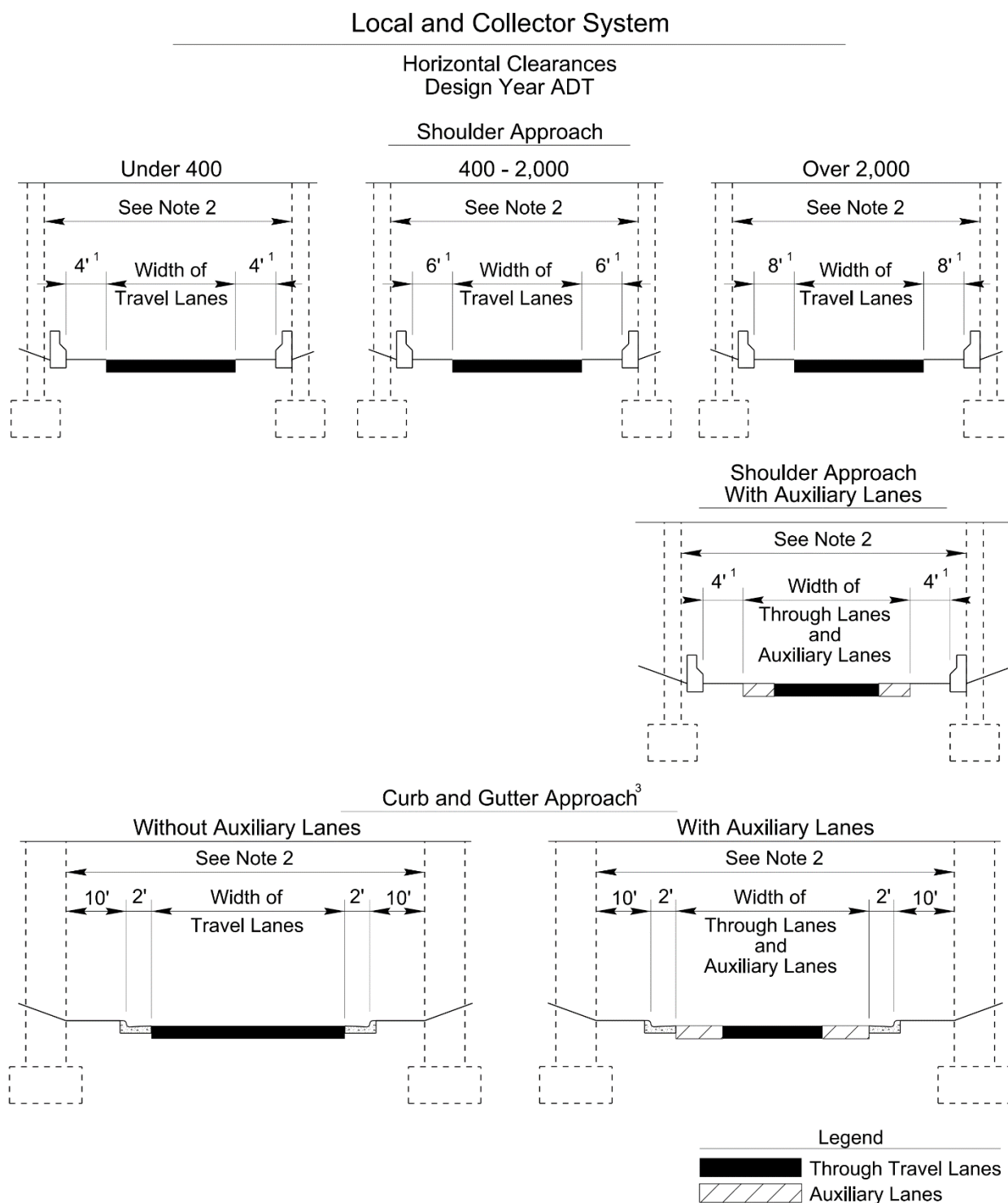
Figure 5-18 Local and Collector System Horizontal Clearances for Design Year ADT
