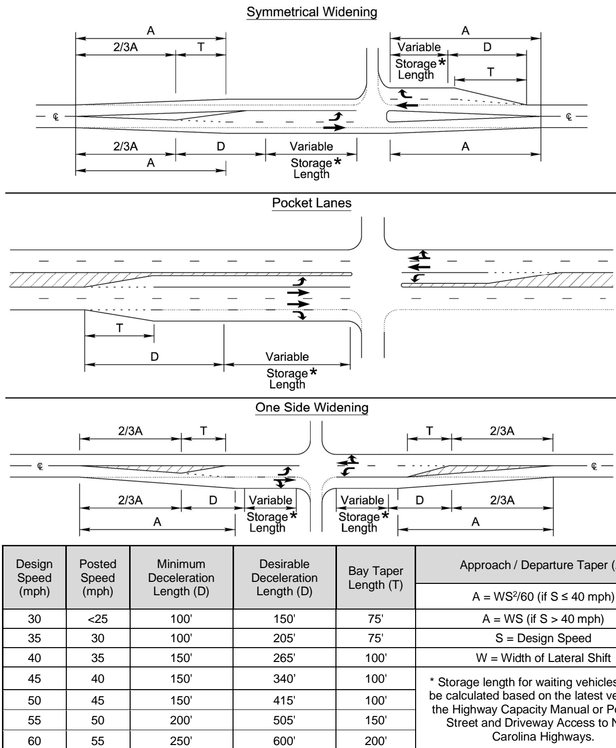
Figure 8-11 Recommended Treatment for Turn Lanes
