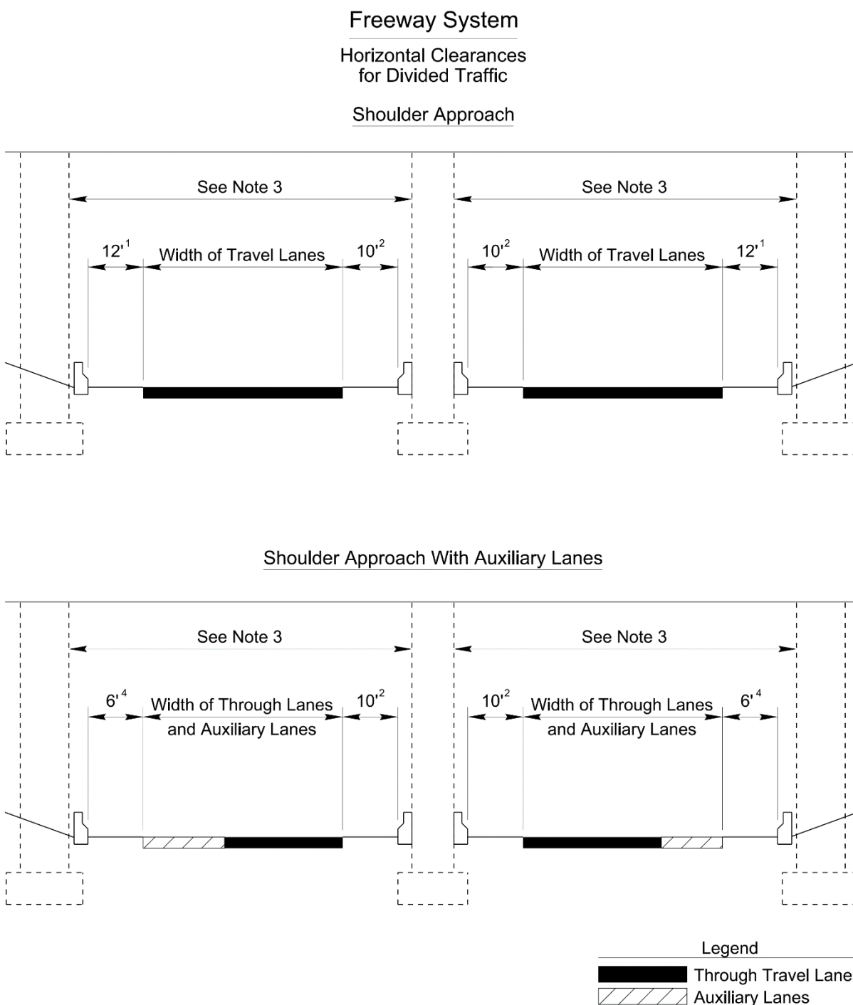
Figure 5-14 Freeway System Horizontal Clearances for Divided Traffic
