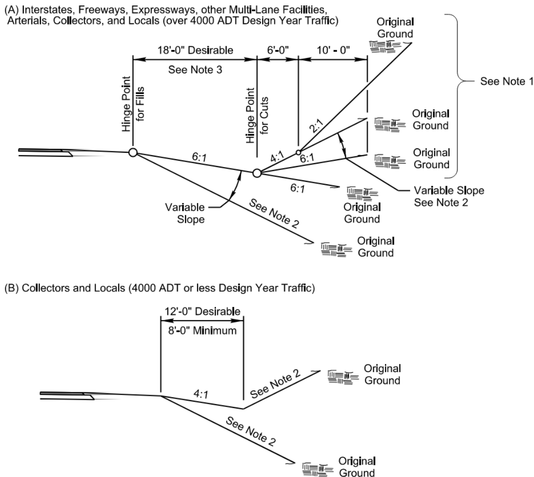
Figure 4-4 Criteria for Roadway Typical Section and Slopes
