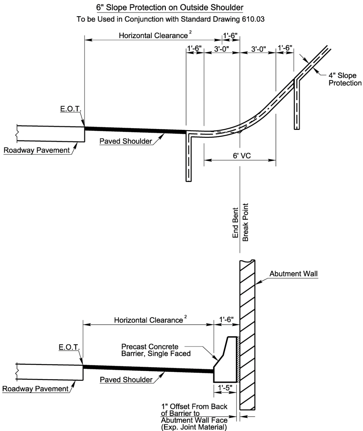
Abutment Wall on Outside Shoulder To be Used in Conjunction with Standard Drawing 610.04
