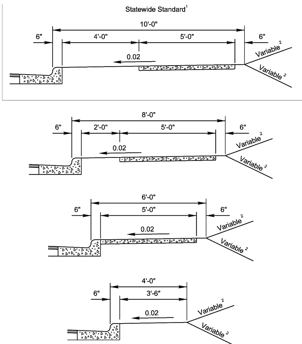
Figure 4-6 Berm Width
