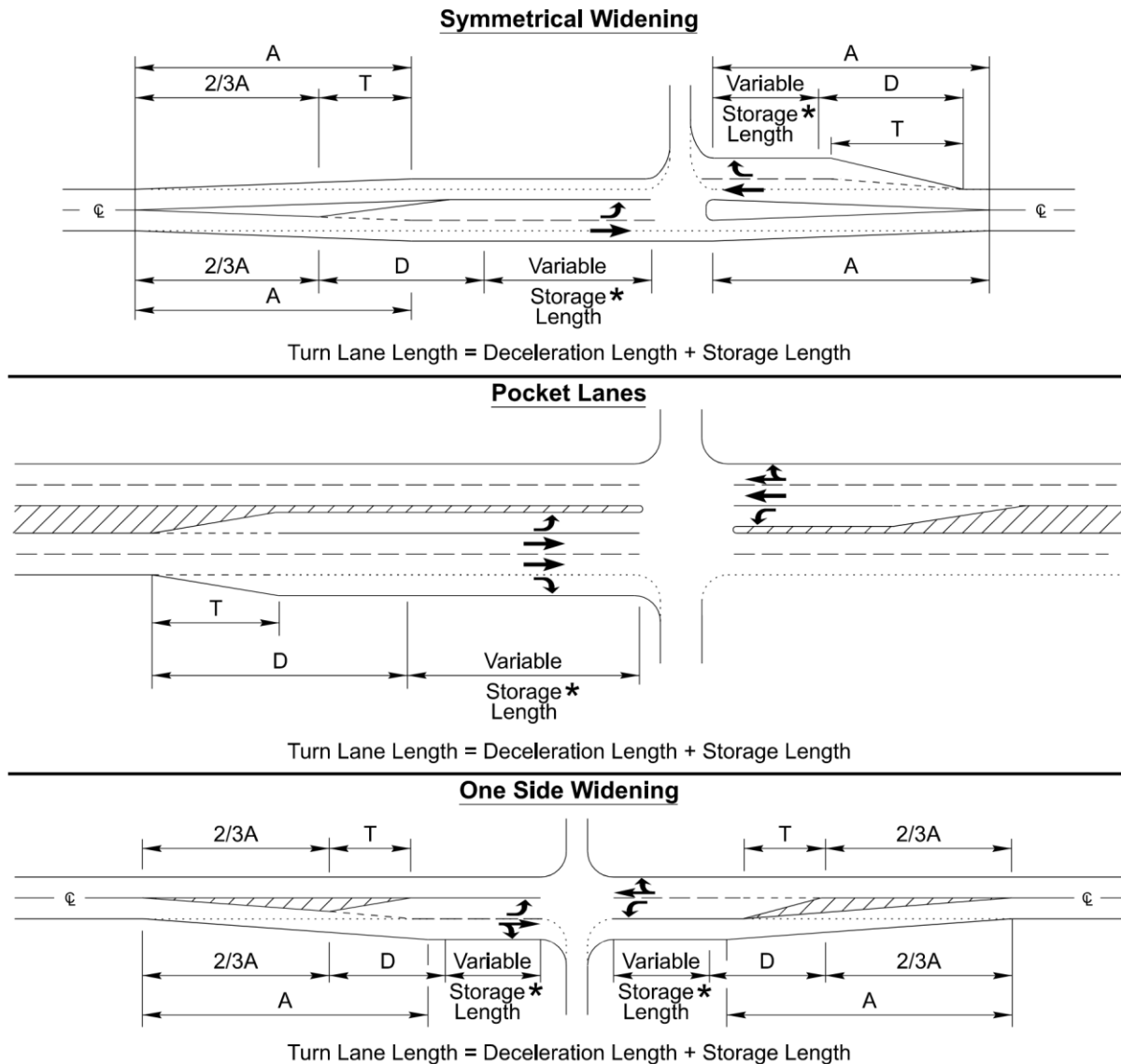
Figure 8-11 Recommended Treatment for Turn Lanes
