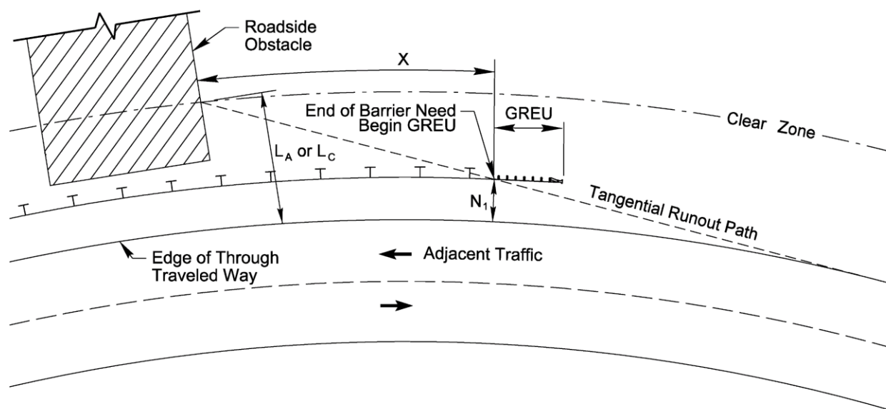
Figure 6-4 Detail of Guardrail Placement on Approach End of Hazard Located on Horizontal Curve
