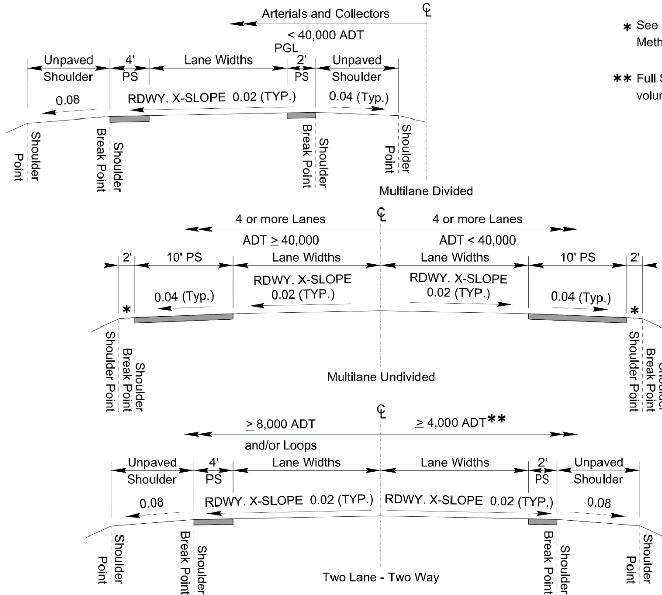
Figure 4-3 Typical Shoulder Cross Slopes (cont.)
