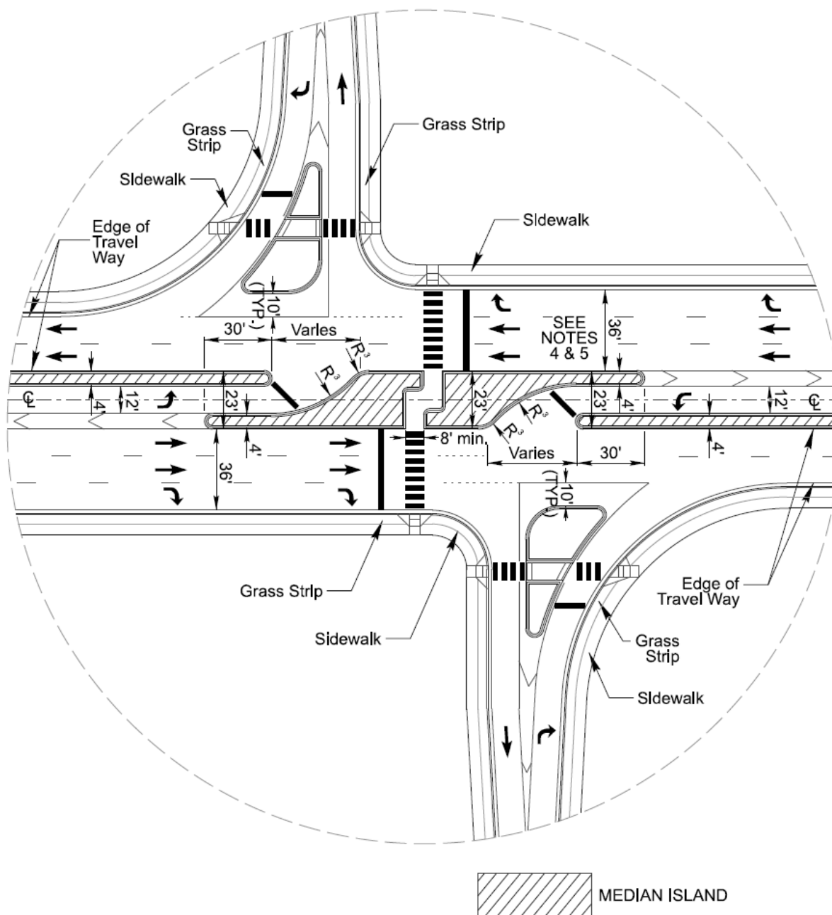
Figure 8-3a Reduced Conflict Intersection – Inset “B” – 23-foot Median - Desirable
