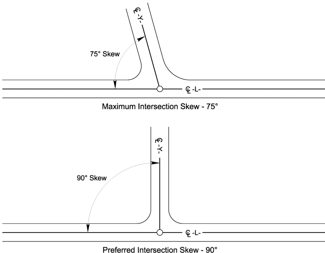
Figure 8-4 Desirable Intersection Skews
