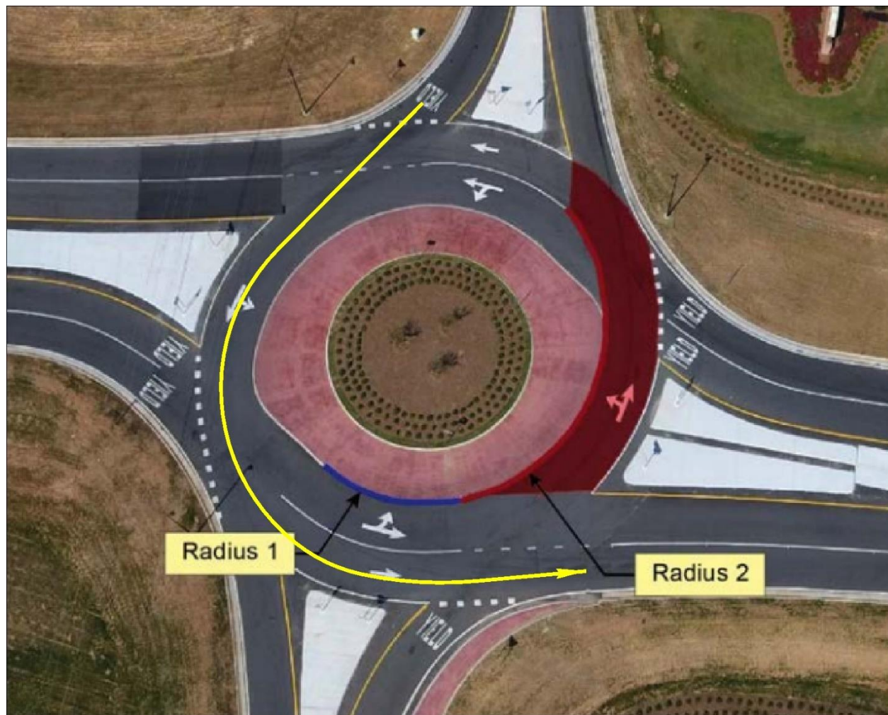
Figure 8-17 Spiraling in a 2x1 Roundabout
