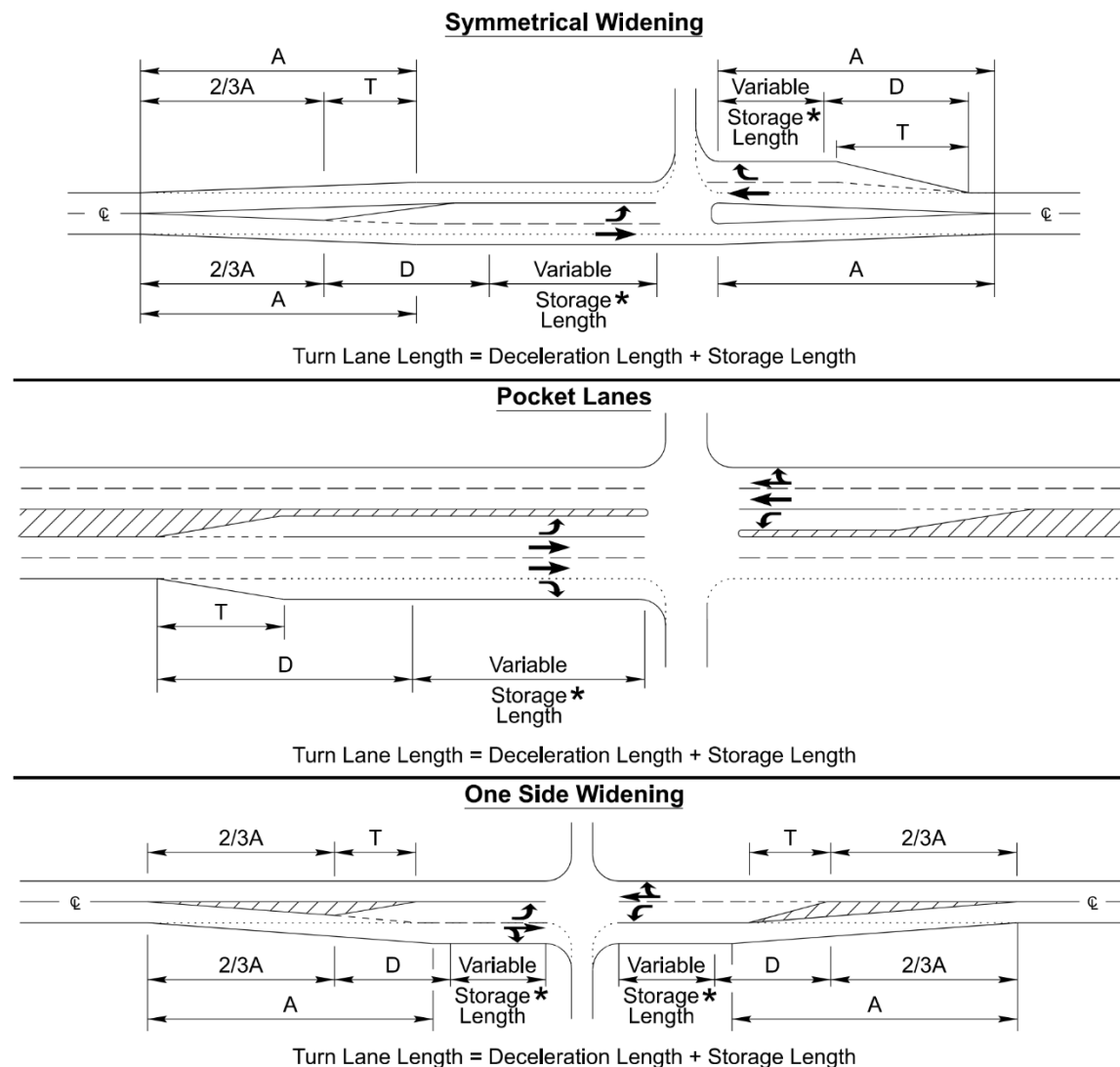
Figure 8-10 Recommended Treatment for Turn Lanes
