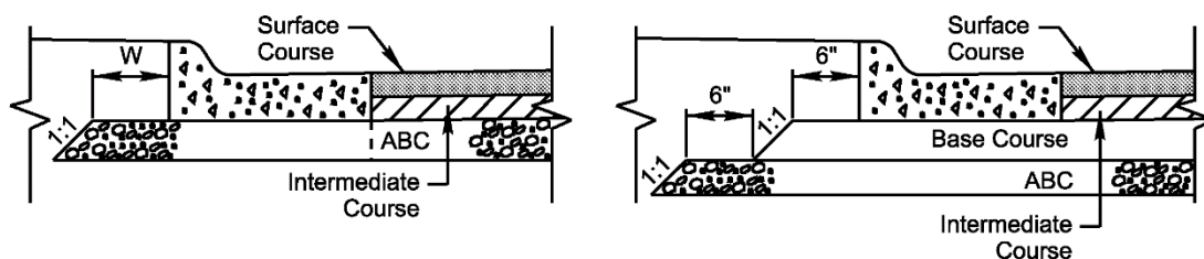
Figure 2-4 Pavement Edge Construction with Shoulder Drains
