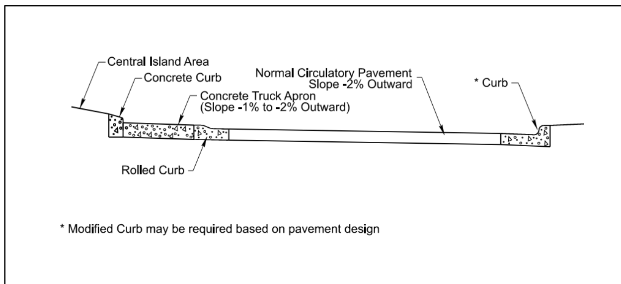
Figure 8-16 Example Roundabout Typical Section
