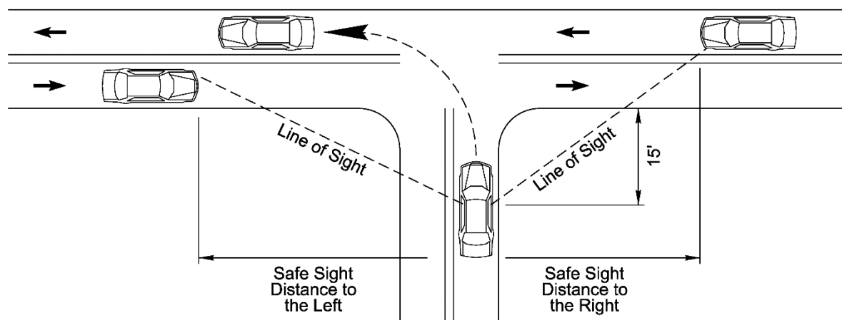
Figure 8-6 Intersection Sight Distance
