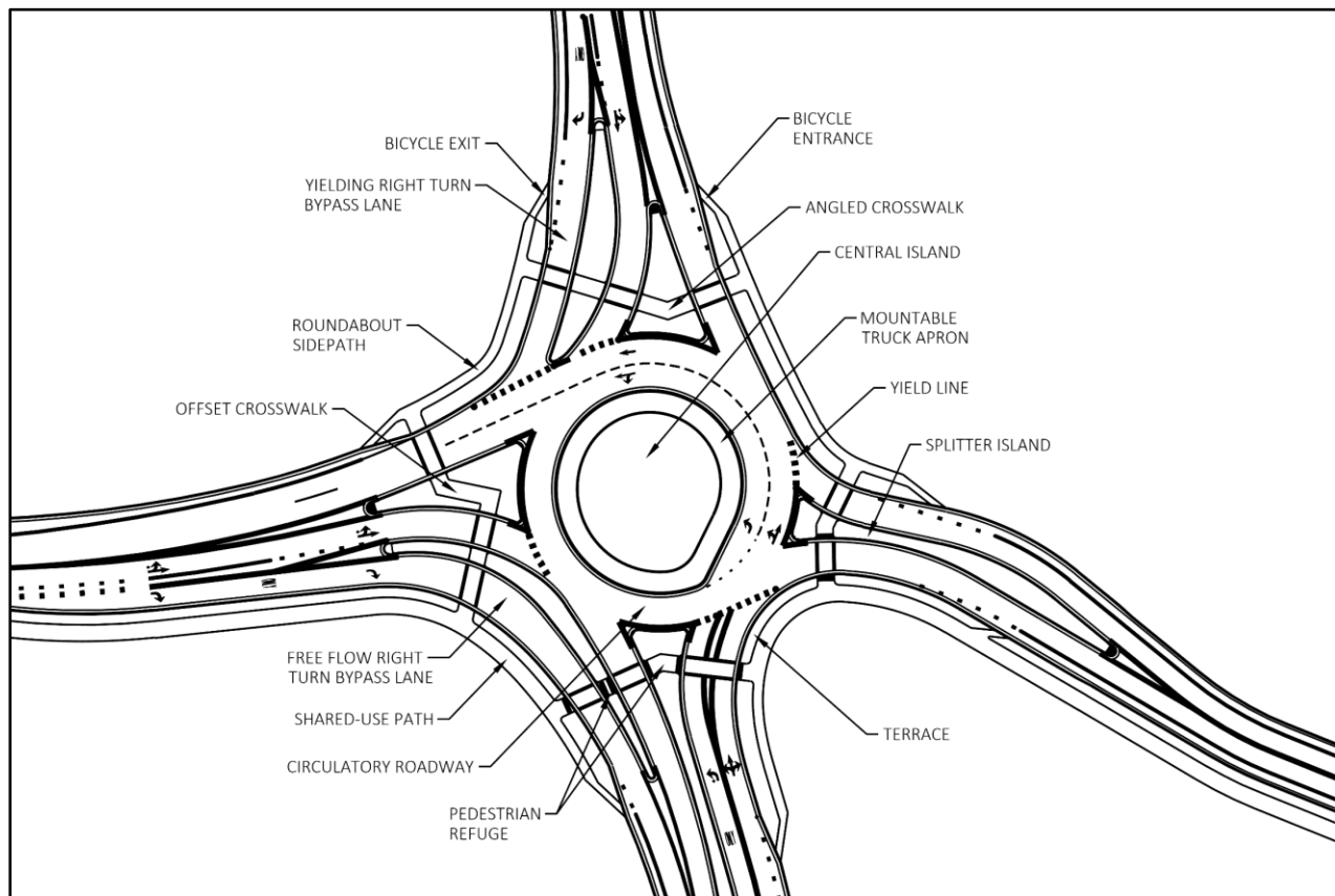
Figure 8-15 Roundabout Common Features
