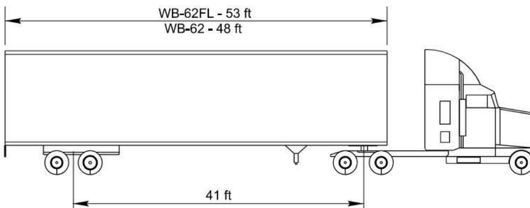
Figure 8-7 WB-62 and WB-62FL Truck Dimensions
