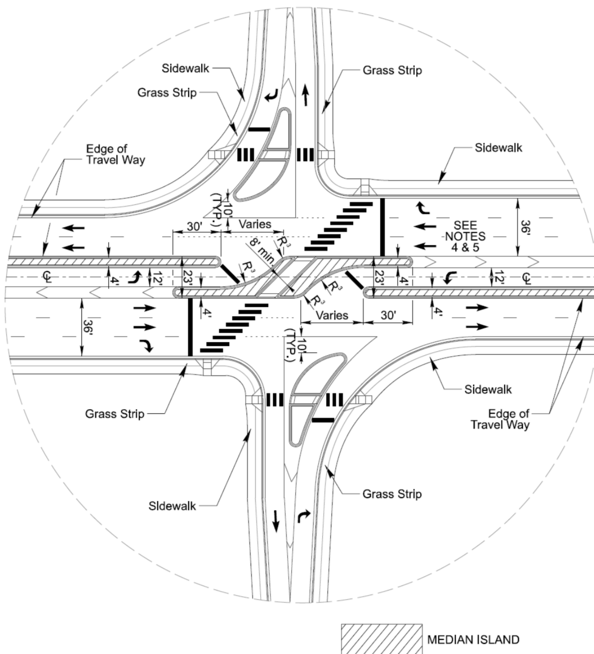
Figure 8-3b Reduced Conflict Intersection – Inset “B” – 23-foot Median – Right of Way Constrained
