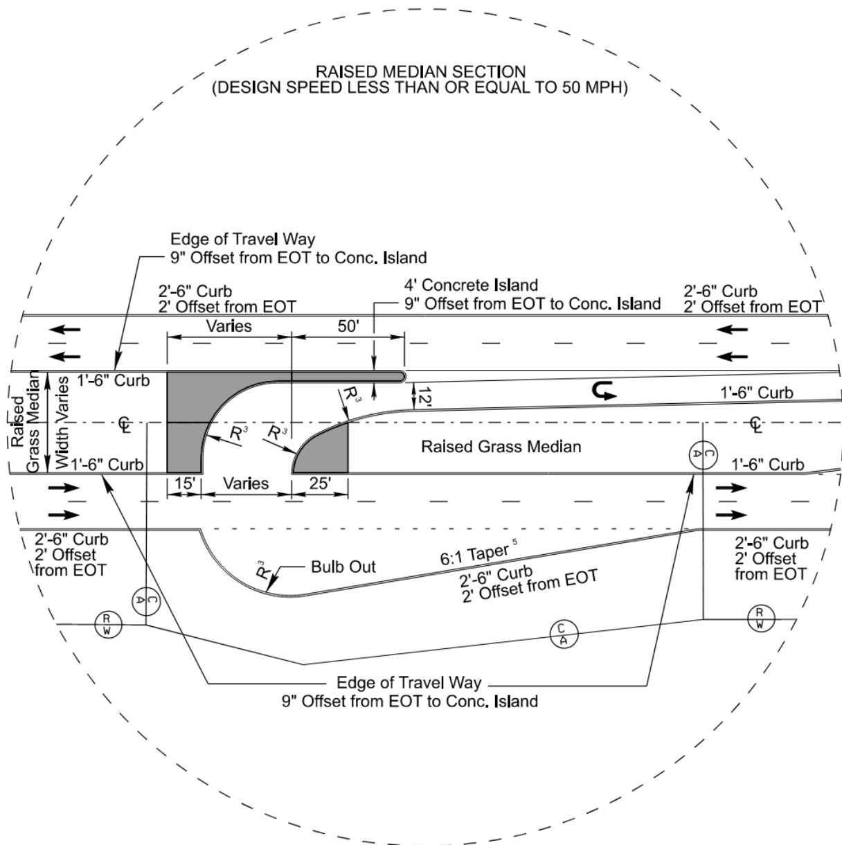
Figure 8-2a Reduced Conflict Intersection – Inset “A” Raised Median Section
