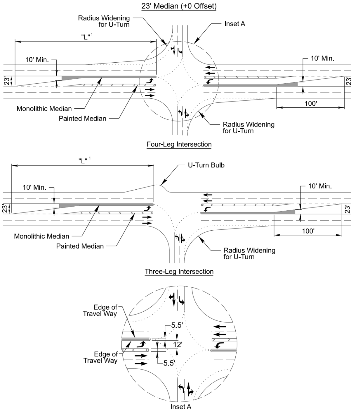
Figure 8-11 Guidelines for Offsetting Opposing Left Turn Lanes on Divided Roadways with a 23' Median
