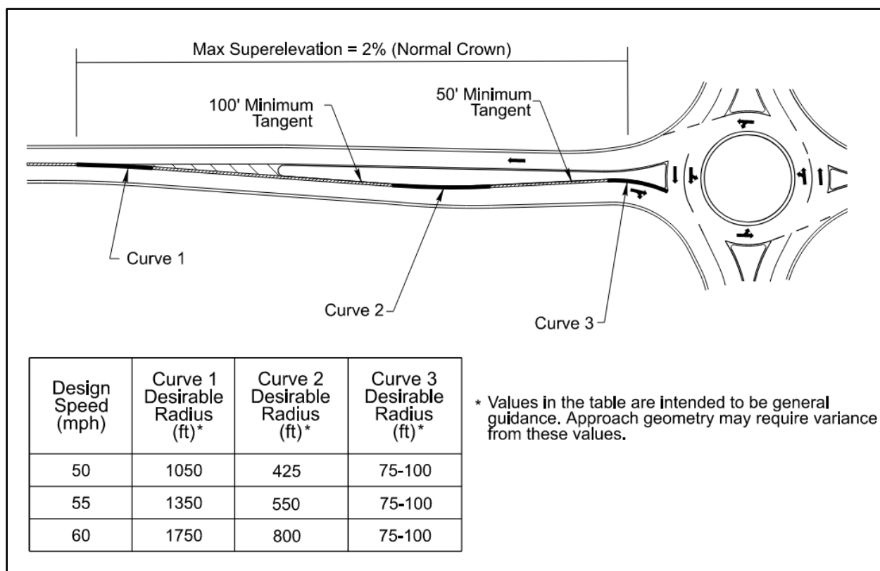
Figure 8-18 High-Speed Roundabout Approach
