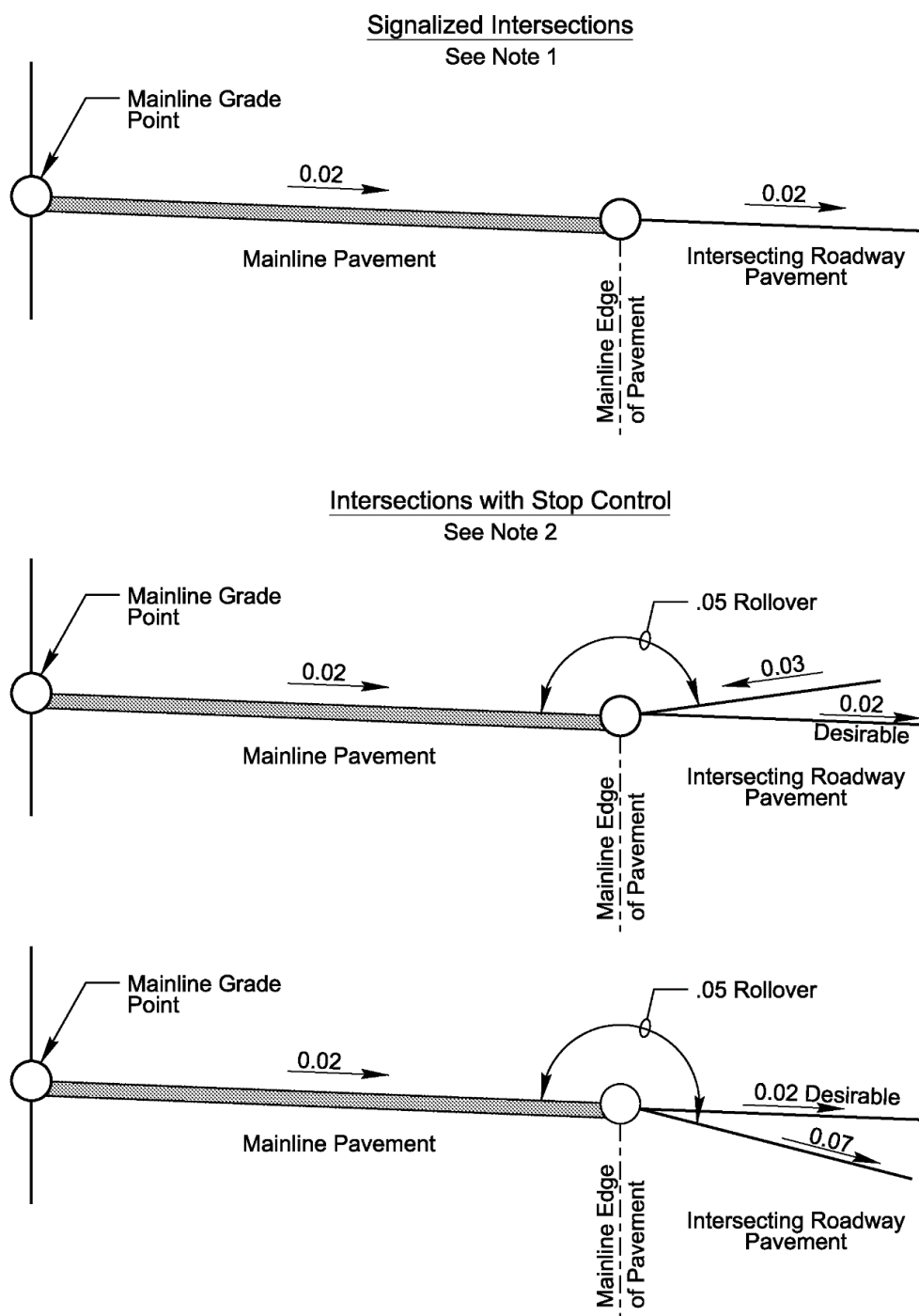
Figure 8-5 Profile Rollover at Intersections
