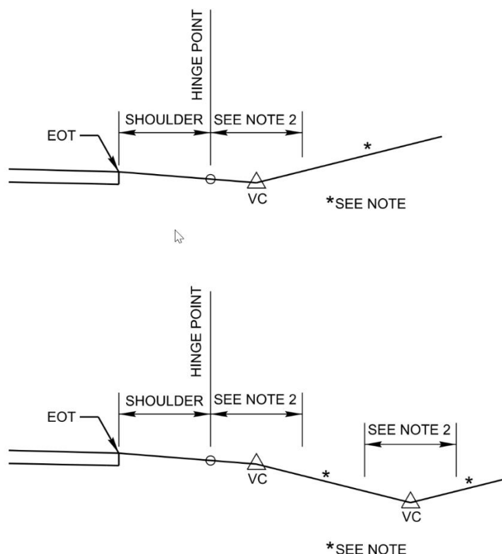
Figure 4-8 Commercial and Residential Driveway Profile
