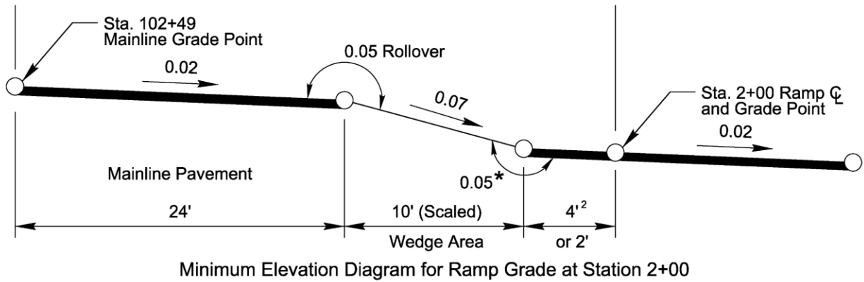
Figure 9-3 Maximum Grade Control Points in Gore Area
