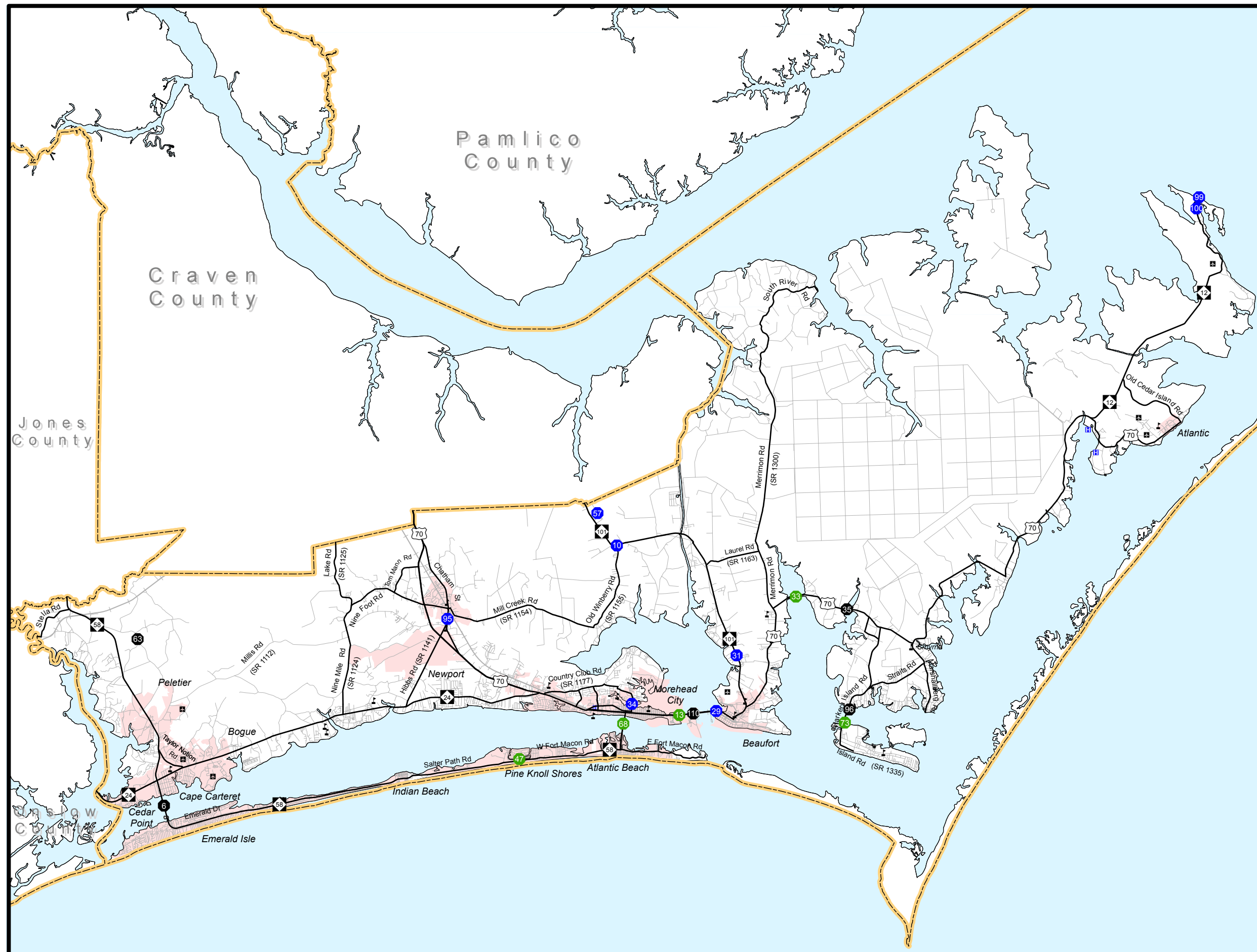
Figure 5 Deficient Bridges
