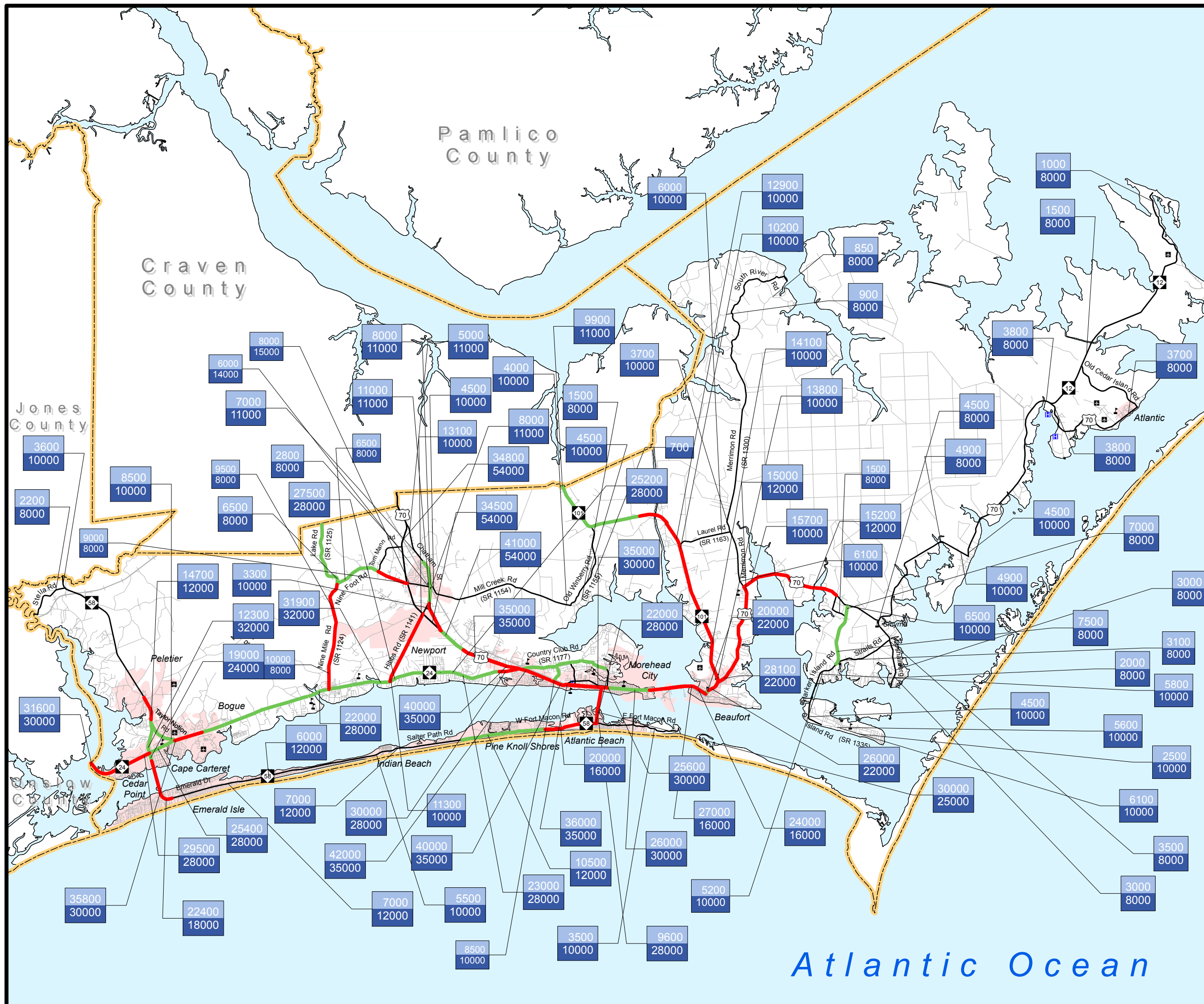
Figure 2 2040 Volumes and Capacity Deficiencies
