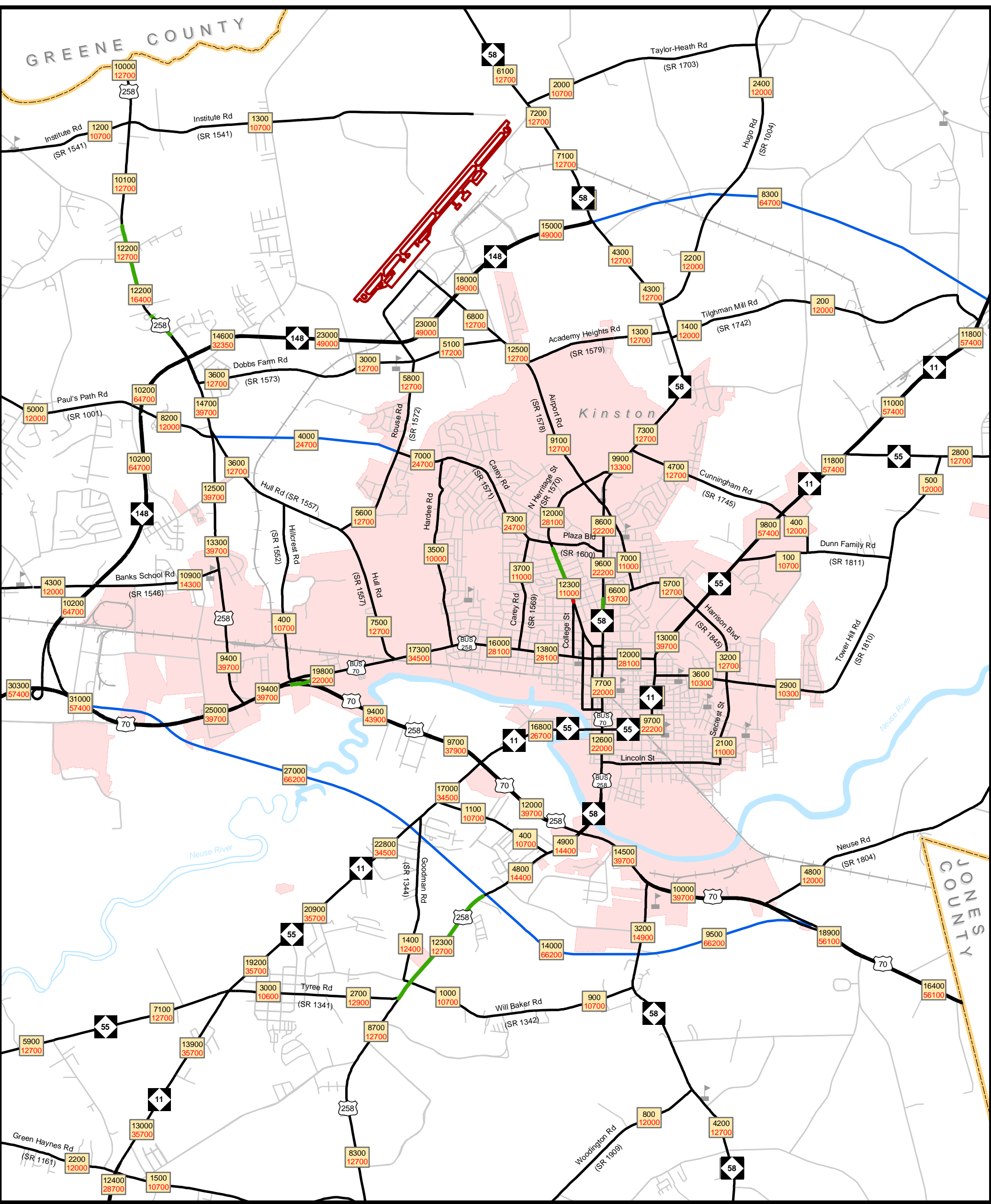
Figure 3A 2045 Volumes and Capacity Deficiencies with Committed Projects
