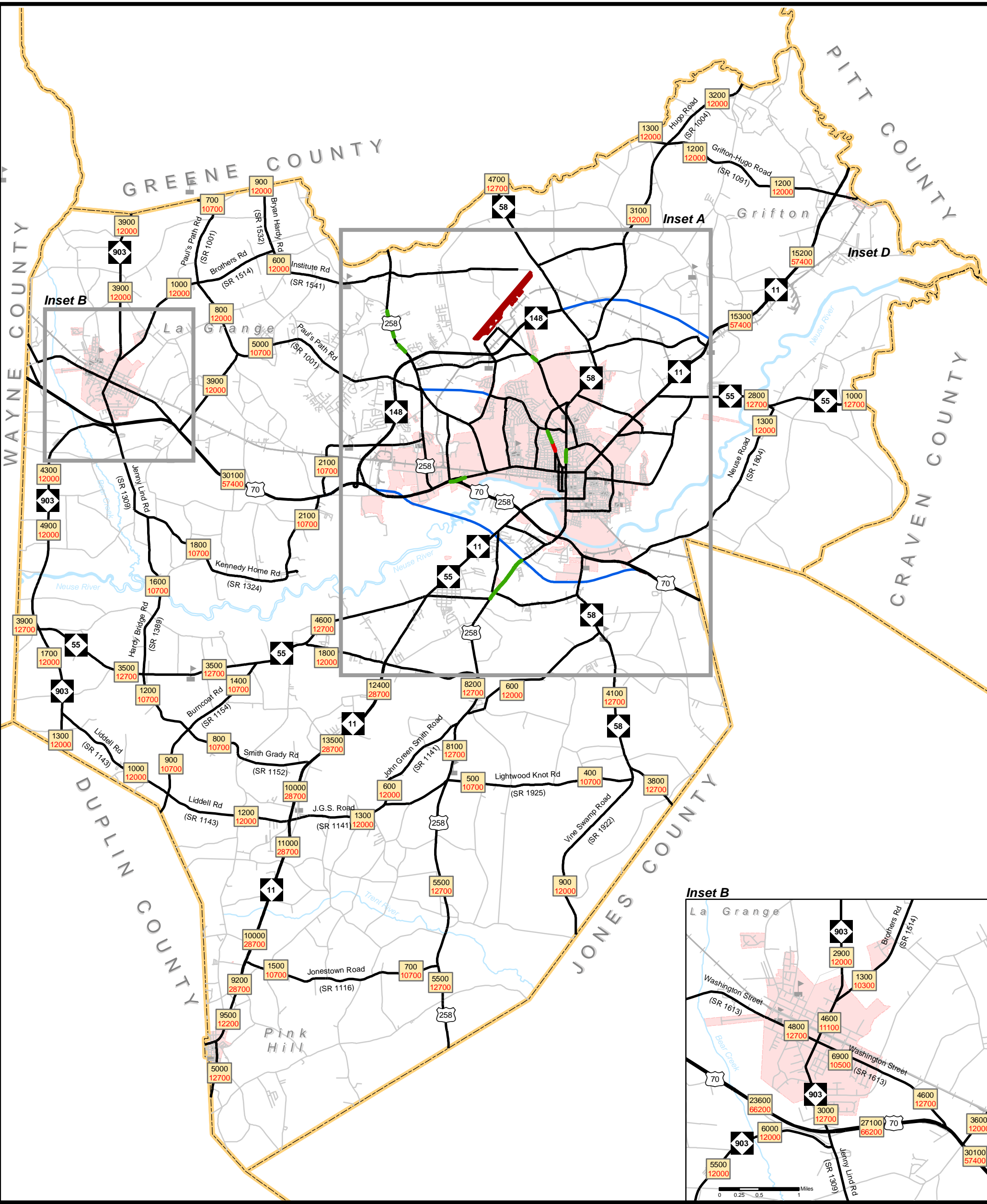
Figure 3 2045 Volumes and Capacity Deficiencies with committed projects
