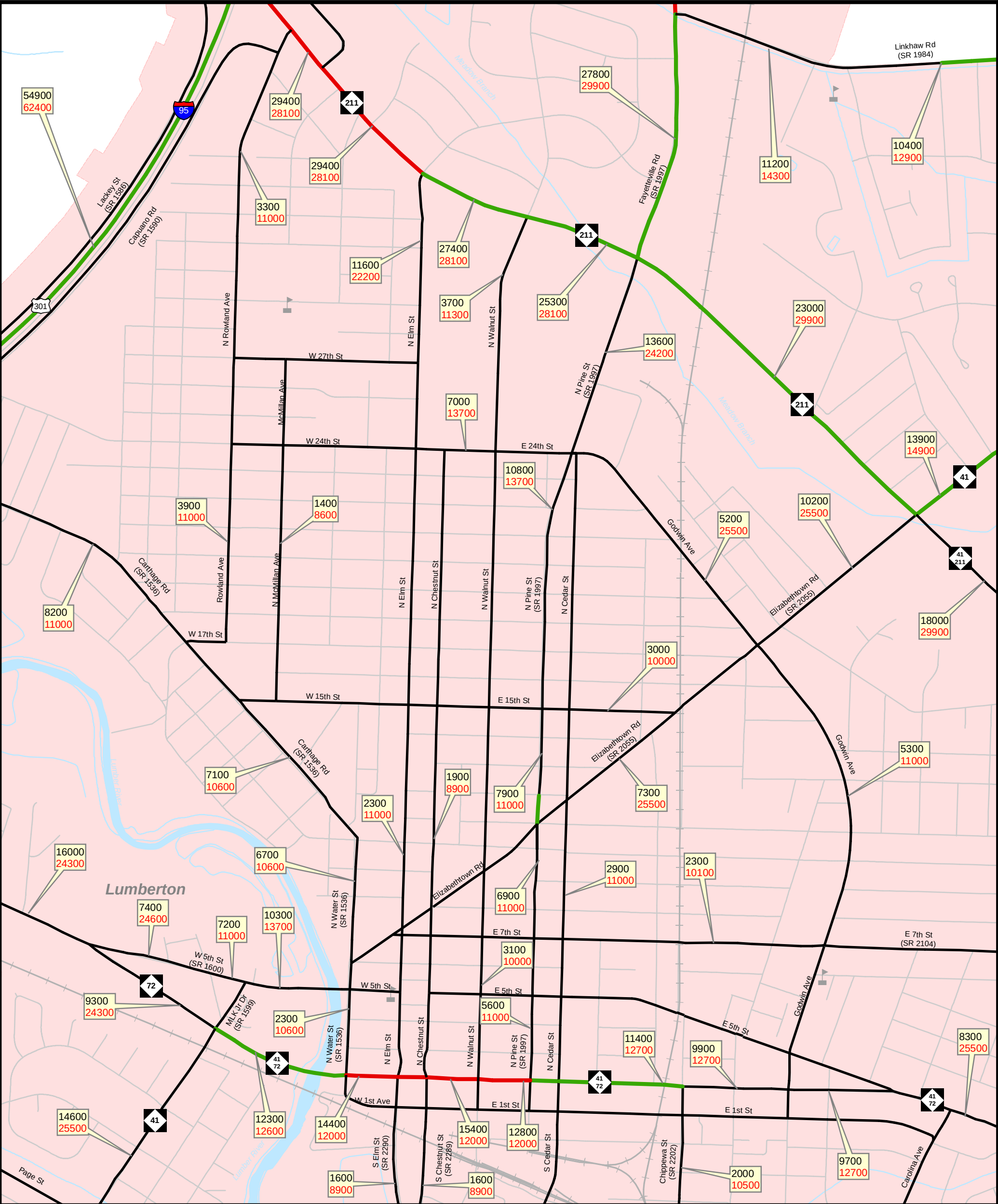
Figure 3, Inset A 2020 Volumes and Capacity Deficiencies
