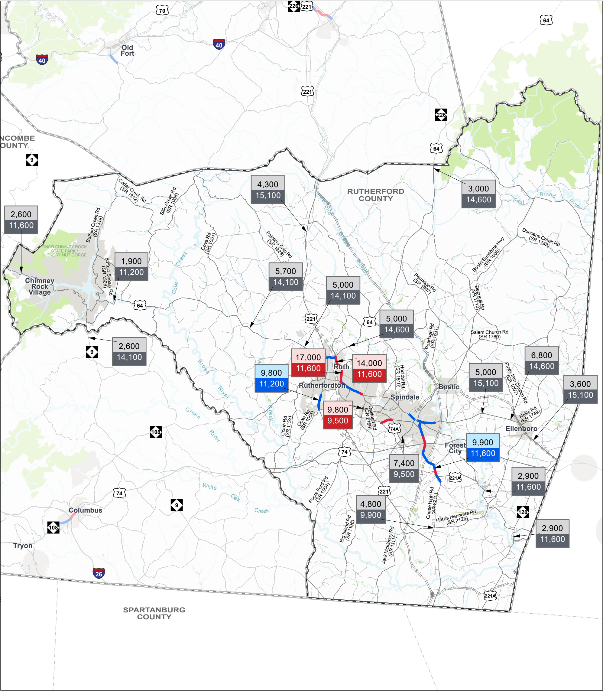
Figure 2 2017 VOLUME AND CAPACITY DEFICIENCIES
