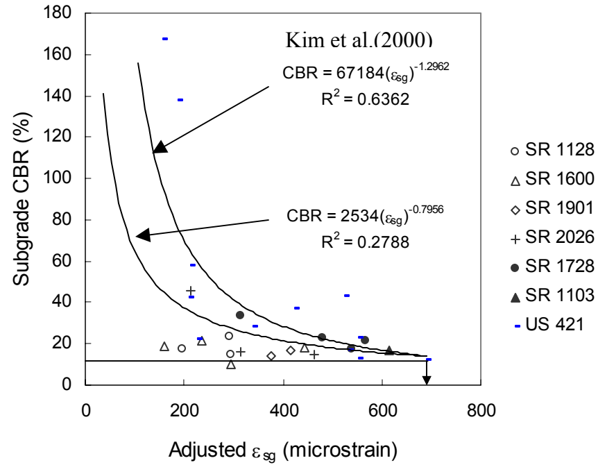
Figure 4.22. Adjusted \varepsilon_{sg} as a subgrade condition indicator for aggregate base pavements.
