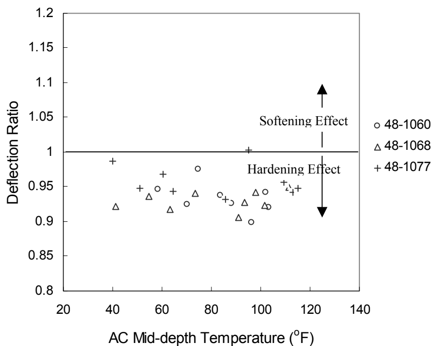
Figure 4.51. Deflection ratio versus AC mid-depth temperature for pavements with a gravel base layer.
