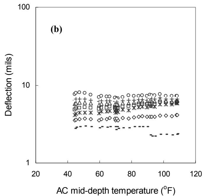
Figure 3.5. NCDOT corrected deflection versus mid-depth temperature for: (a) US 264; (b) US 17.
