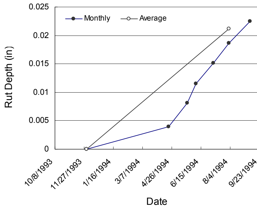
Figure 5.16. Predicted rut depths using the deflections at monthly and average spring/summer AC mid-depth temperatures for the 48-1060 section.
