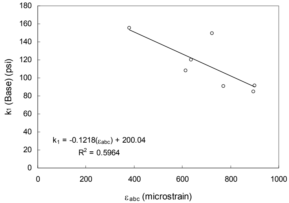
Figure 4.40. Adjusted \epsilon_{abc} versus k_1 of aggregate base for LTPP test sections.
