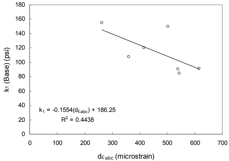
Figure 4.41. Adjusted d\epsilon_{abc} versus k_1 of aggregate base for LTPP test sections.
