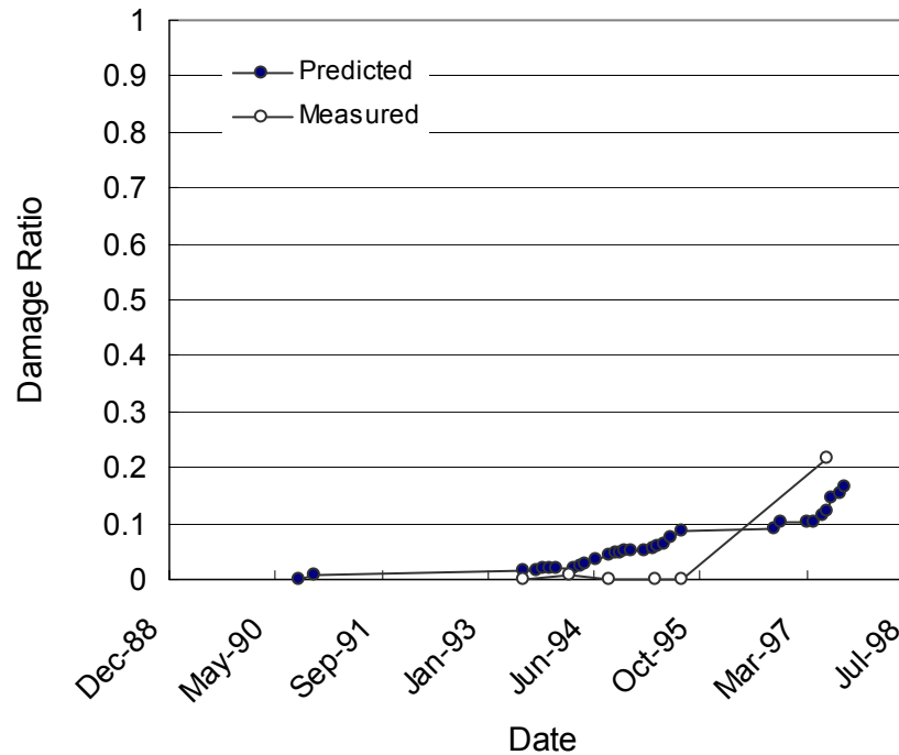
Figure 5.12. Predicted and measured damage ratios due to fatigue cracking for the 27-6251 section (wet freeze region).
