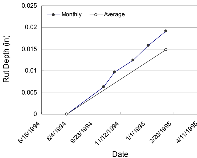
Figure 5.17. Predicted rut depths using the deflections at monthly and average fall/winter AC mid-depth temperatures for the 48-1060 section.
