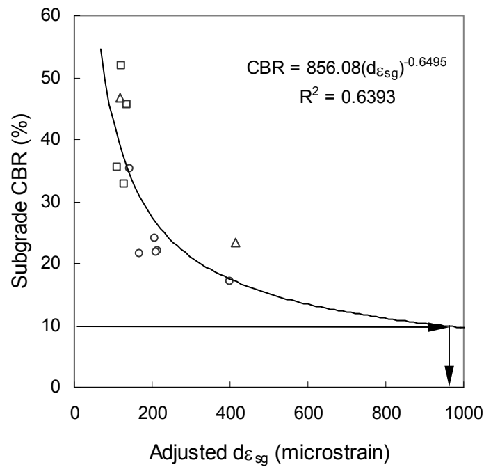
Figure 4.4. Adjusted d\varepsilon_{sg} as a subgrade condition indicator for full depth pavements.
