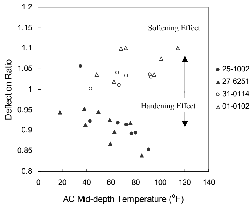
Figure 4.544 Effect of subgrade soil type on nonlinear behavior of a pavement structure.
