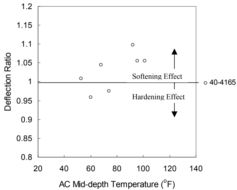
Figure 4.53. Deflection ratio versus AC mid-depth temperature for pavements with a HMAC base layer.
