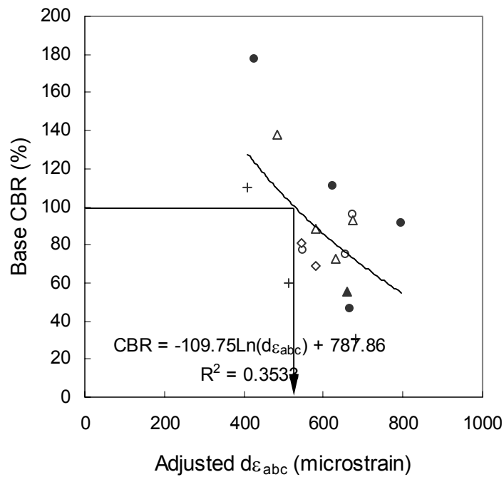
Figure 4.19. Adjusted d\varepsilon_{abc} as a base condition indicator for aggregate base pavements.
