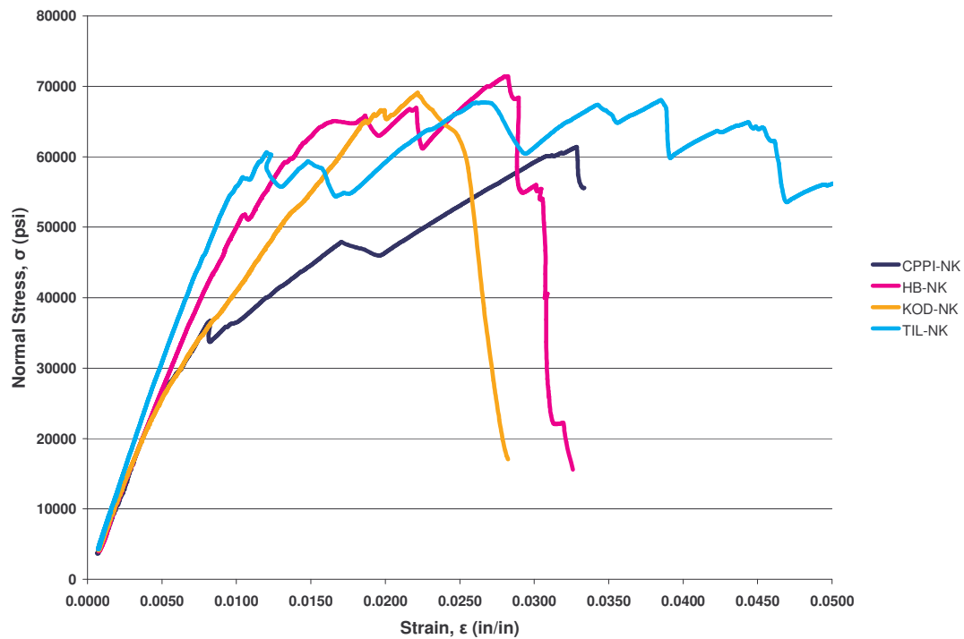
Figure H.12 Tensile Stress vs. Strain for Nicked at Room Temperature at 6 Months
