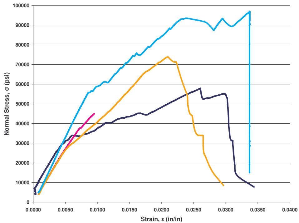
Figure H.4 Tensile Stress vs. Strain for Nicked at Room Temperature for 3 Months
