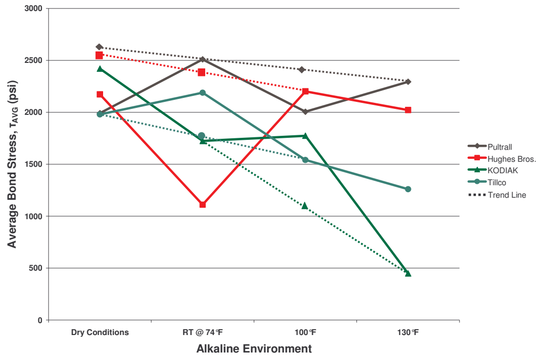
Figure 7.44 Trend Line of Bond Stress for 5\phi_b at 6 Months
