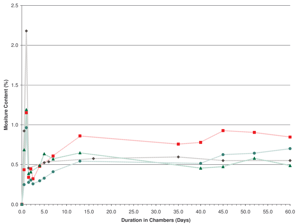
Figure 7.21 Weight-Based Effects Due to Moisture Uptake of Nicked Specimens at Room Temperature
