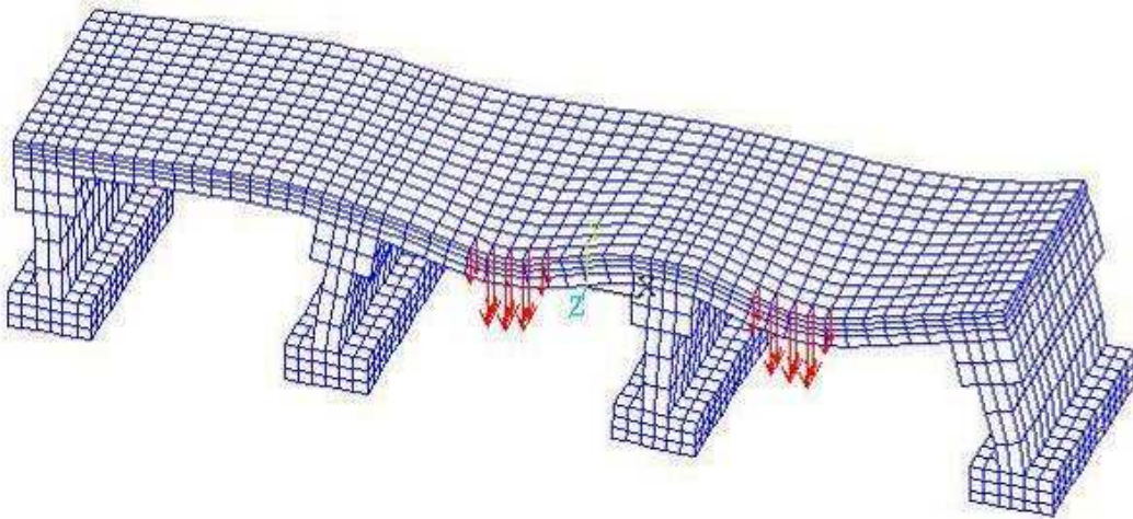
Figure 3.18 General View of the Deformed Shape (Half of the Lab Model)
