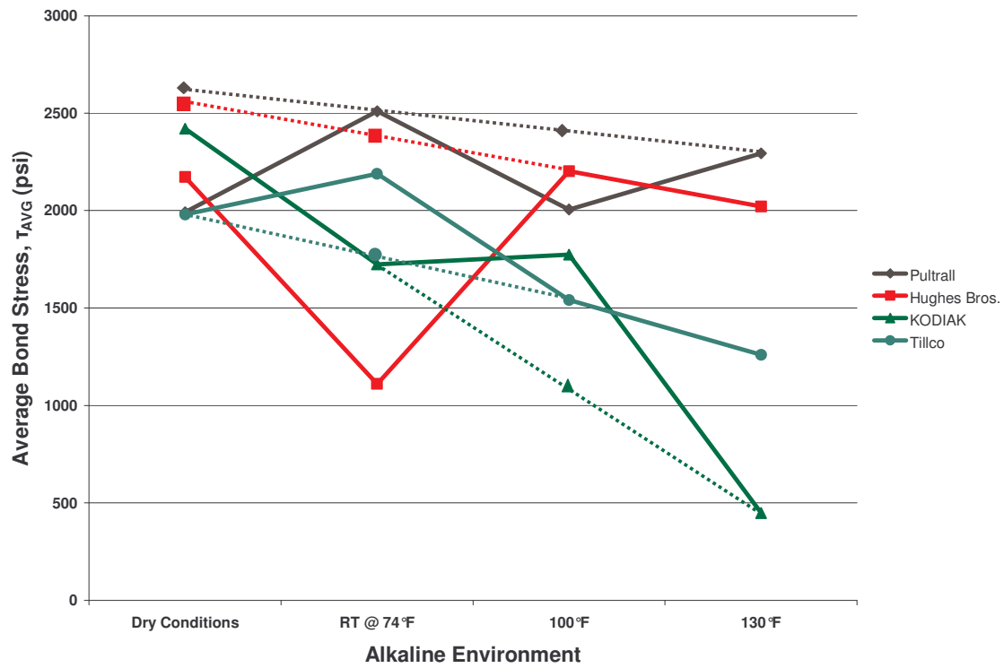
Figure 7.45 Trend Line of Bond Stress for 5\phi_b at 12 Months
