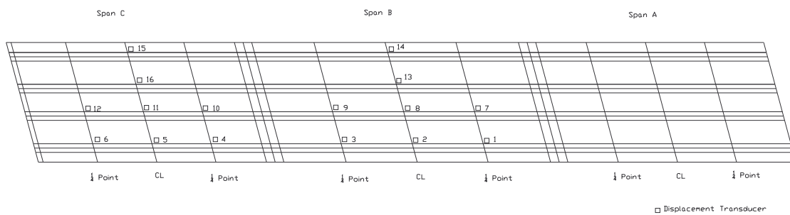
Figure 4.46 Bridge Instrumentation – Displacement Transducer Location
