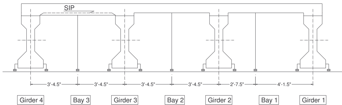
Figure B.4 Displacement transducer positioning
