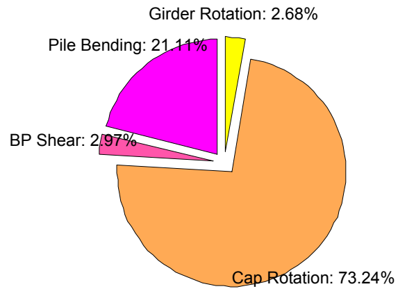
4% ALR Circular / BP V / Load 1 / -1.5in Top Displ.
