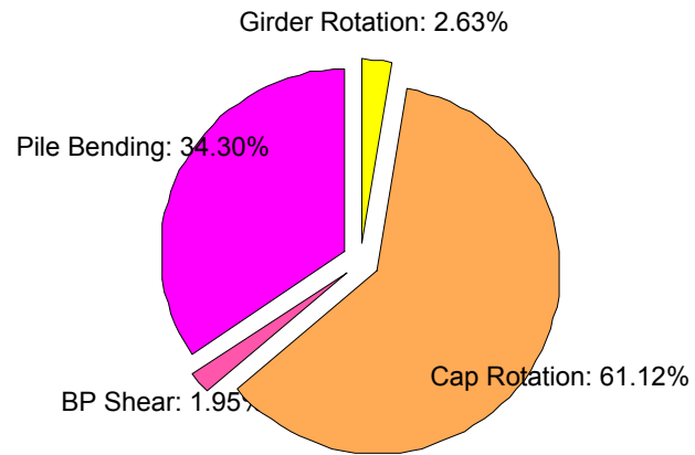
4% ALR Circular / BP V / Load 1 / 1.5in Top Displ.
