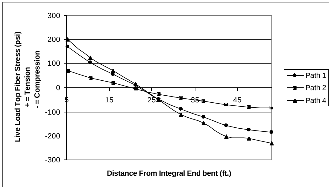
Figure 3-23. Top Fiber Live Load Normal Stress - Deck Girder 1
