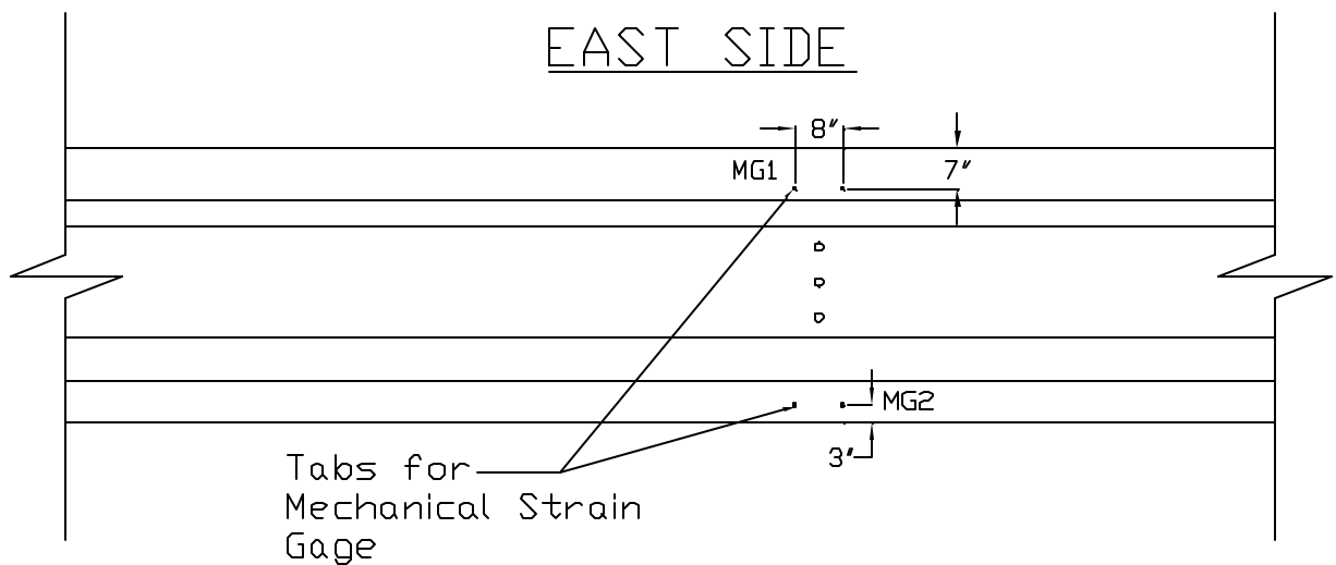
Figure 5-22. Location of Tab Inserts at Mid-Span of the Girder
