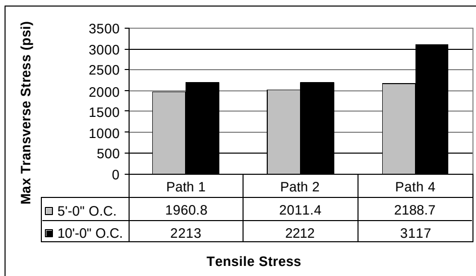
Figure 3-10. ANSYS™ Maximum Tensile Transverse Plate Stress
