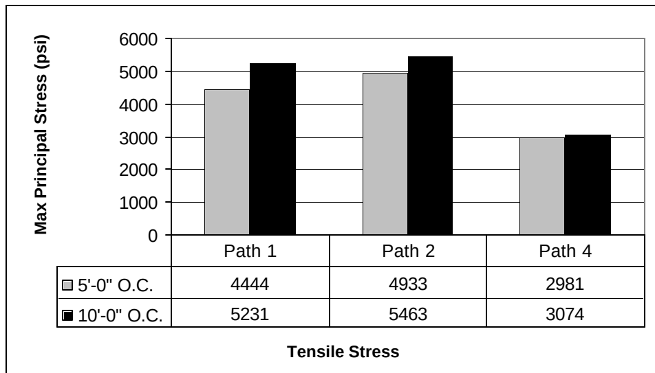
Figure 3-12. ANSYS™ Maximum Tensile Principal Plate Stress
