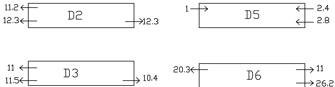
Figure 6-17. Diagram of Axial Forces in Diaphragms (kips) for Path 2 West
