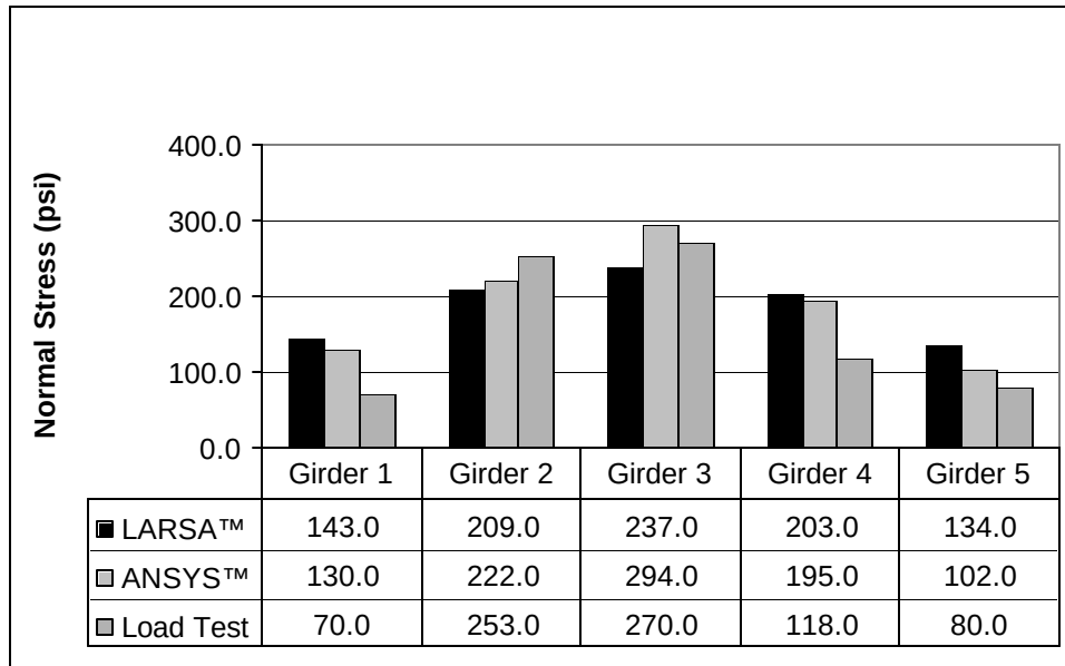
Figure 7-2. Normal Stress at Mid-Span Path 2
