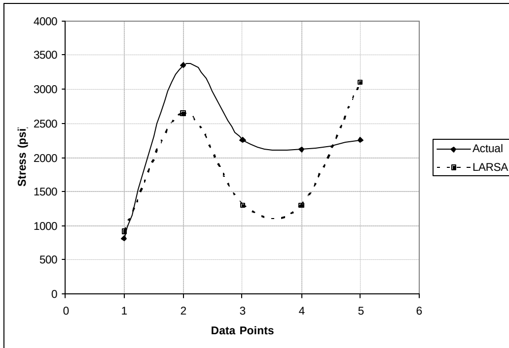
Figure 5-23. Actual vs. Predicted Stress Levels at Selected Points
