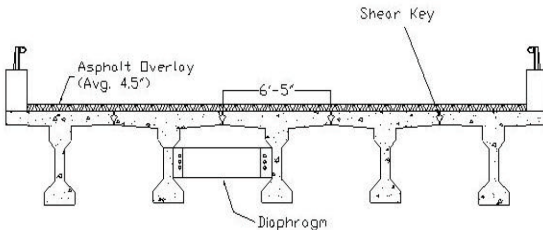
Figure A-2. Section View of Deck Girder Bridge
