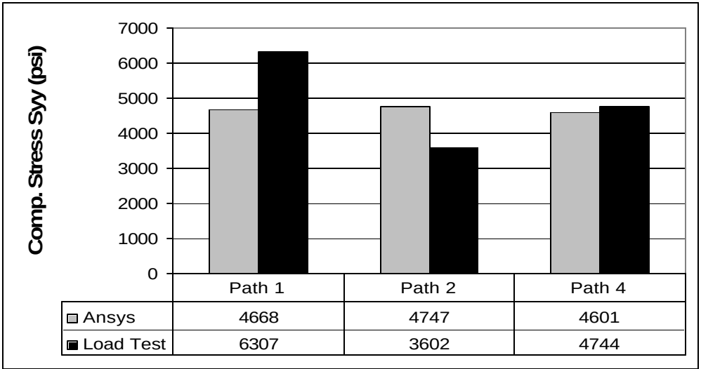
Figure 7-12. Maximum Transverse Compressive Plate Stress
