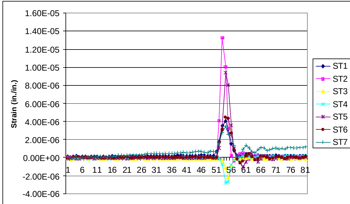
Figure 6-23. Dynamic Loading Strains for Path 1E
