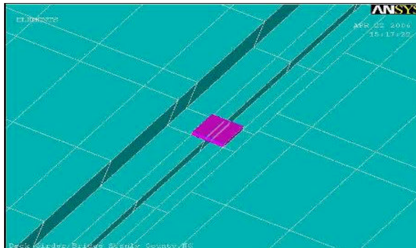
Figure 3-4. Plate Connecting Deck Girder Flanges
