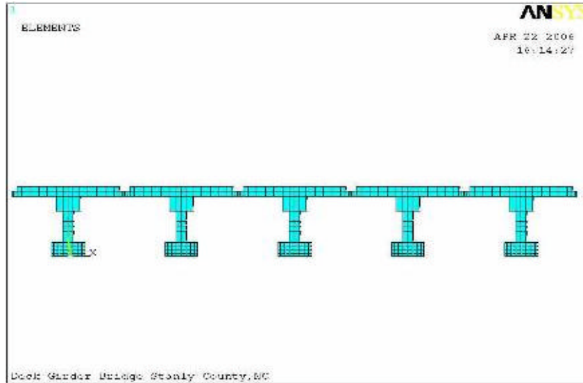
Figure 3-3. Deck Girder Bridge Model
