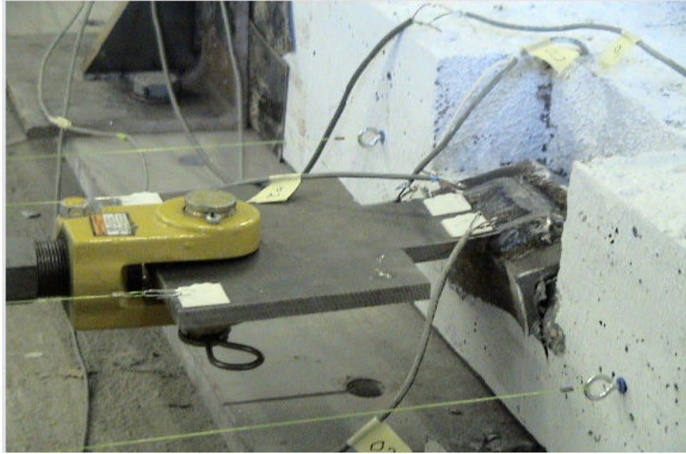
Figure 4-9. Tensile Connection Failure
