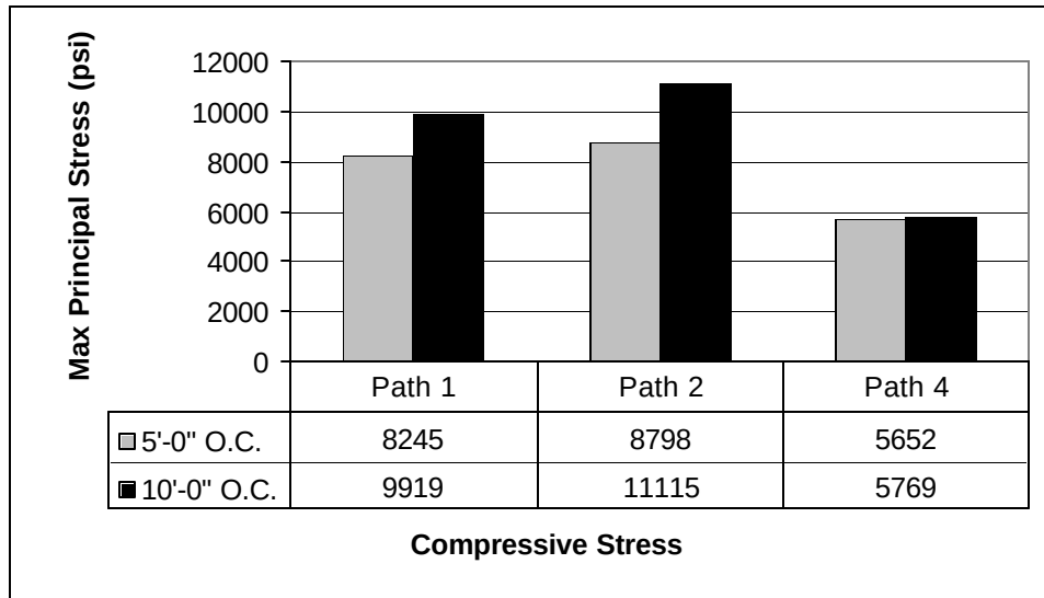
Figure 3-13. ANSYS™ Maximum Compressive Principal Plate Stress
