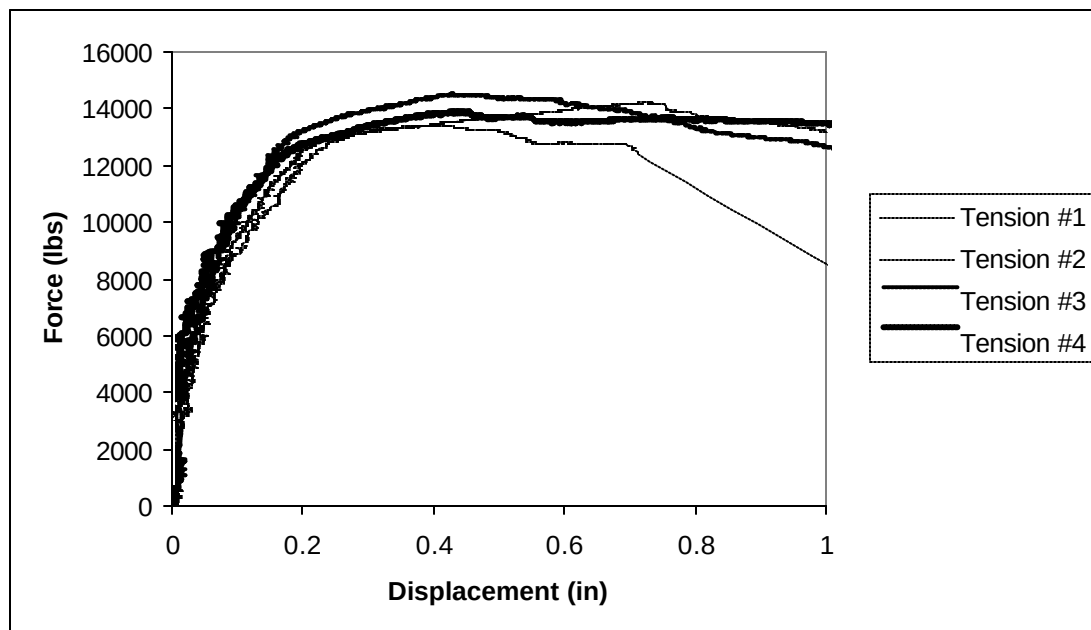
Figure 4-8. Load vs. Displacement for Tension Tests
