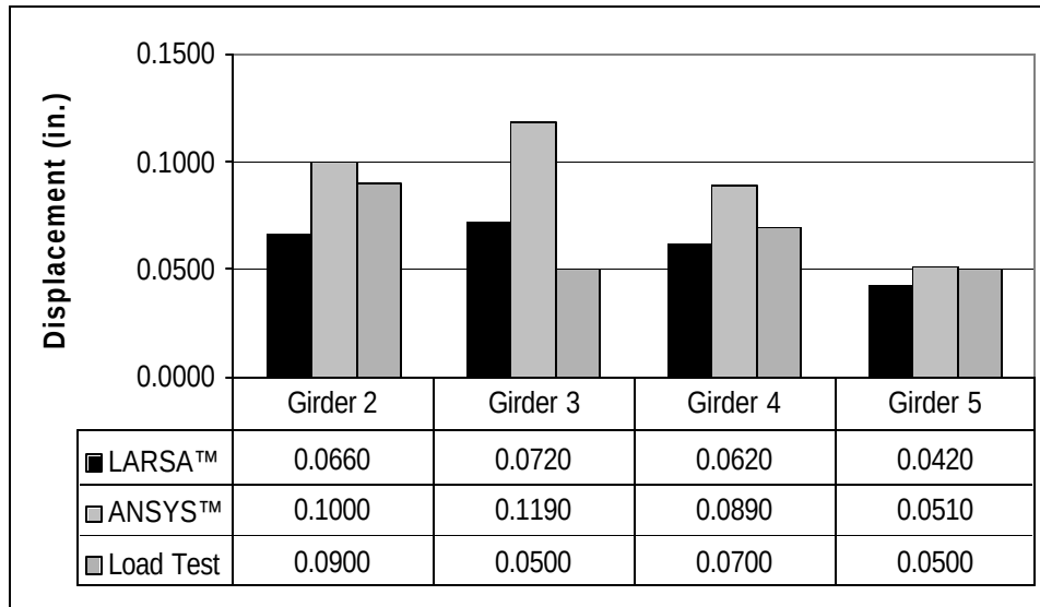
Figure 7-5. Vertical Displacement at Mid-Span Path 2
