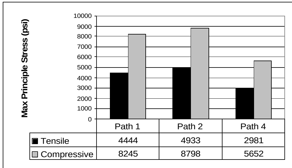
Figure 7-13. Maximum Principal Plate Stress
