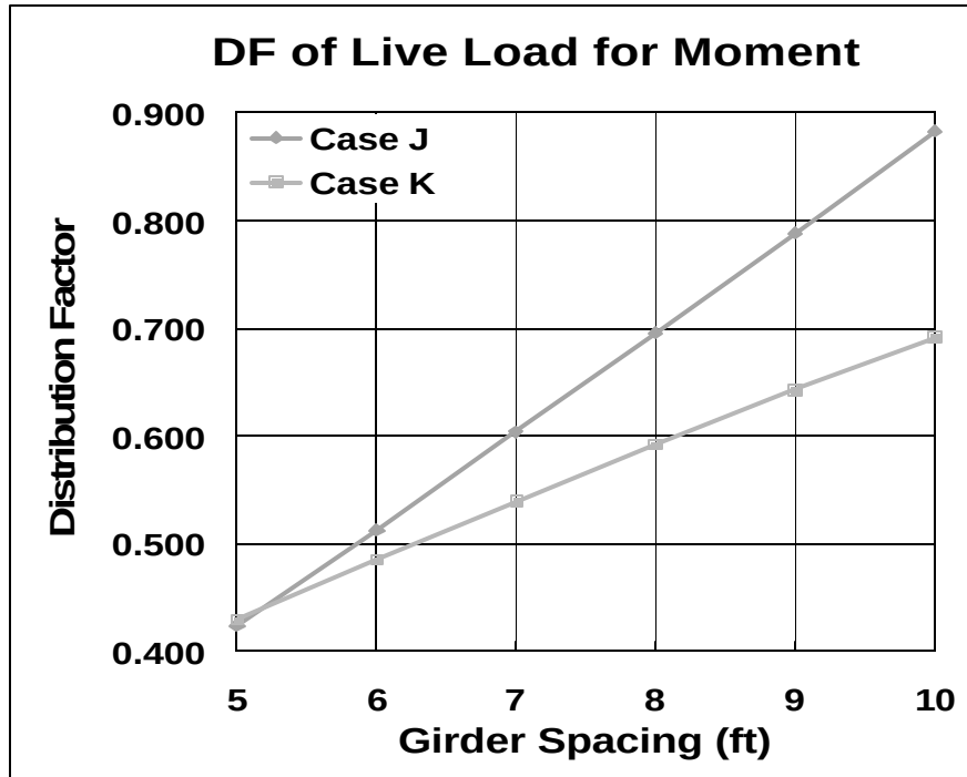
Figure 2-1. Category k and j Moment Distribution Factor Comparison
