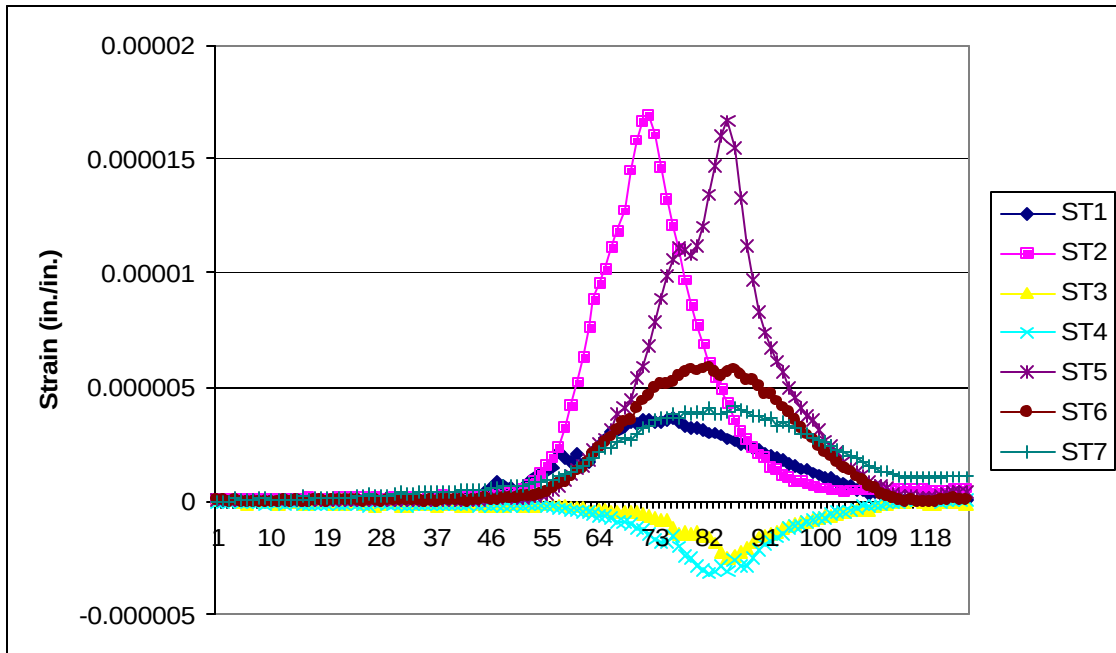
Figure 6-20. One Truck (Slow) Loading Strains for Path 1E
