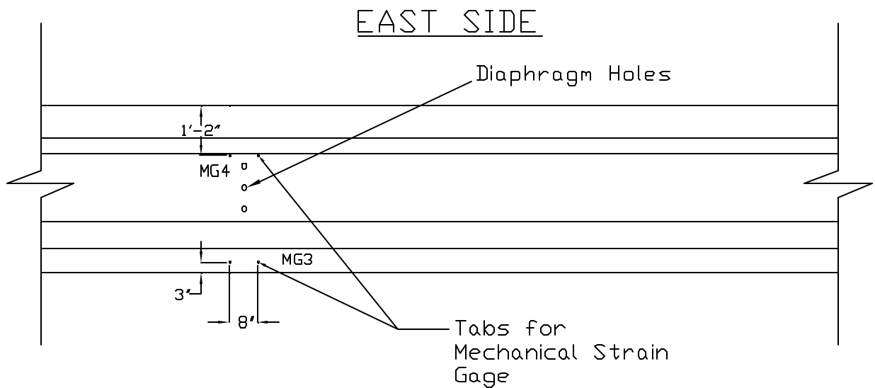
Figure 5-21. Location of Tab Inserts at Quarter Point on the Girder
