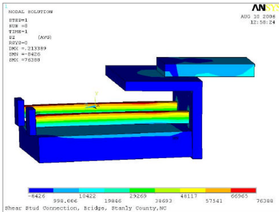
Figure 4-3. Deformed Flange Connection with Pivot Surface
