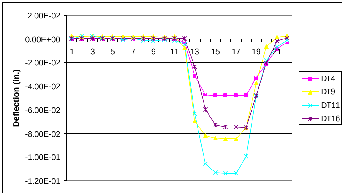
Figure 6-19. Deflections in Deck Girder 2 from Load Path 1 East
