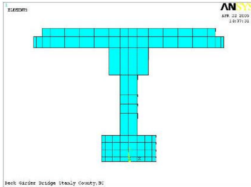
Figure 3-1. Equivalent Deck Girder Cross Section
