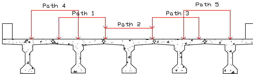
Figure 3-9. Bridge Load Test Truck Paths
