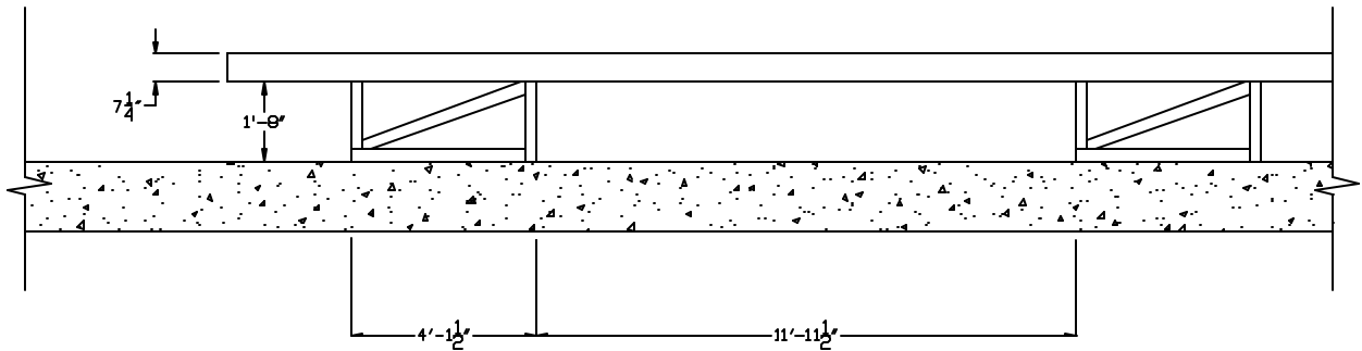
Figure 5-17. Section of Deck Formwork
