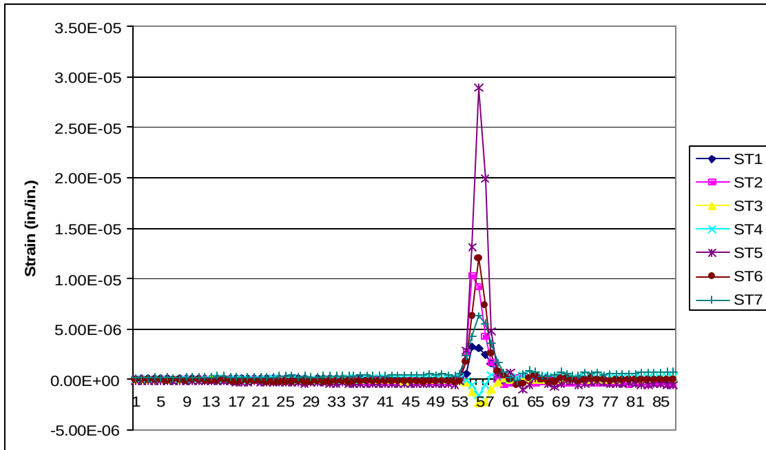
Figure 6-24. Dynamic Loading Strains for Path 2E
