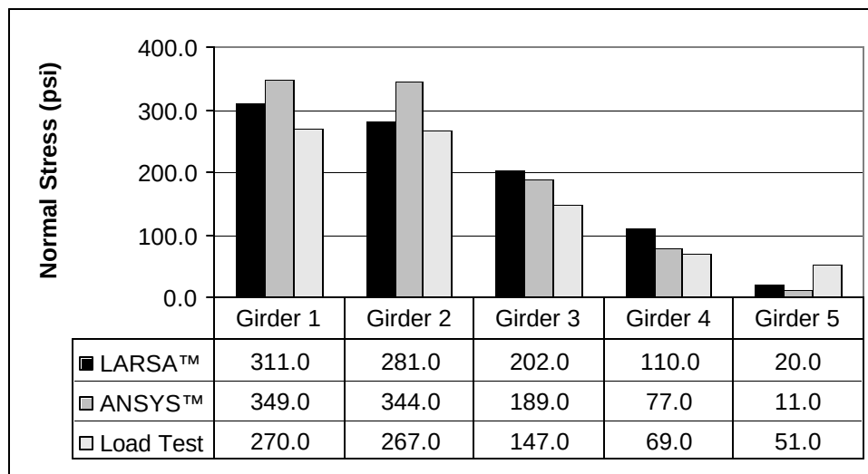
Figure 7-1. Normal Stress at Mid-Span Path 1
