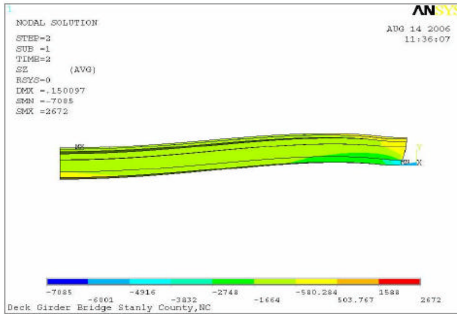
Figure 3-24. Deformed Shape and Un-adjusted Normal Stress- Deck Girder 1
