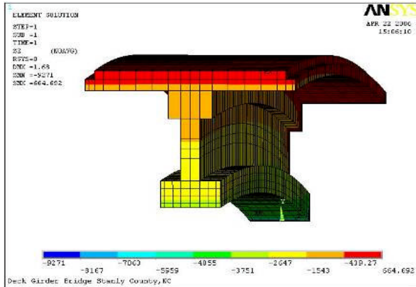
Figure 3-2. Prestress + Self-Weight Normal Stress
