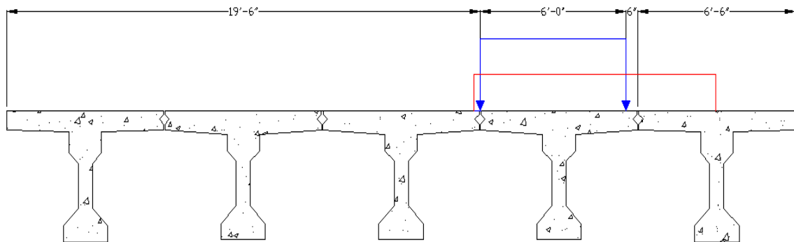
Figure 2-9. Truck 2 and Lane Load Layout
