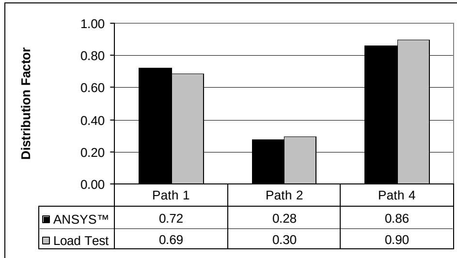
Figure 7-8. 2 –Wheel Lines Distribution Factor for Exterior Deck Girder Paths
