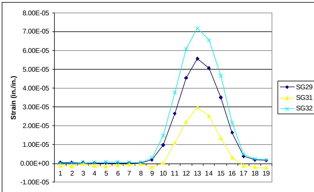
Figure 6-15. Strains in D6 for Path 2 West
