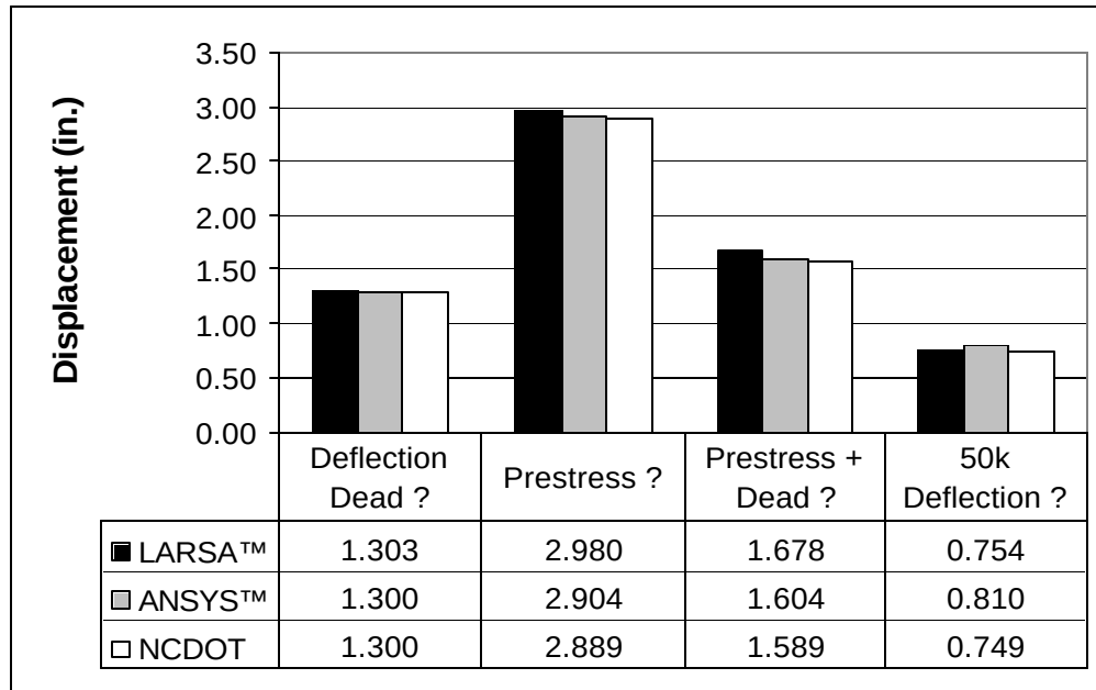
Figure 3-7. Equivalent Deck Girder Displacement Comparison.
