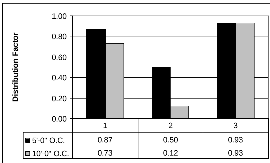
Figure 3-22. 4 –Wheel Lines Distribution Factor for Exterior Girder Paths
