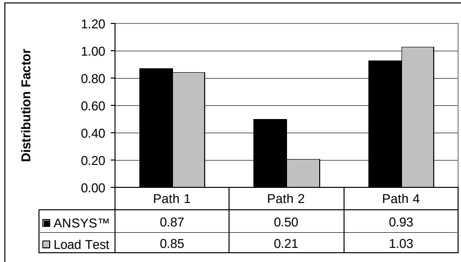
Figure 7-10. 4 –Wheel Lines Distribution Factor for Exterior Deck Girder Paths
