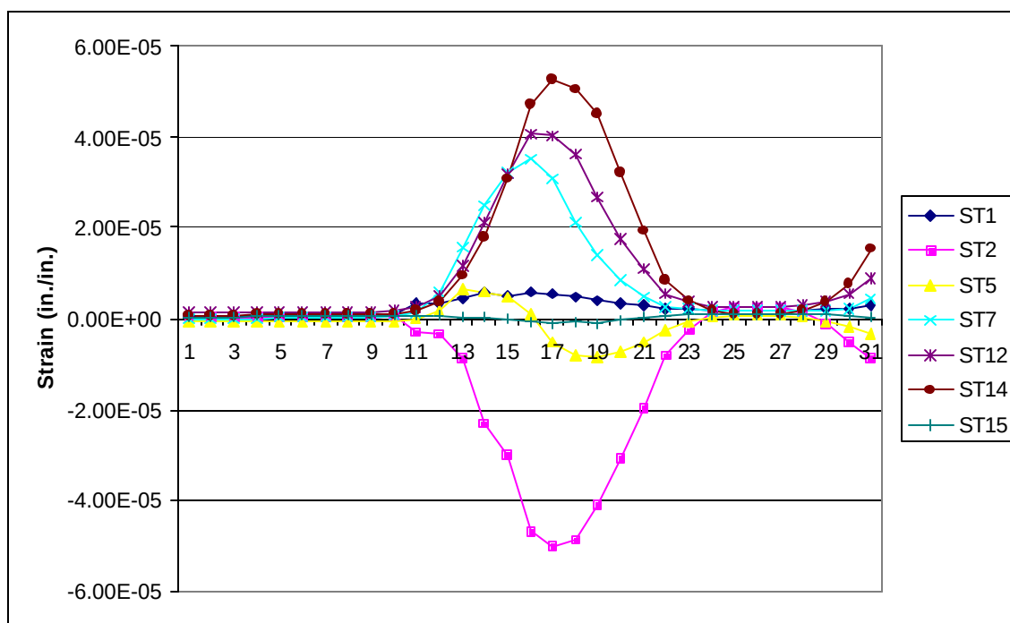
Figure 6-9. Deck Girder 1 Strain Values from Path 4E
