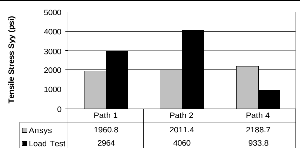
Figure 7-11. Maximum Transverse Tensile Plate Stress
