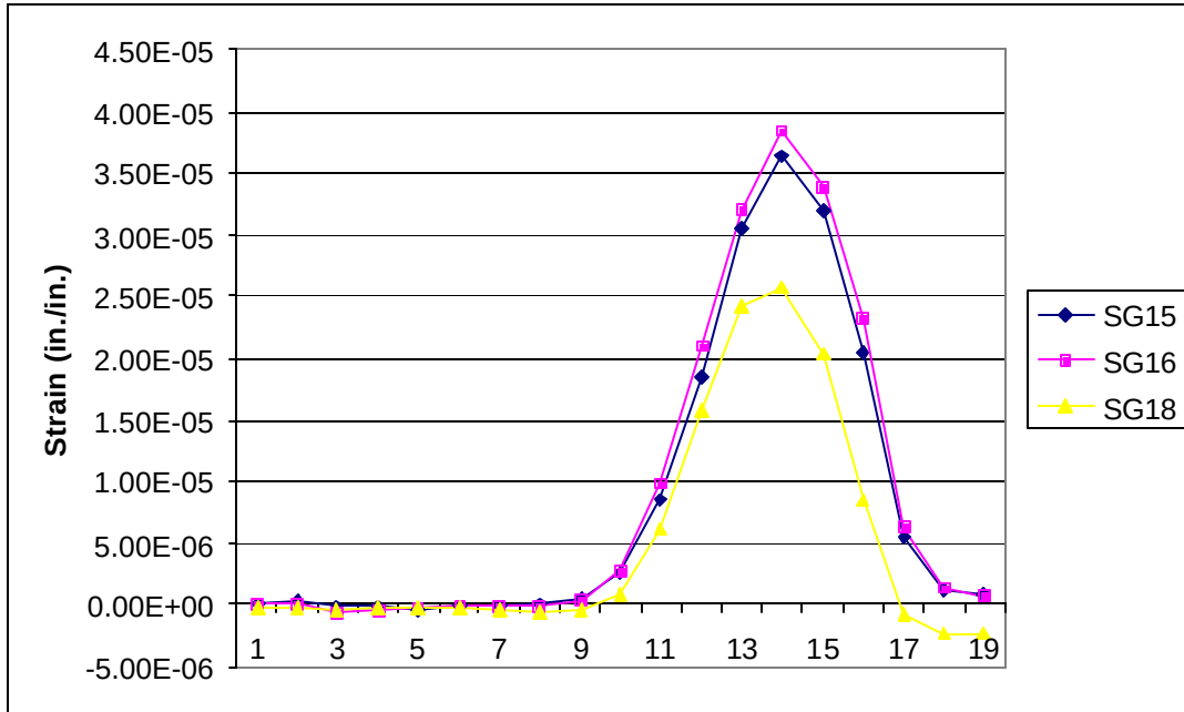
Figure 6-14. Strains in D3 for Path 3 West
