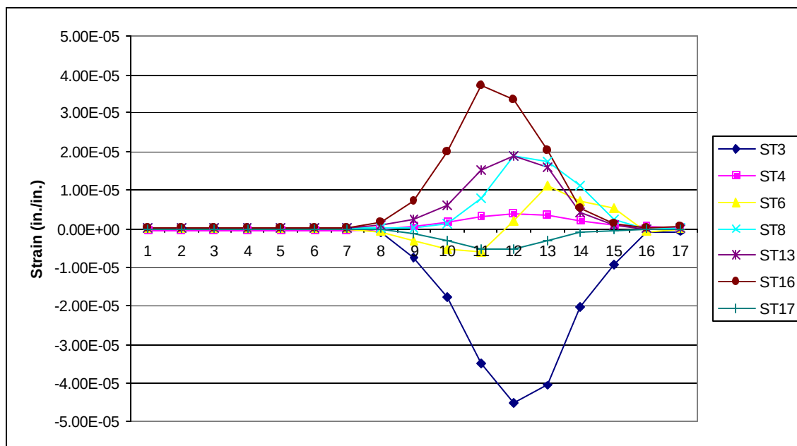
Figure 6-9. Deck Girder 1 Strain Values from Path 4E
