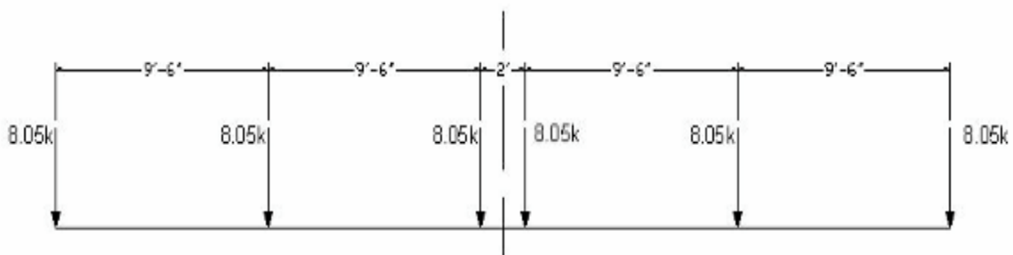
Figure 3-8. Equivalent Truck Live Loading
