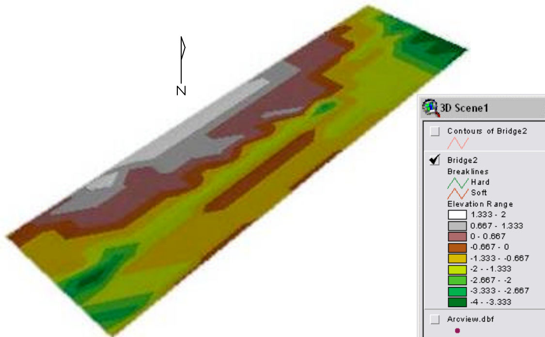
Figure 5-29. Arcview GIS 3.3® Image of Riding Surface Without Wearing Surface
