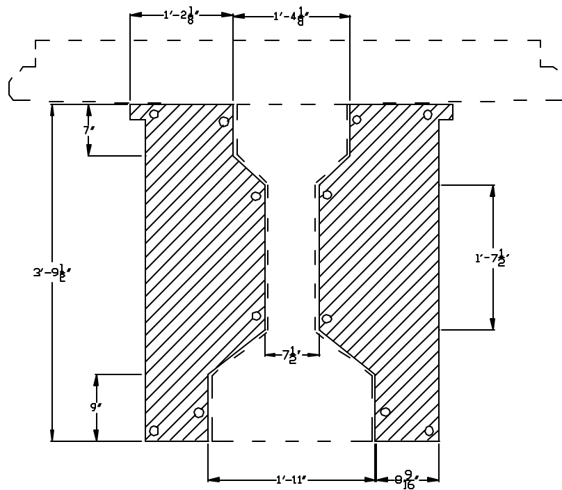
Figure 5-16. AASHTO Girder Formwork
