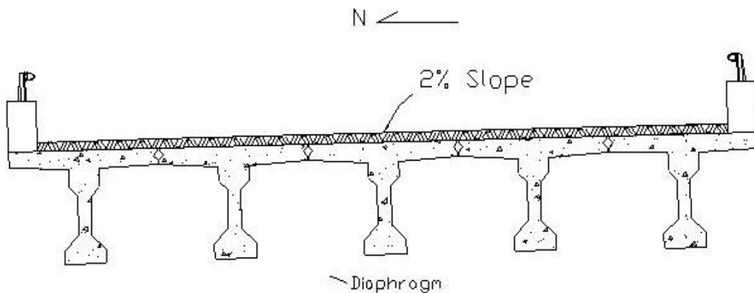
Figure A-3. Transverse Slope of New Deck Girder Bridge
