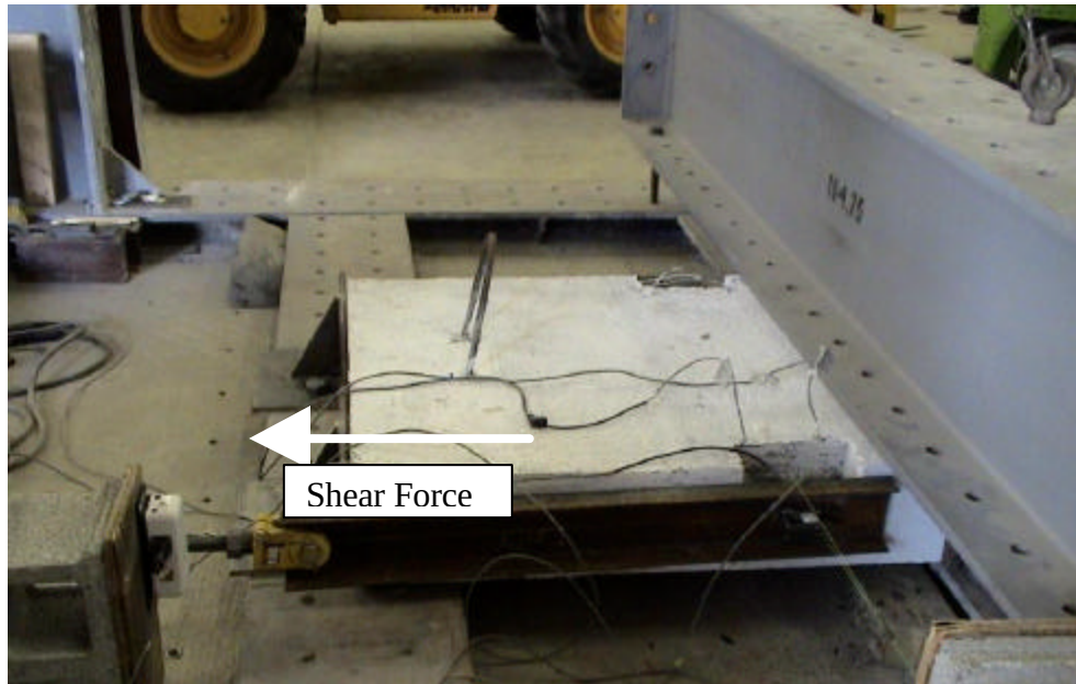
Figure 4-10. Shear Connection Test
