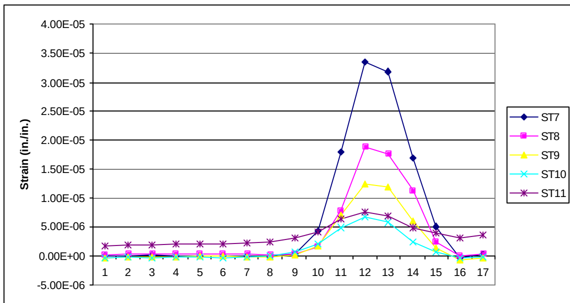
Figure 6-12. Strain Readings at the Quarter-Points on Path 4 West
