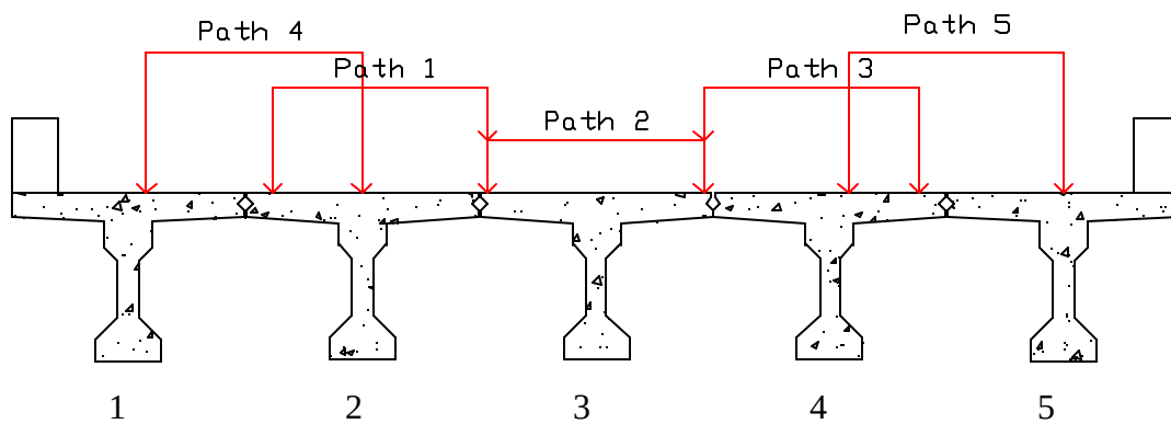
Figure 6-6. Loading Paths for Testing
