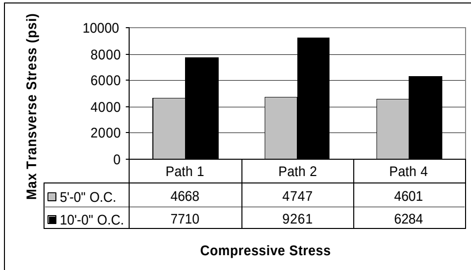
Figure 3-11. ANSYS™ Maximum Compressive Transverse Plate Stress
