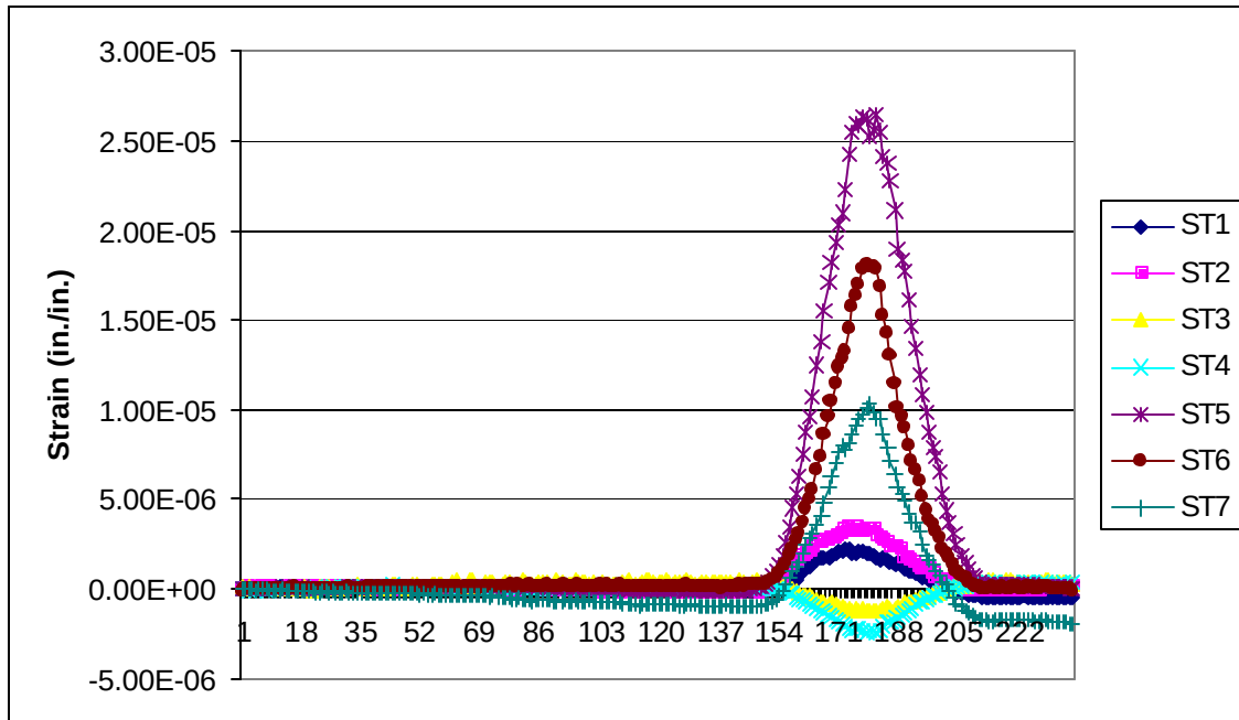
Figure 6-22. One Truck (Slow) Loading Strains for Path 3E
