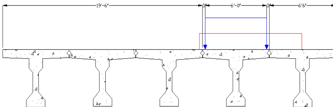
Figure 2-11. Truck 4 and Lane Load Layout
