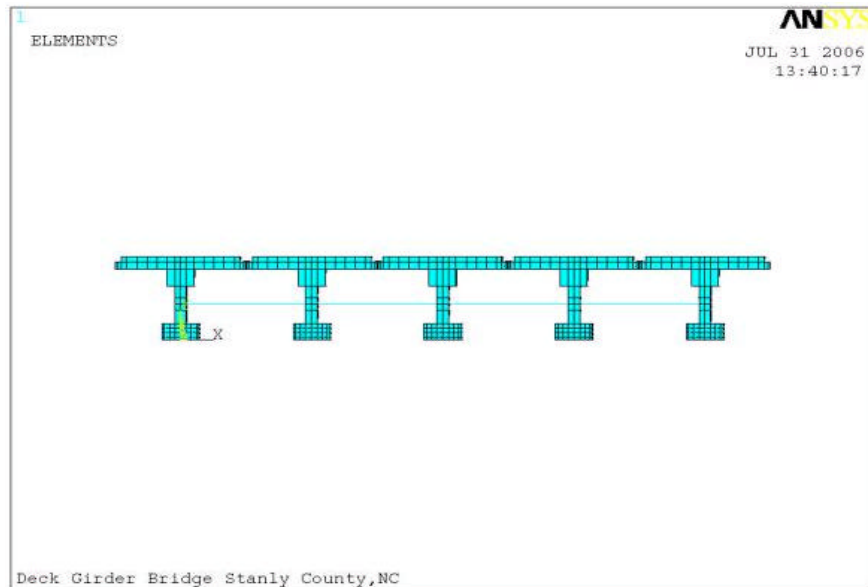
Figure 3-5. Diaphragms on Half-Bridge Model
