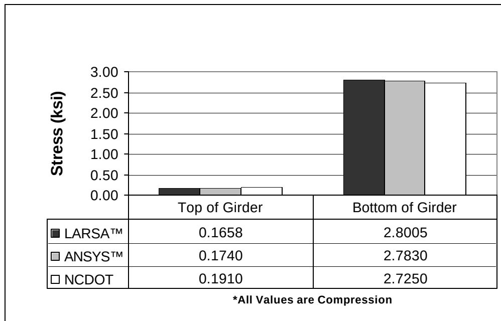
Figure 3-6. Equivalent Deck Girder Stress at Extreme Fiber Comparison
