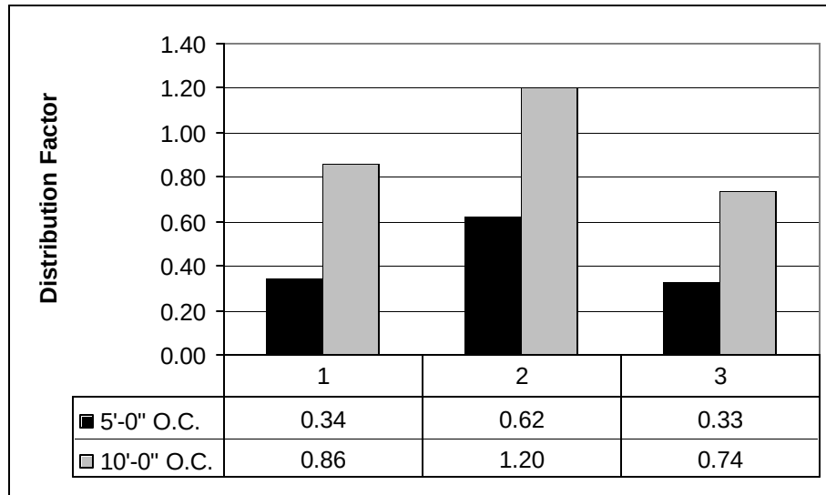
Figure 3-21. 4 –Wheel Lines Distribution Factor for Interior Girder Paths
