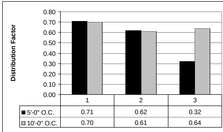
Figure 3-19. 2 –Wheel Lines Distribution Factor for Interior Girder Paths
