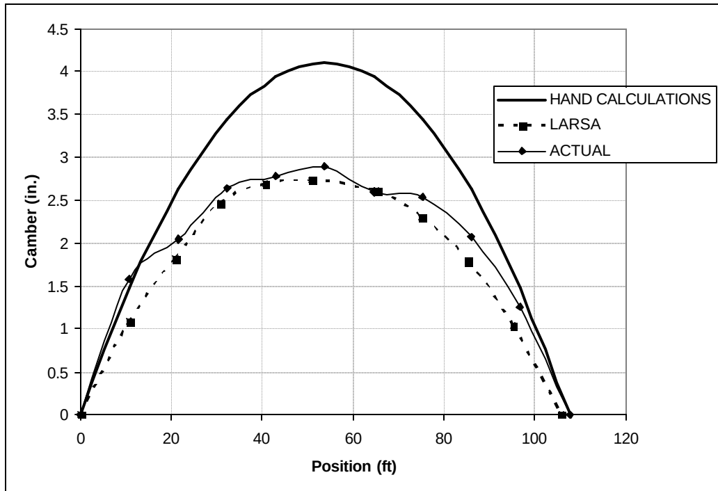
Figure 5-20. Predicted vs. Actual Camber Measurements
