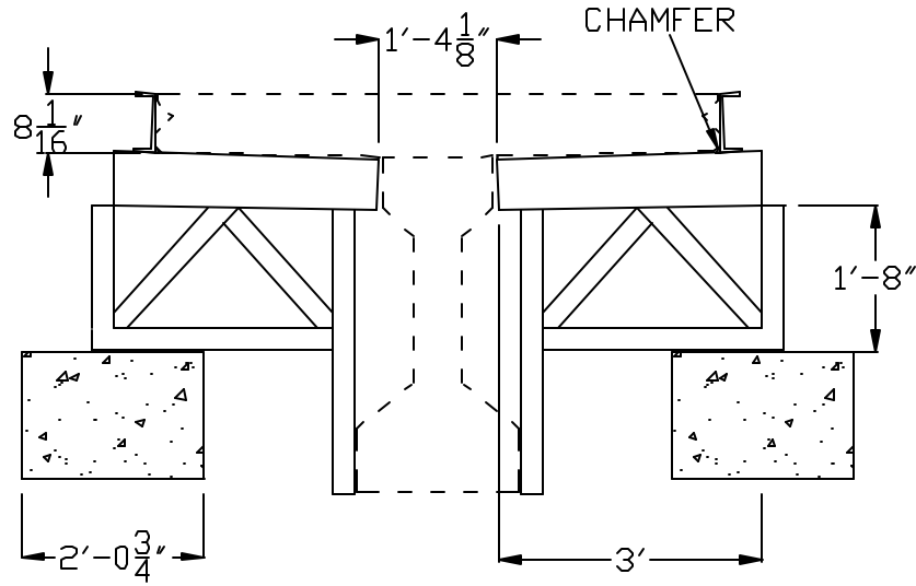
Figure 5-17. Section of Deck Formwork
