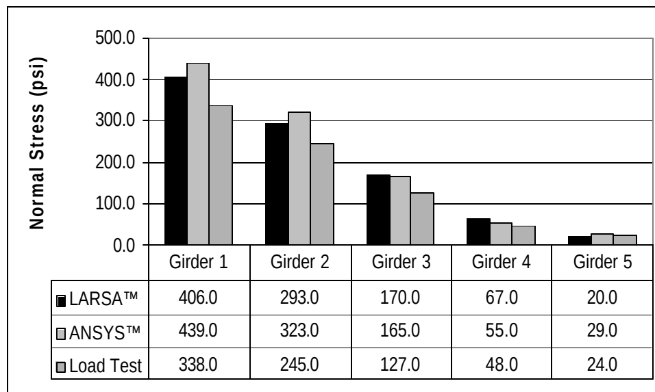
Figure 7-3. Normal Stress at Mid-Span Path 4
