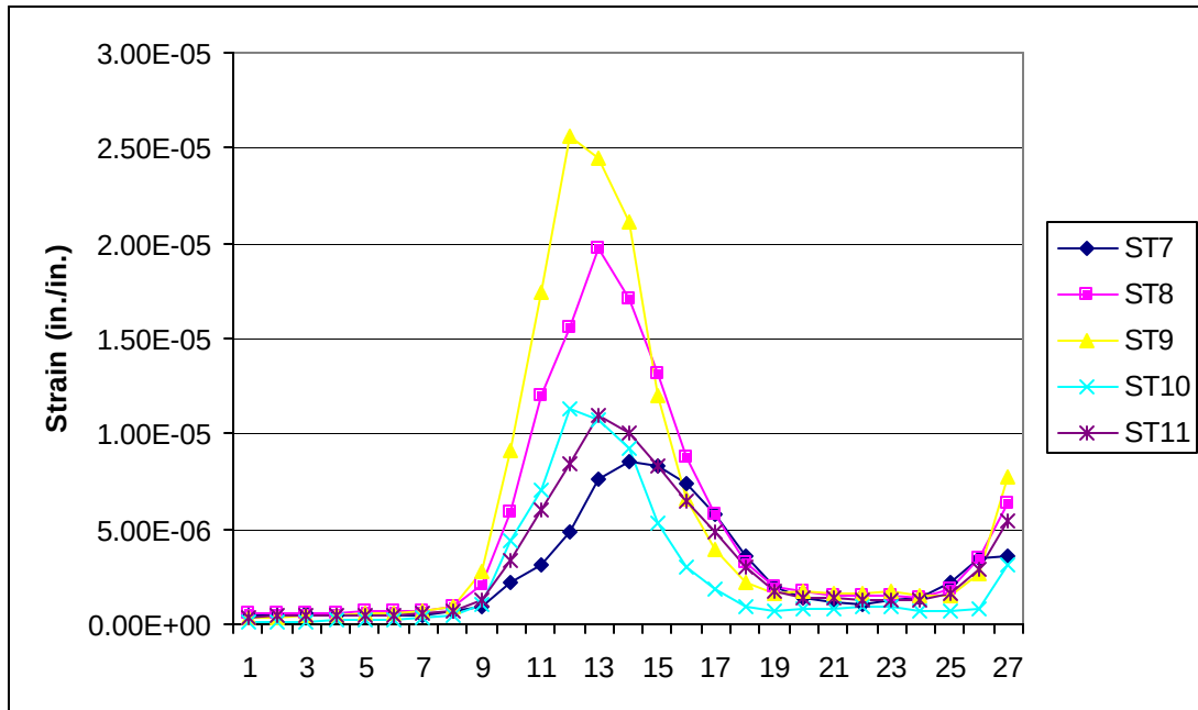
Figure 6-11. Strain Readings at the Quarter-Points on Path 2 West
