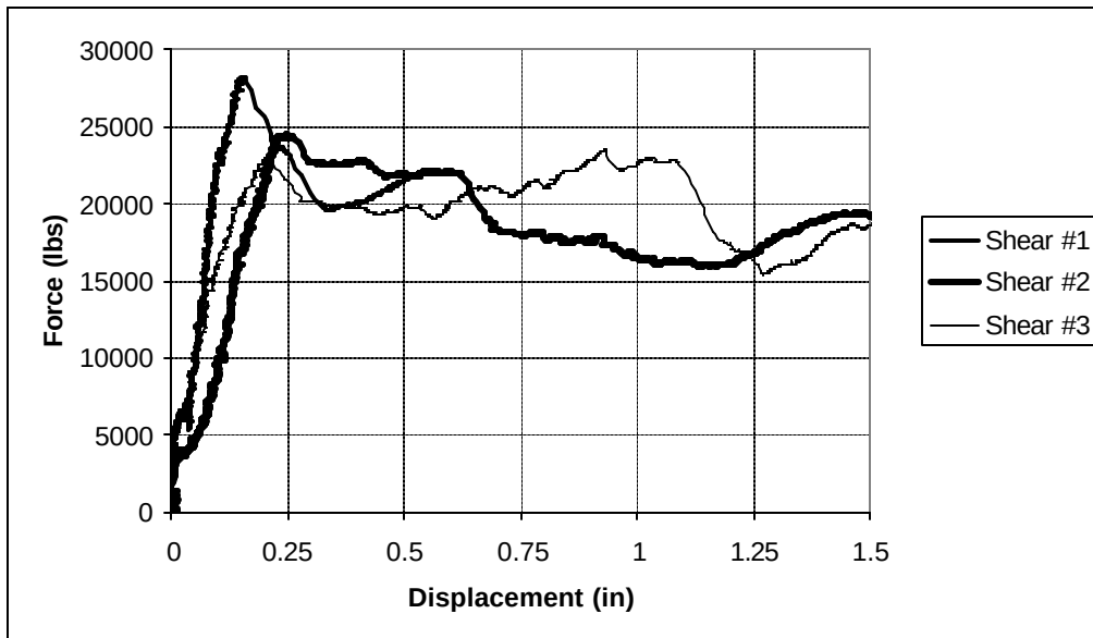
Figure 4-11. Load vs. Displacement for Shear Tests
