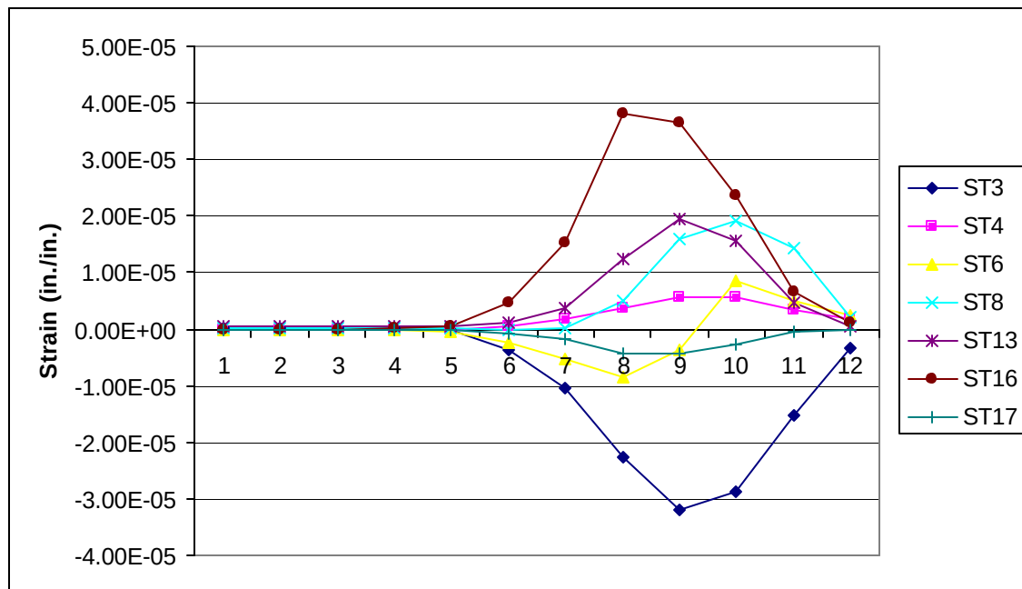
Figure 6-8. Deck Girder 1 Strain Values from Path 1W
