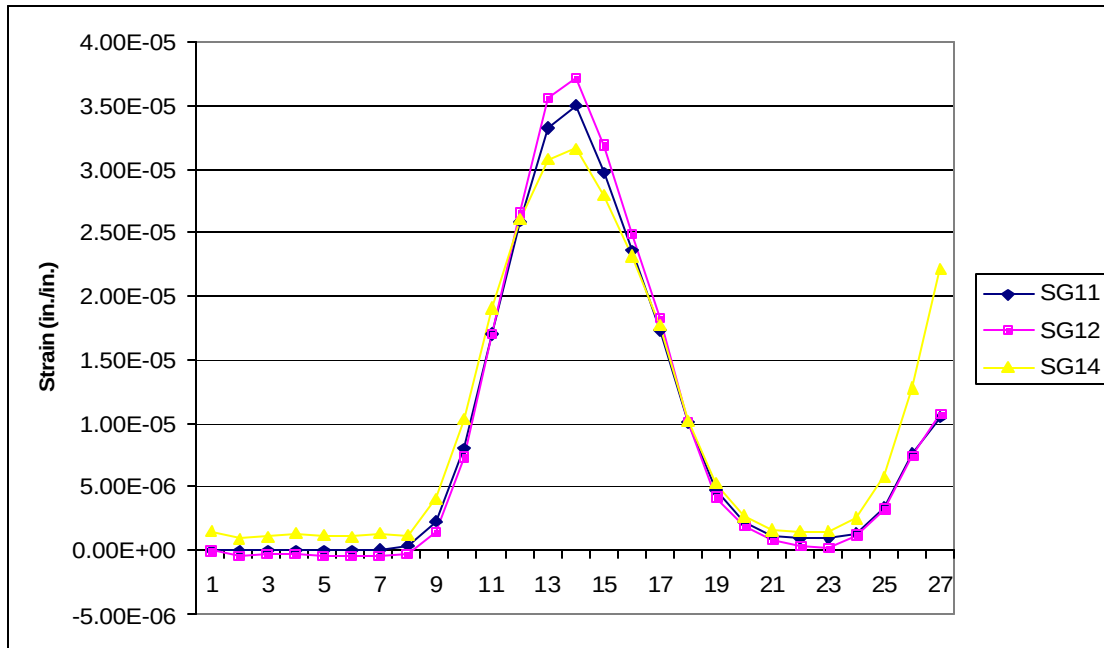
Figure 6-13. Strains in D2 for Path 2 East
