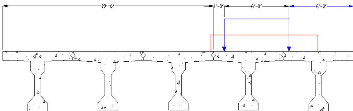
Figure 2-10. Truck 3 and Lane Load Layout
