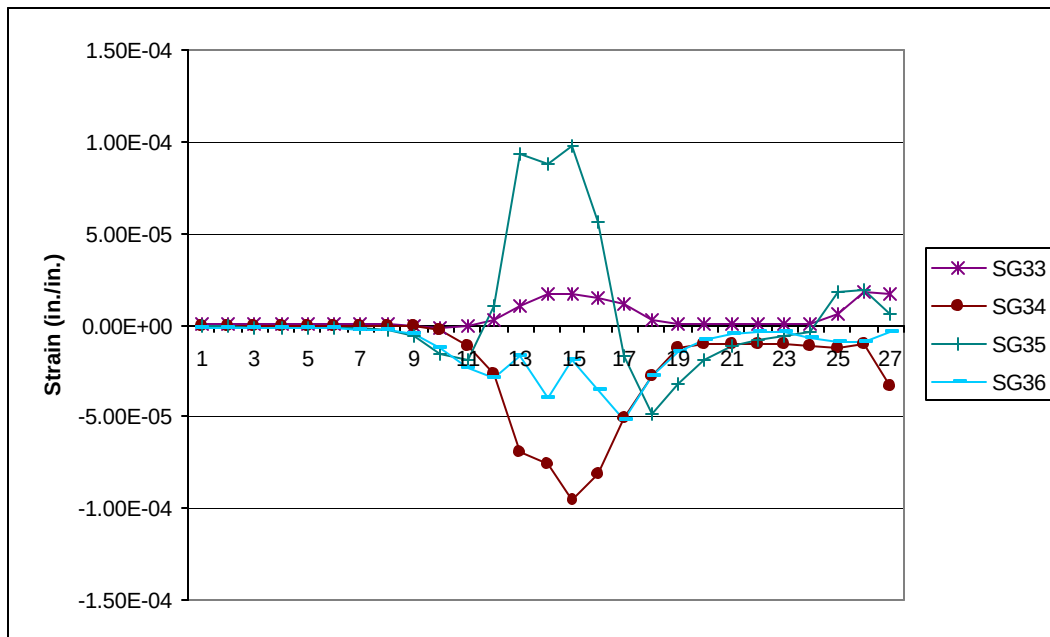
Figure 6-18. Plate Strains From Path 2 East
