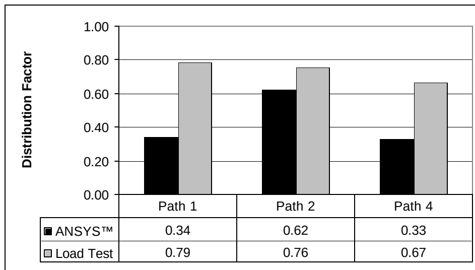
Figure 7-9. 4 –Wheel Lines Distribution Factor for Interior Deck Girder Paths
