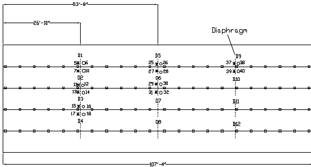
Figure C-3. Plate Connection Strain Gage Layout
