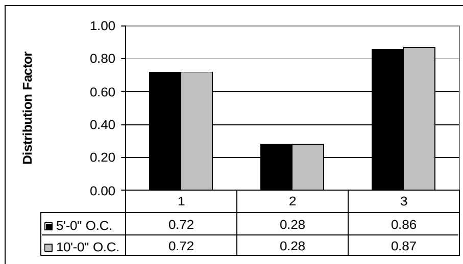
Figure 3-20. 2 –Wheel Lines Distribution Factor for Exterior Girder Paths
