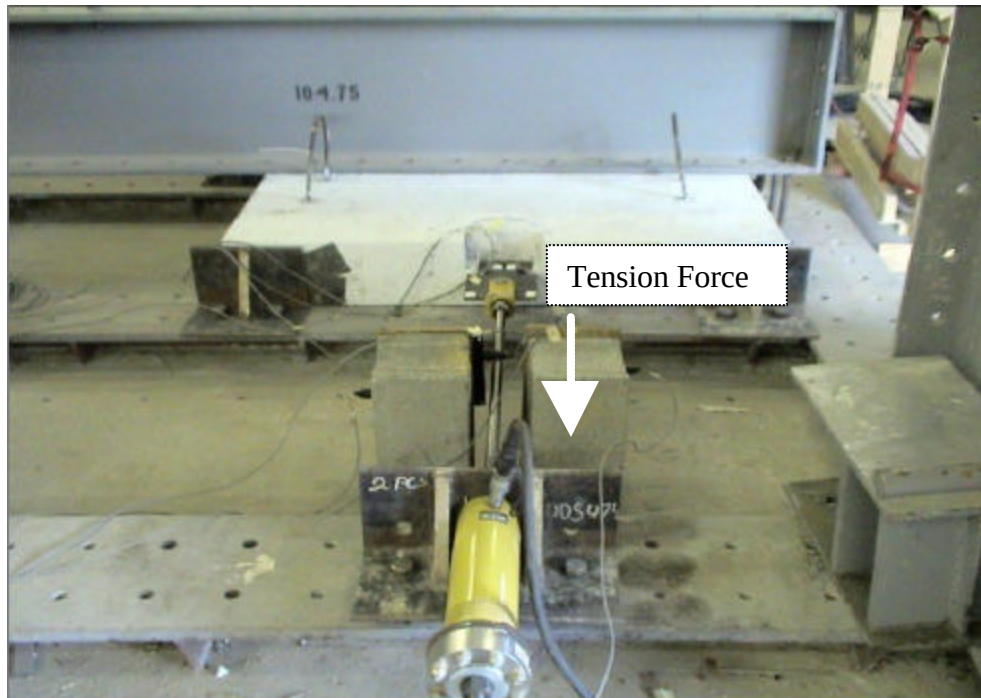
Figure 4-7. Tension Connection Test
