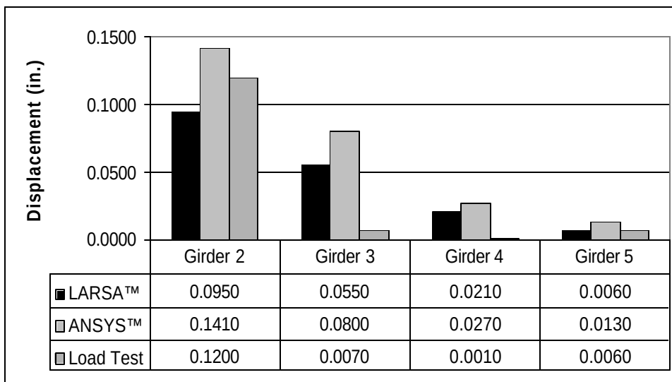
Figure 7-6. Vertical Displacement at Mid-Span Path 4
