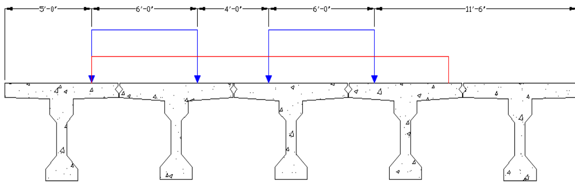
Figure 2-8. Truck 1 and Lane Load Layout
