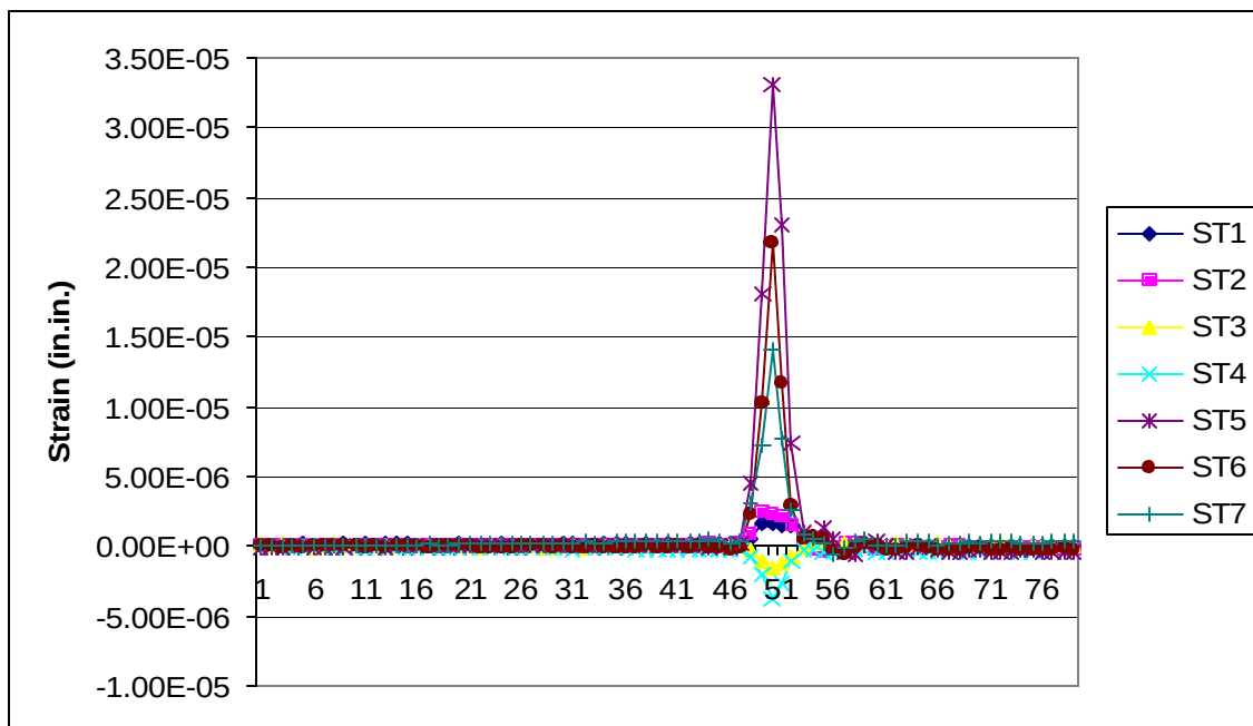
Figure 6-25. Dynamic Loading Strains for Path 3E
