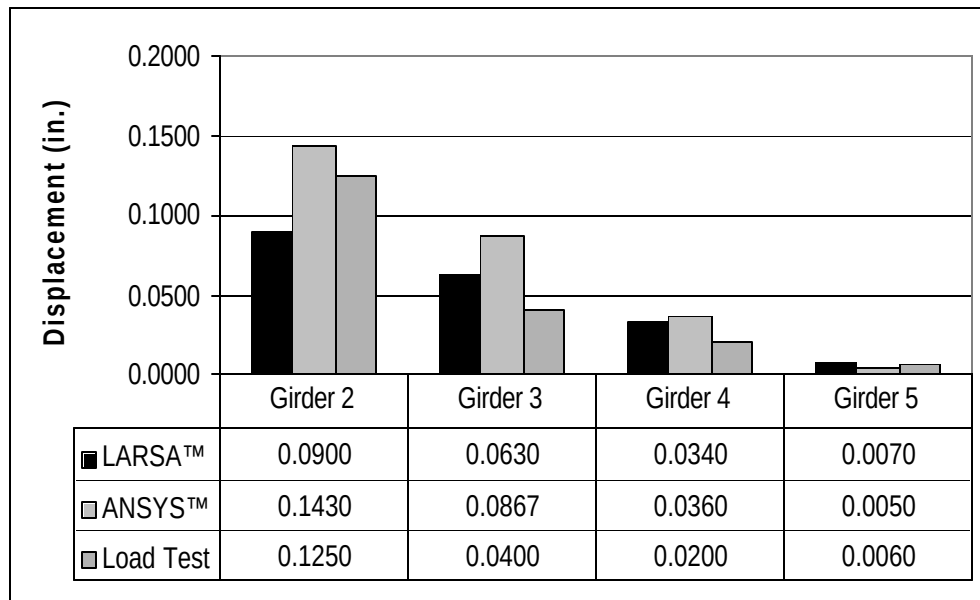
Figure 7-4. Vertical Displacement at Mid-Span Path 1
