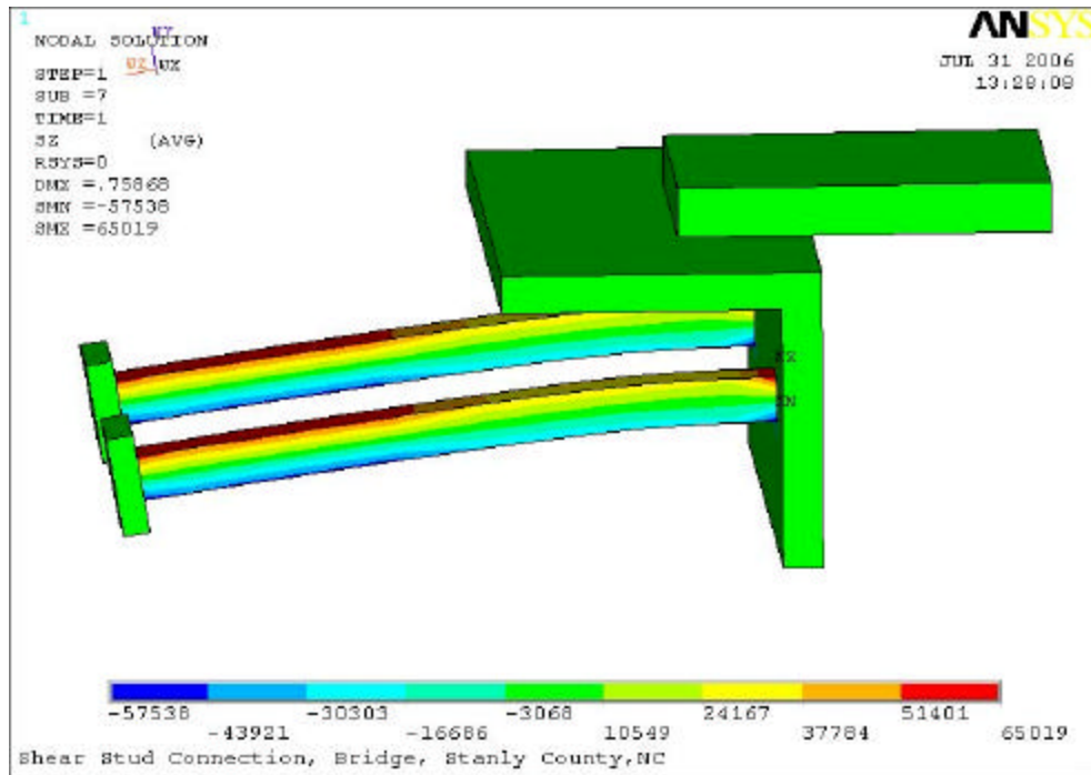
Figure 4-2. Flange Connection Deformed Shape
