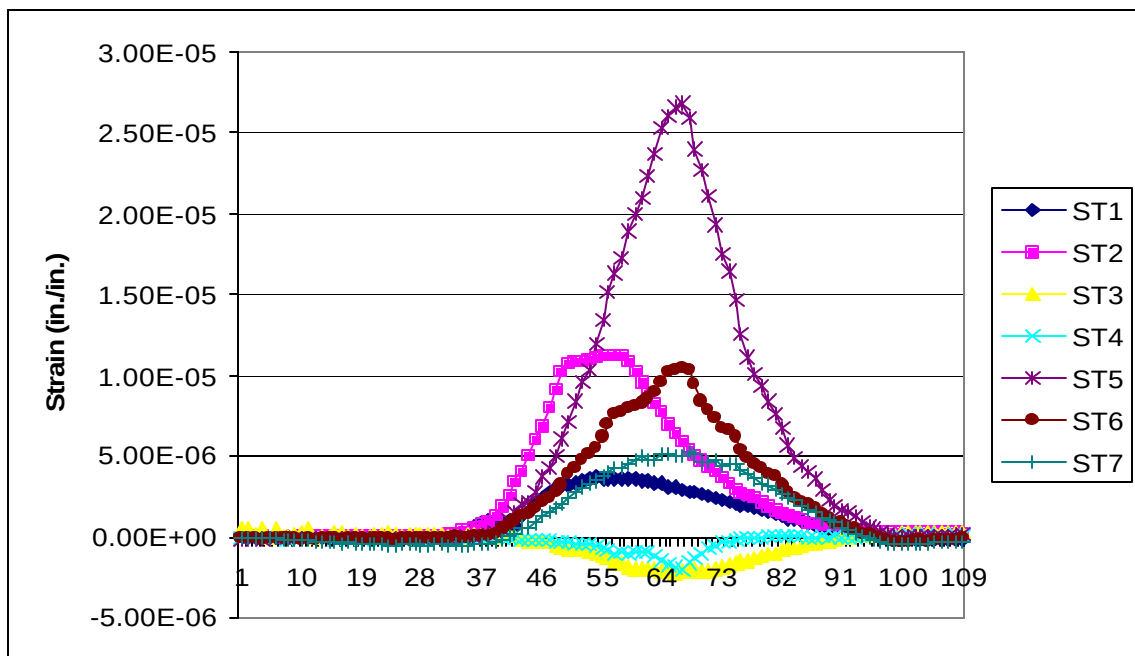
Figure 6-21. One Truck (Slow) Loading Strains for Path 2E
