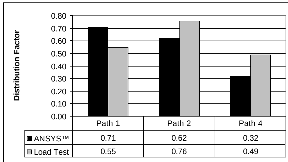
Figure 7-7. 2 –Wheel Lines Distribution Factor for Interior Deck Girder Paths
