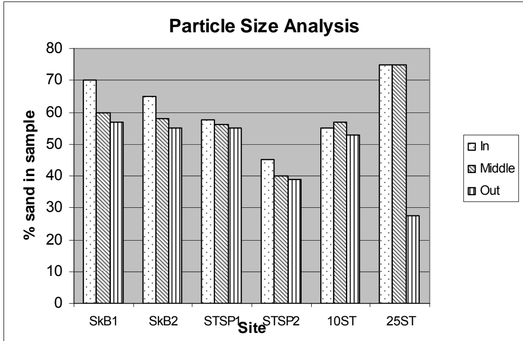
Figure 19. Sand content for soil samples taken within the devices at the end of the monitoring period..
