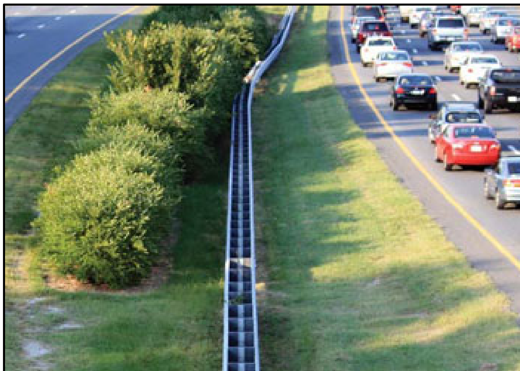
Exhibit 32: Grass Median with Guardrail.
