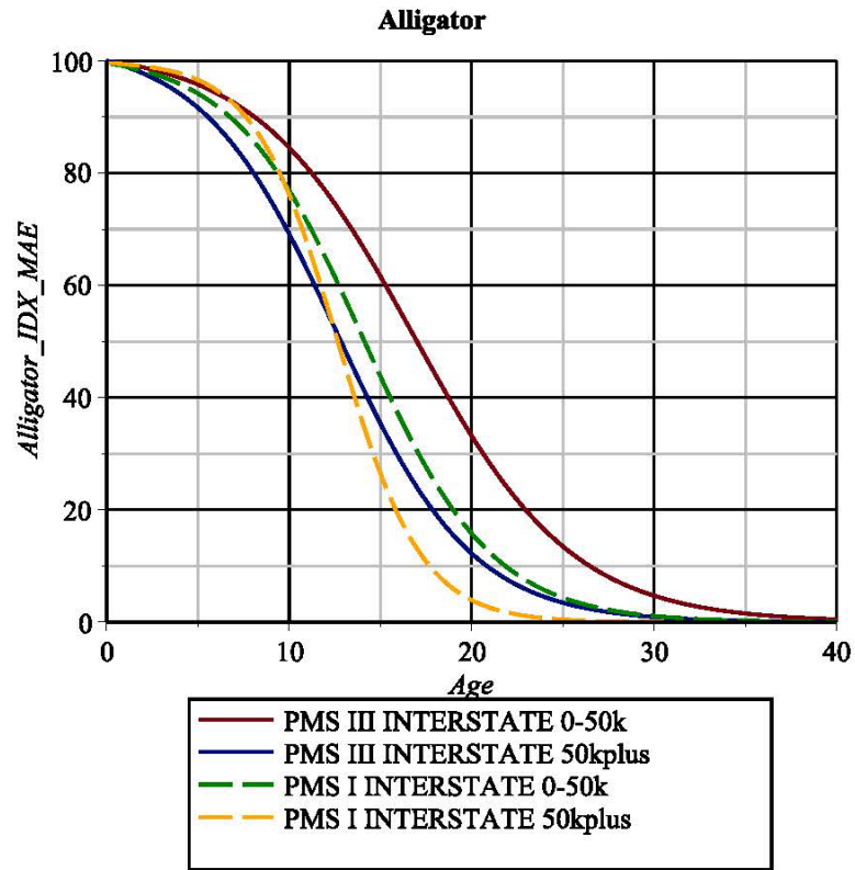
Figure 1: Alligator Cracking Comparison Curves (PMS I Interstate 0-50, PMS I Interstate 50kplus, PMS III Interstate 0-50k, PMS III Interstate 50kplus)
