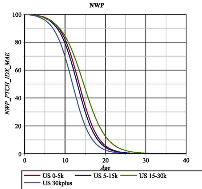
Figure 14: NWP Curves (US 0-5k, US 5-15k, US 15-30k, US 30kplus)
