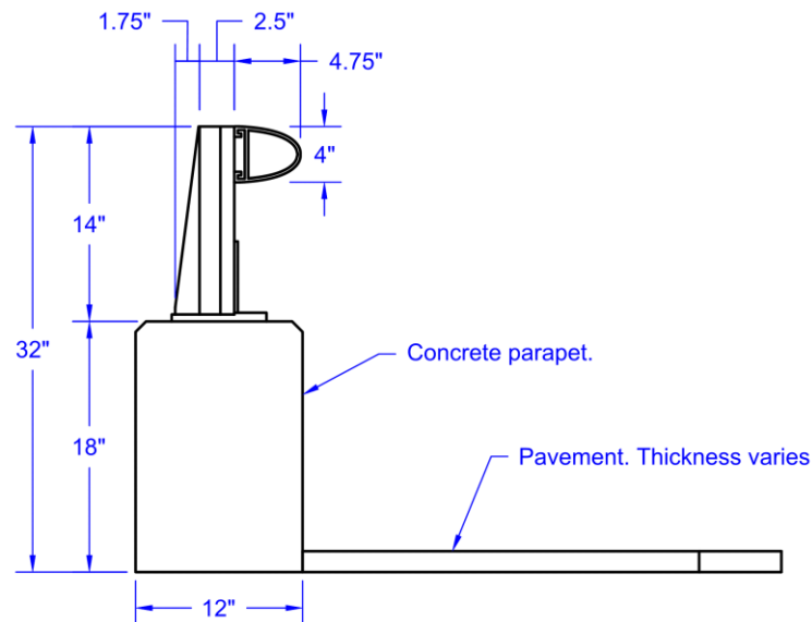
Figure 5 – Guardrail Type 01 section
