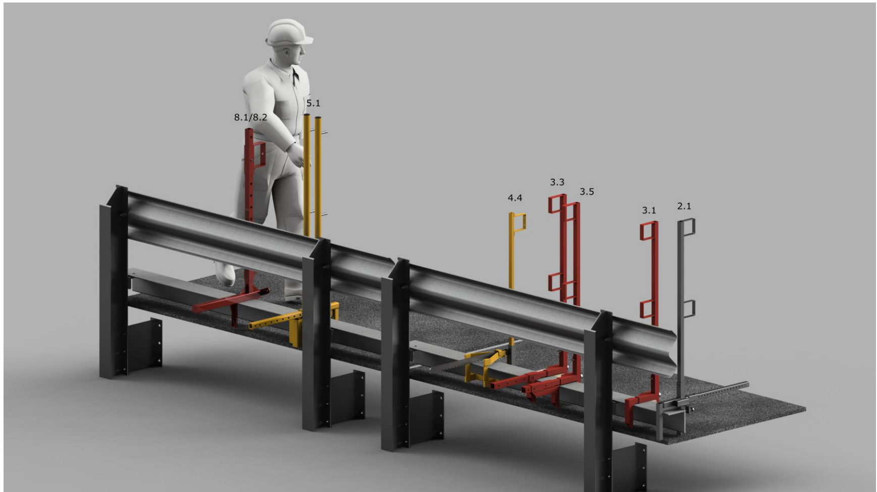
Figure 83 - Guardrail Type 23, wheel guard fit; view from the southwest
