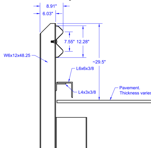
Figure 70 - Guardrail Type 23 section
