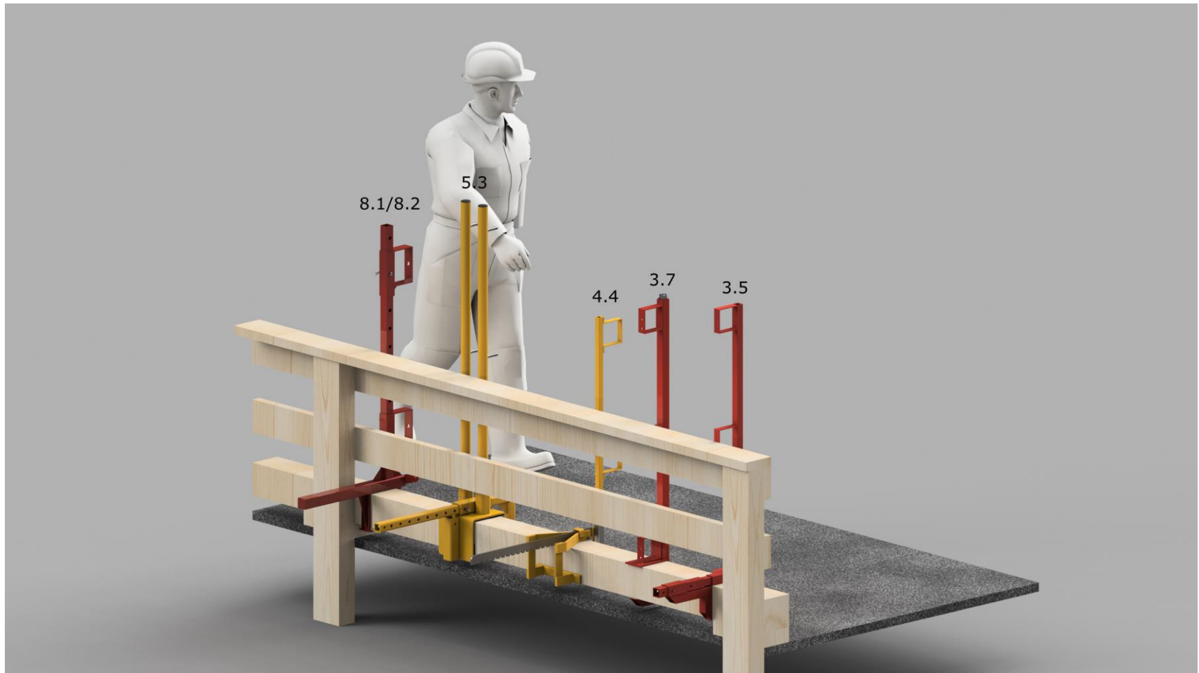
Figure 66 – Guardrail Type 22, wheel guard fit; view from the southwest
