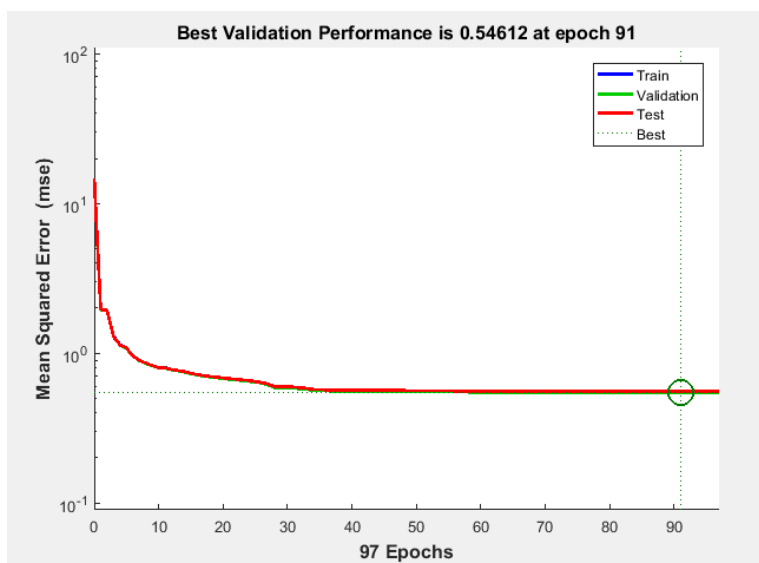
Figure 11 Performance of the Neural Network Model
