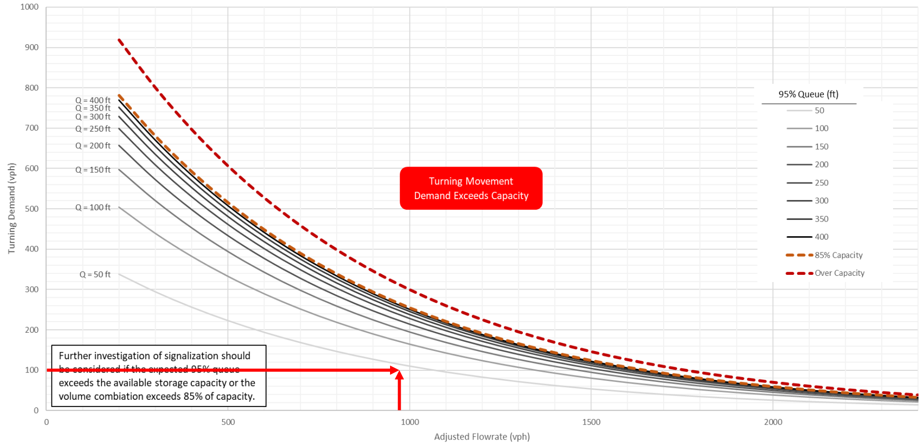
Right Turn - 95% Queue Length
